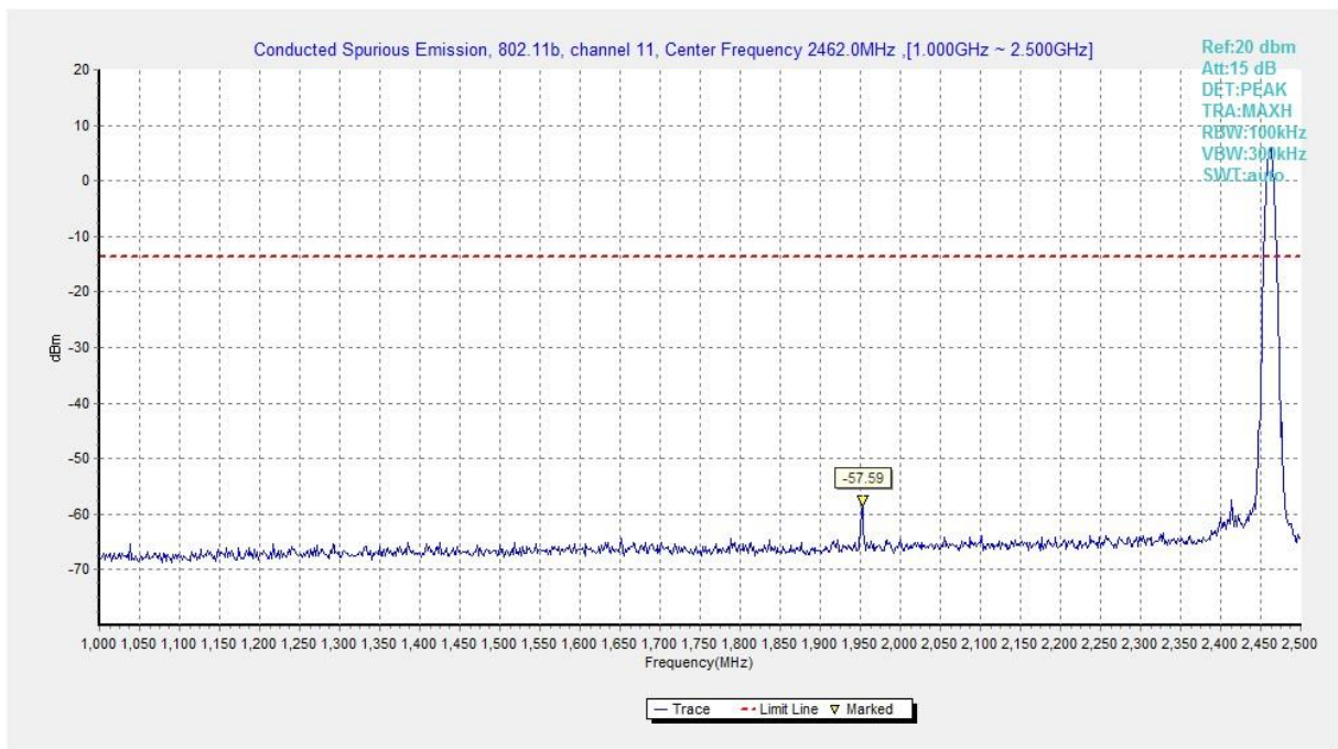
Fig.A.6.1.163 Transmitter Spurious Emission - Conducted (802.11b, Ch11, 1 GHz-2.5 GHz)
