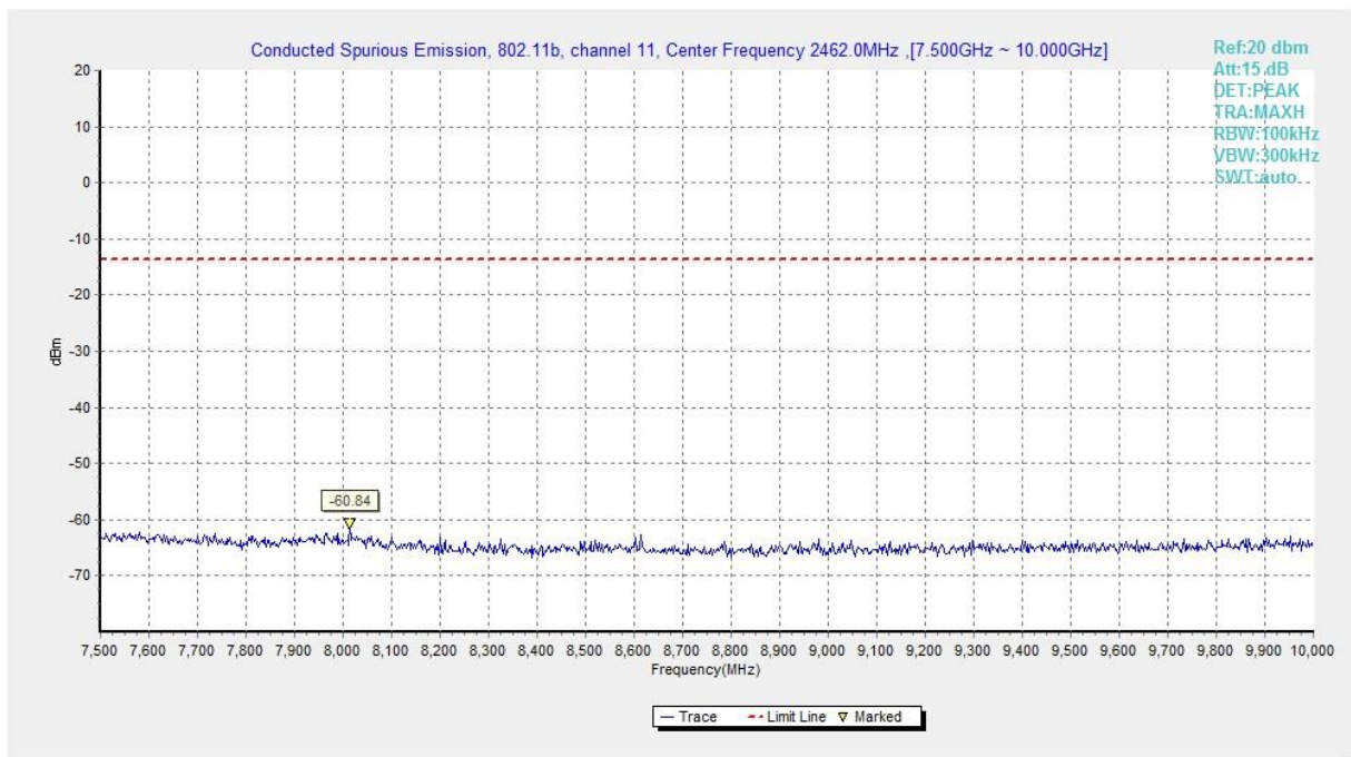
Fig.A.6.1.165 Transmitter Spurious Emission - Conducted (802.11b, Ch11, 7.5 GHz-10 GHz)
