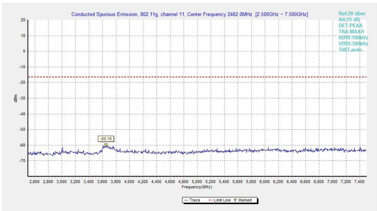
Fig.A.6.1.188 Transmitter Spurious Emission - Conducted (802.11g, Ch11, 2.5 GHz-7.5 GHz)
