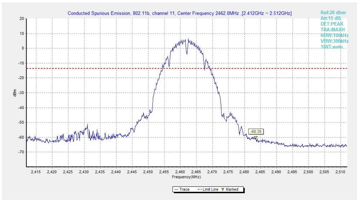
Fig.A.6.1.161 Transmitter Spurious Emission - Conducted (802.11b, Ch11, Center Frequency)
