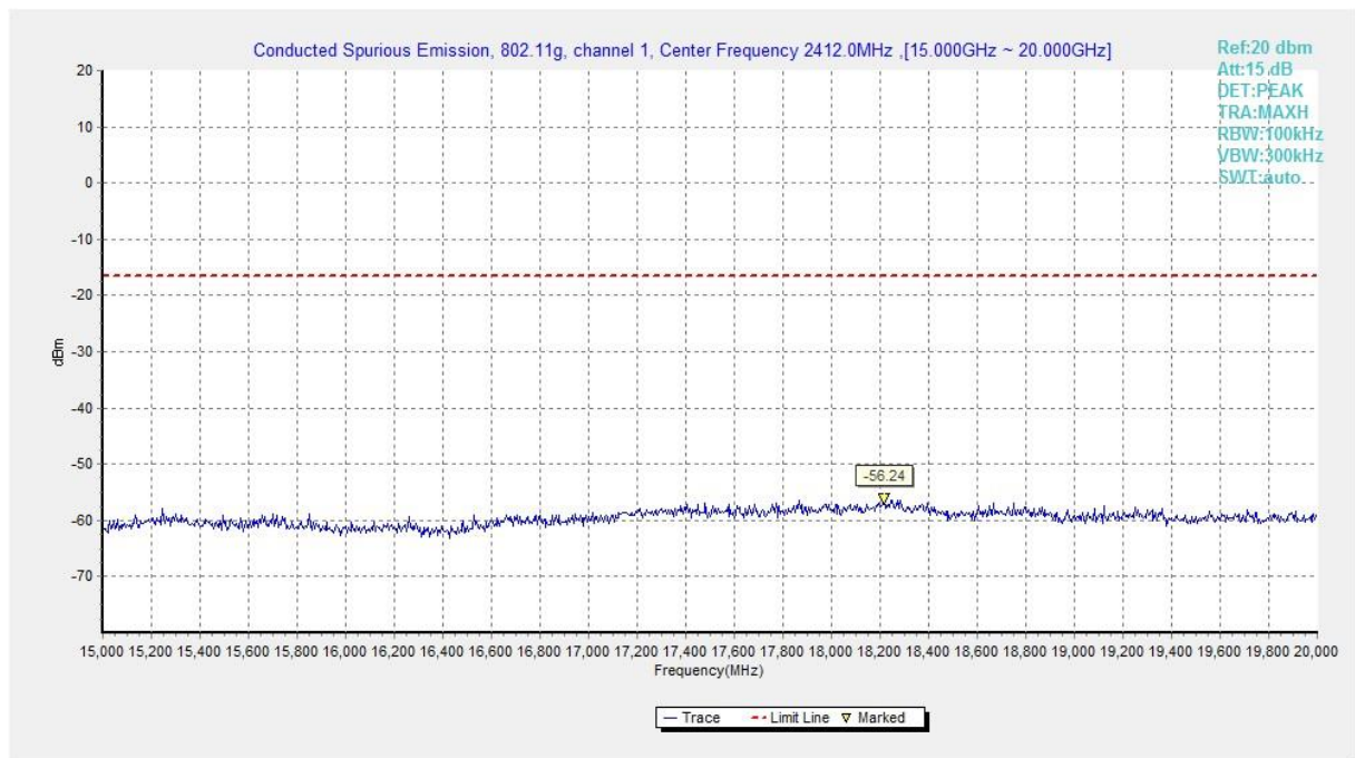
Fig.A.6.1.175 Transmitter Spurious Emission - Conducted (802.11g, Ch1, 15 GHz-20 GHz)
