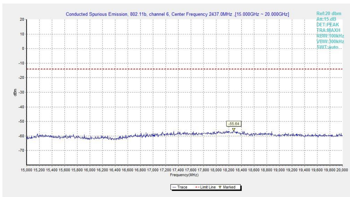
Fig.A.6.1.159 Transmitter Spurious Emission - Conducted (802.11b, Ch6, 15 GHz-20 GHz)
