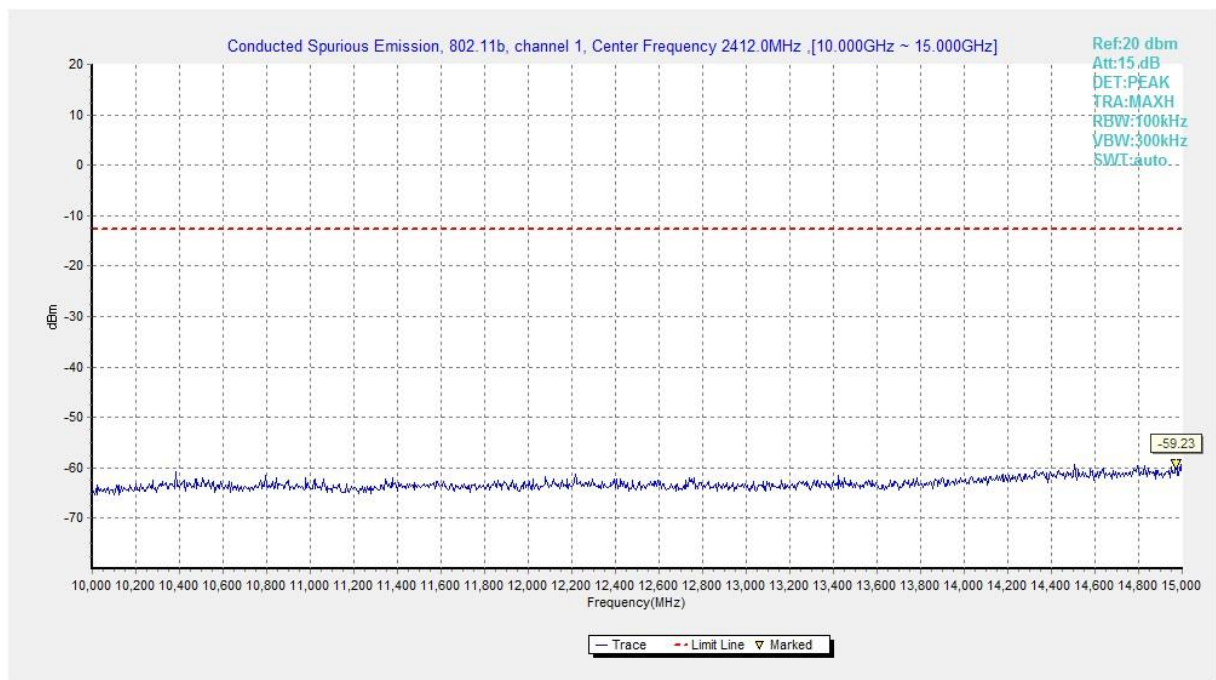
Fig.A.6.1.150 Transmitter Spurious Emission - Conducted (802.11b, Ch1, 10 GHz-15 GHz)
