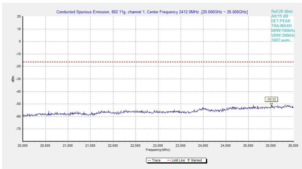
Fig.A.6.1.176 Transmitter Spurious Emission - Conducted (802.11g, Ch1, 20 GHz-26 GHz)
