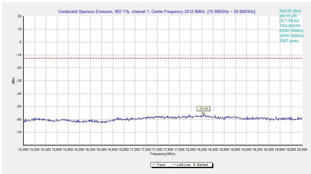
Fig.A.6.1.151 Transmitter Spurious Emission - Conducted (802.11b, Ch1, 15 GHz-20 GHz)
