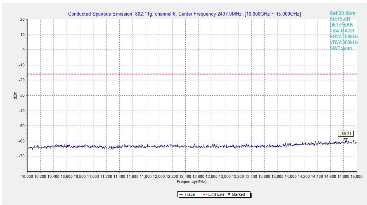
Fig.A.6.1.182 Transmitter Spurious Emission - Conducted (802.11g, Ch6, 10 GHz-15 GHz)
