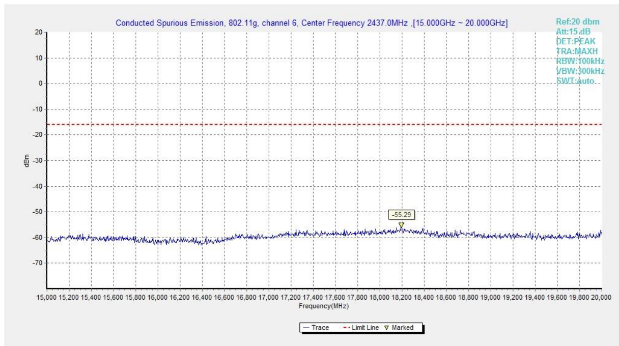
Fig.A.6.1.183 Transmitter Spurious Emission - Conducted (802.11g, Ch6, 15 GHz-20 GHz)
