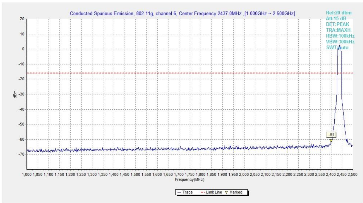
Fig.A.6.1.179 Transmitter Spurious Emission - Conducted (802.11g, Ch6, 1 GHz-2.5 GHz)
