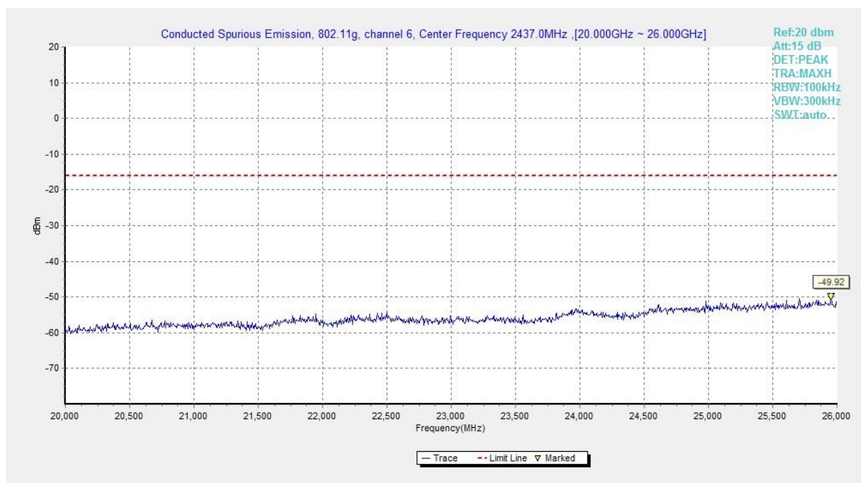
Fig.A.6.1.184 Transmitter Spurious Emission - Conducted (802.11g, Ch6, 20 GHz-26 GHz)
