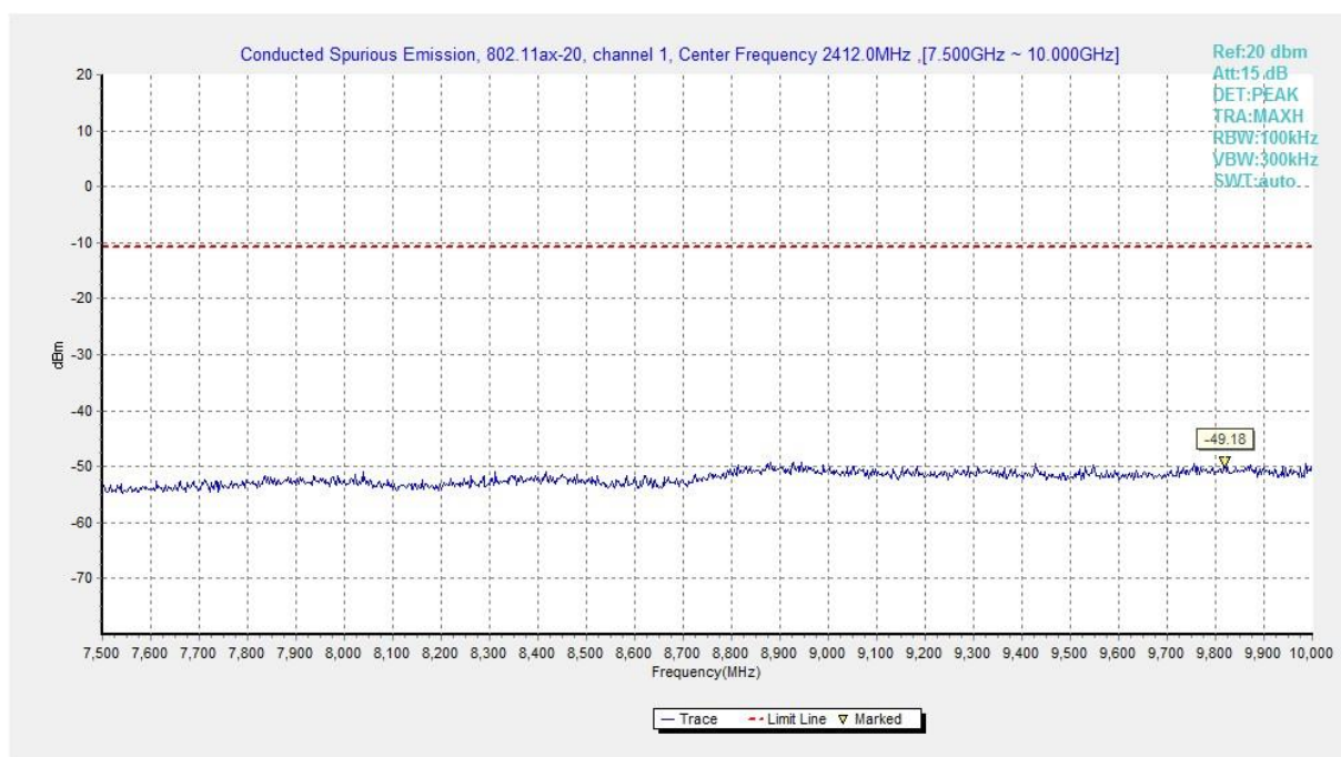
Fig.A.6.1.197 Transmitter Spurious Emission - Conducted (802.11ax-HE20, Ch1, 7.5 GHz-10 GHz)
