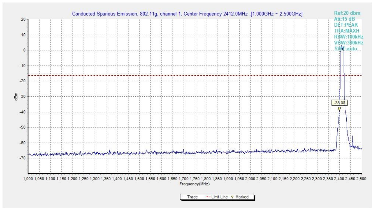
Fig.A.6.1.171 Transmitter Spurious Emission - Conducted (802.11g, Ch1, 1 GHz-2.5 GHz)
