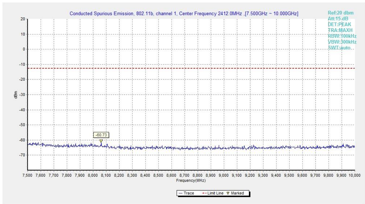
Fig.A.6.1.149 Transmitter Spurious Emission - Conducted (802.11b, Ch1, 7.5 GHz-10 GHz)
