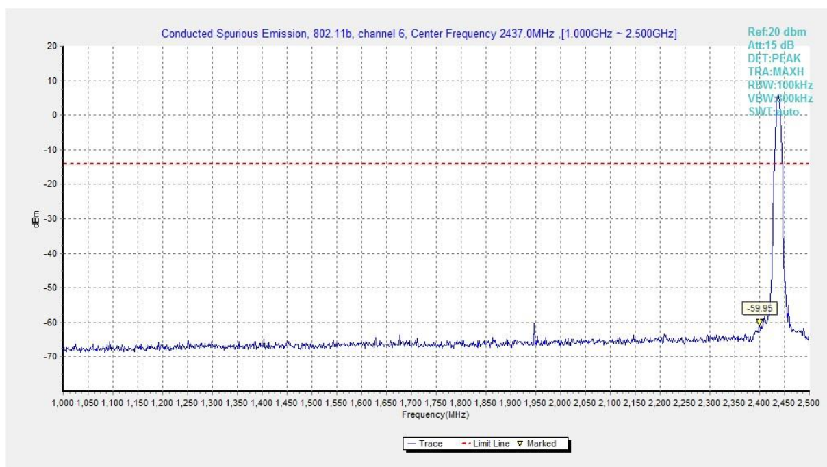
Fig.A.6.1.155 Transmitter Spurious Emission - Conducted (802.11b, Ch6, 1 GHz-2.5 GHz)
