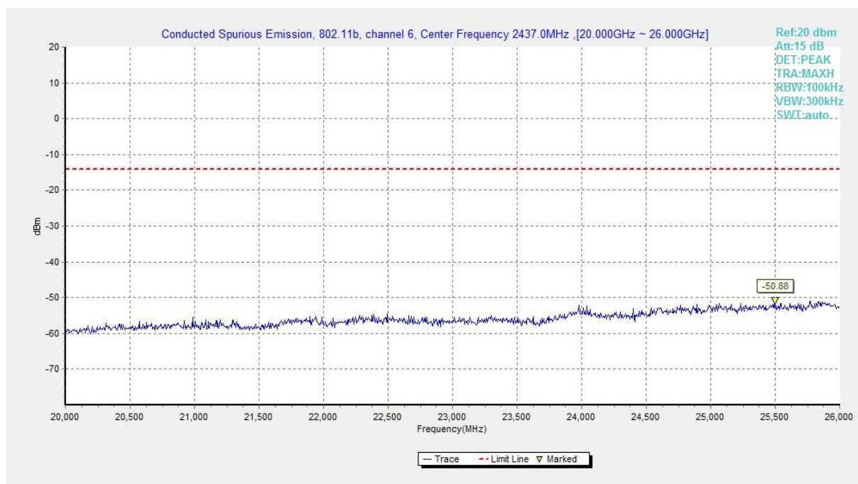
Fig.A.6.1.160 Transmitter Spurious Emission - Conducted (802.11b, Ch6, 20 GHz-26 GHz)
