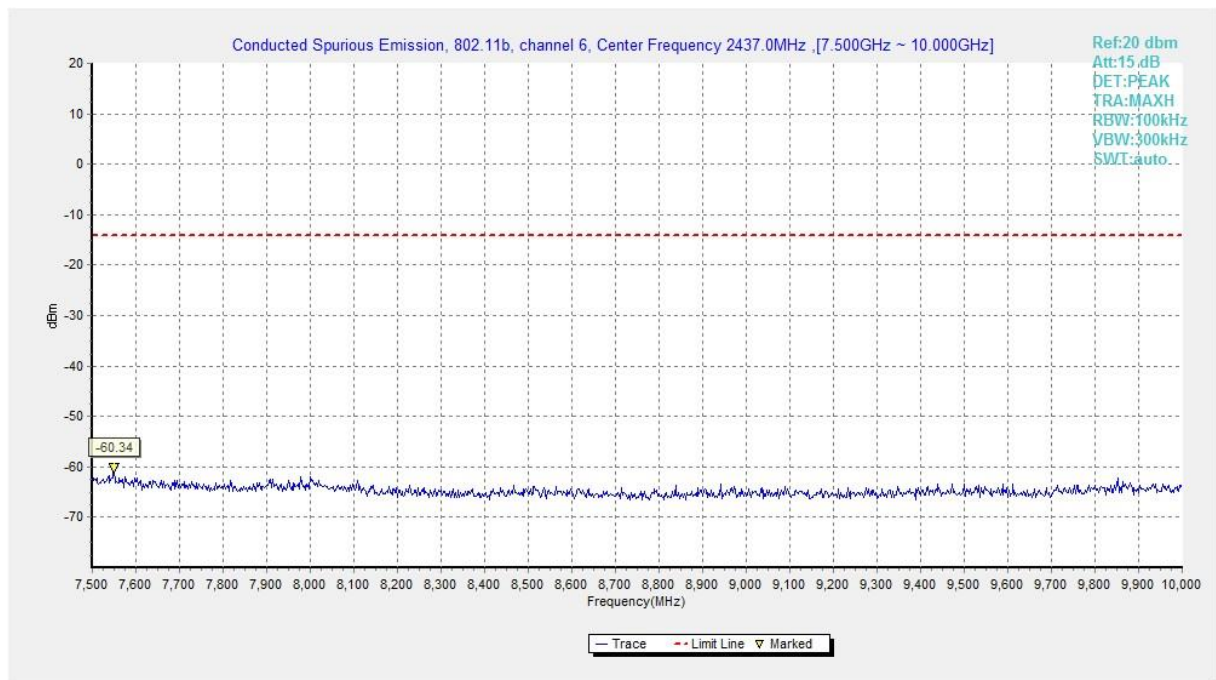
Fig.A.6.1.157 Transmitter Spurious Emission - Conducted (802.11b, Ch6, 7.5 GHz-10 GHz)
