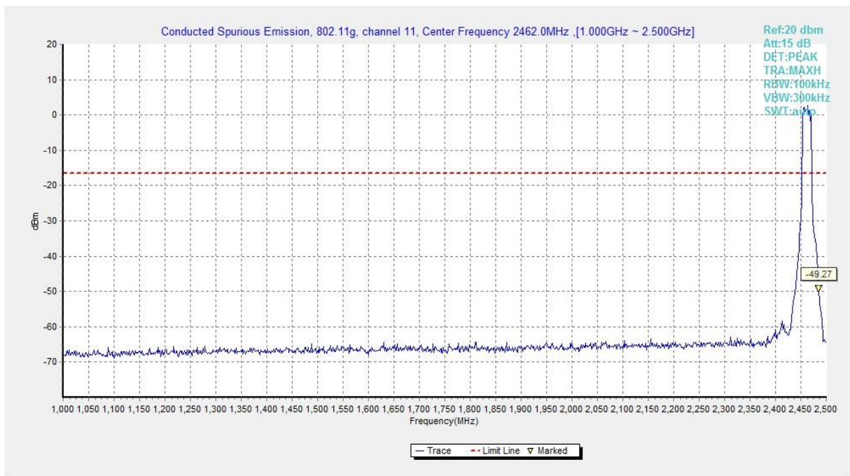
Fig.A.6.1.187 Transmitter Spurious Emission - Conducted (802.11g, Ch11, 1 GHz-2.5 GHz)
