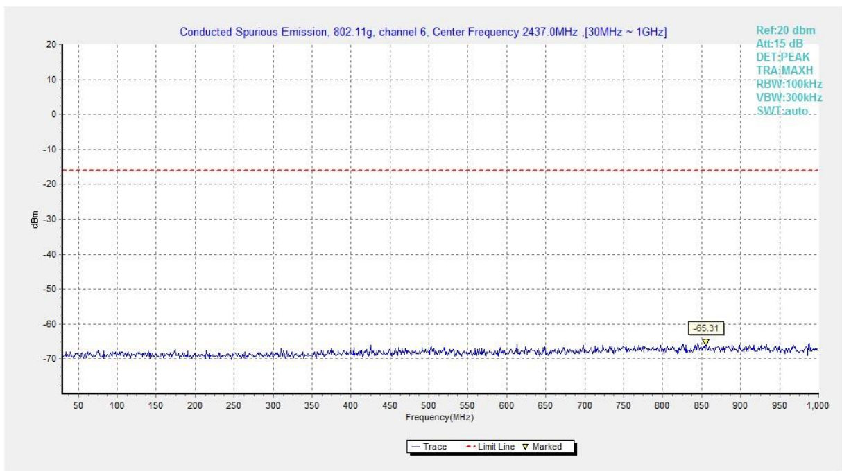
Fig.A.6.1.178 Transmitter Spurious Emission - Conducted (802.11g, Ch6, 30 MHz-1 GHz)
