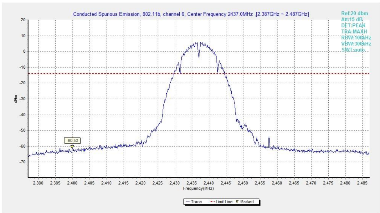
Fig.A.6.1.153 Transmitter Spurious Emission - Conducted (802.11b, Ch6, Center Frequency)
