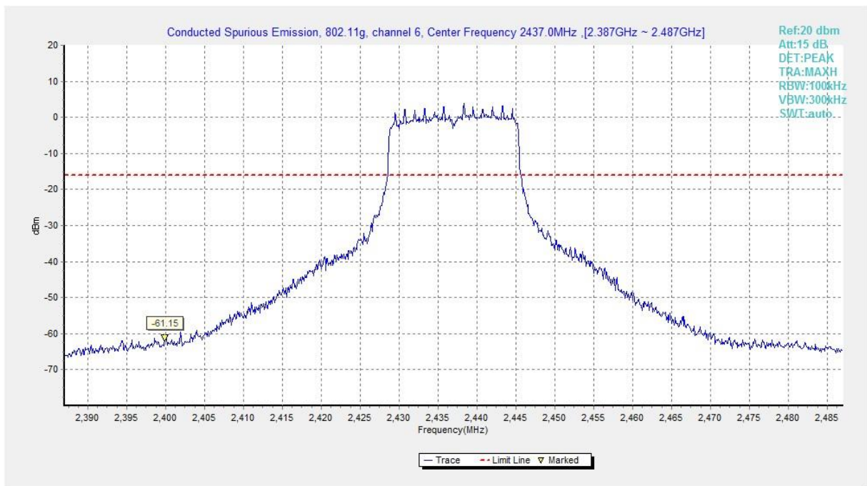
Fig.A.6.1.177 Transmitter Spurious Emission - Conducted (802.11g, Ch6, Center Frequency)
