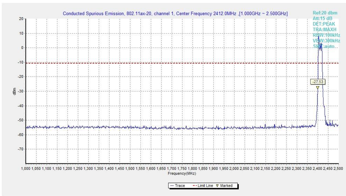
Fig.A.6.1.195 Transmitter Spurious Emission - Conducted (802.11ax-HE20, Ch1, 1 GHz-2.5 GHz)
