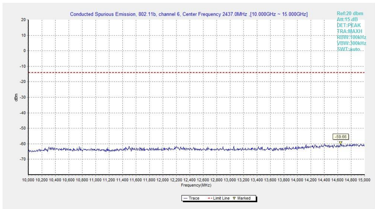
Fig.A.6.1.158 Transmitter Spurious Emission - Conducted (802.11b, Ch6, 10 GHz-15 GHz)
