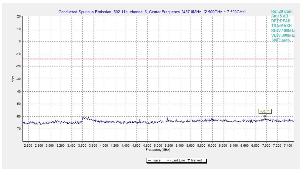
Fig.A.6.1.156 Transmitter Spurious Emission - Conducted (802.11b, Ch6, 2.5 GHz-7.5 GHz)
