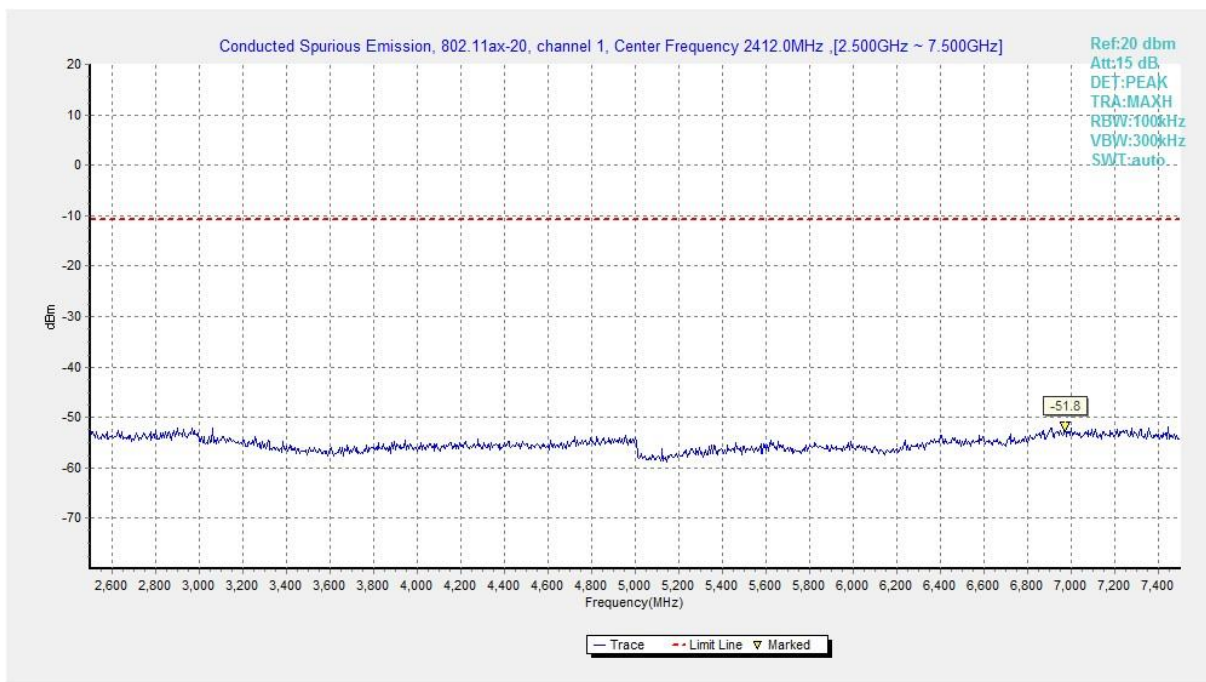
Fig.A.6.1.196 Transmitter Spurious Emission - Conducted (802.11ax-HE20, Ch1, 2.5 GHz-7.5 GHz)
