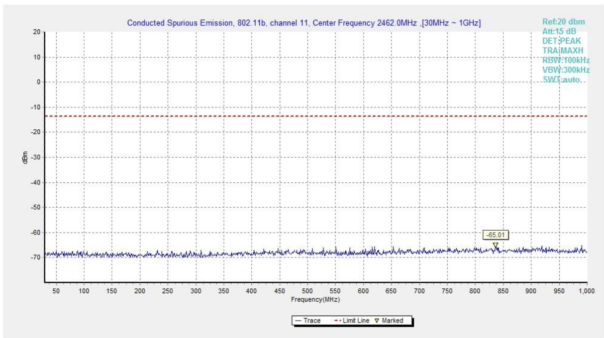
Fig.A.6.1.162 Transmitter Spurious Emission - Conducted (802.11b, Ch11, 30 MHz-1 GHz)
