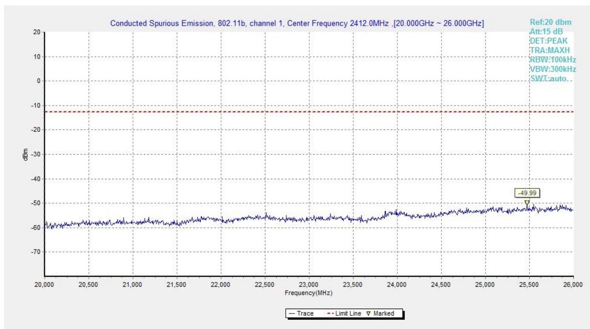
Fig.A.6.1.152 Transmitter Spurious Emission - Conducted (802.11b, Ch1, 20 GHz-26 GHz)
