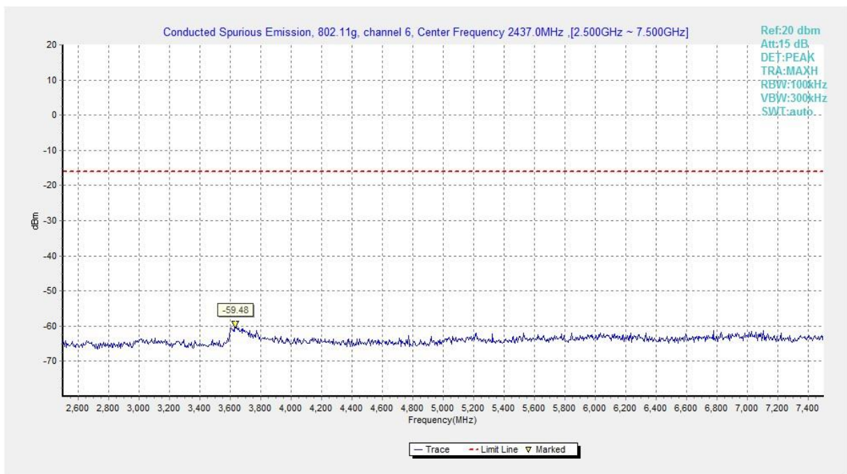
Fig.A.6.1.180 Transmitter Spurious Emission - Conducted (802.11g, Ch6, 2.5 GHz-7.5 GHz)
