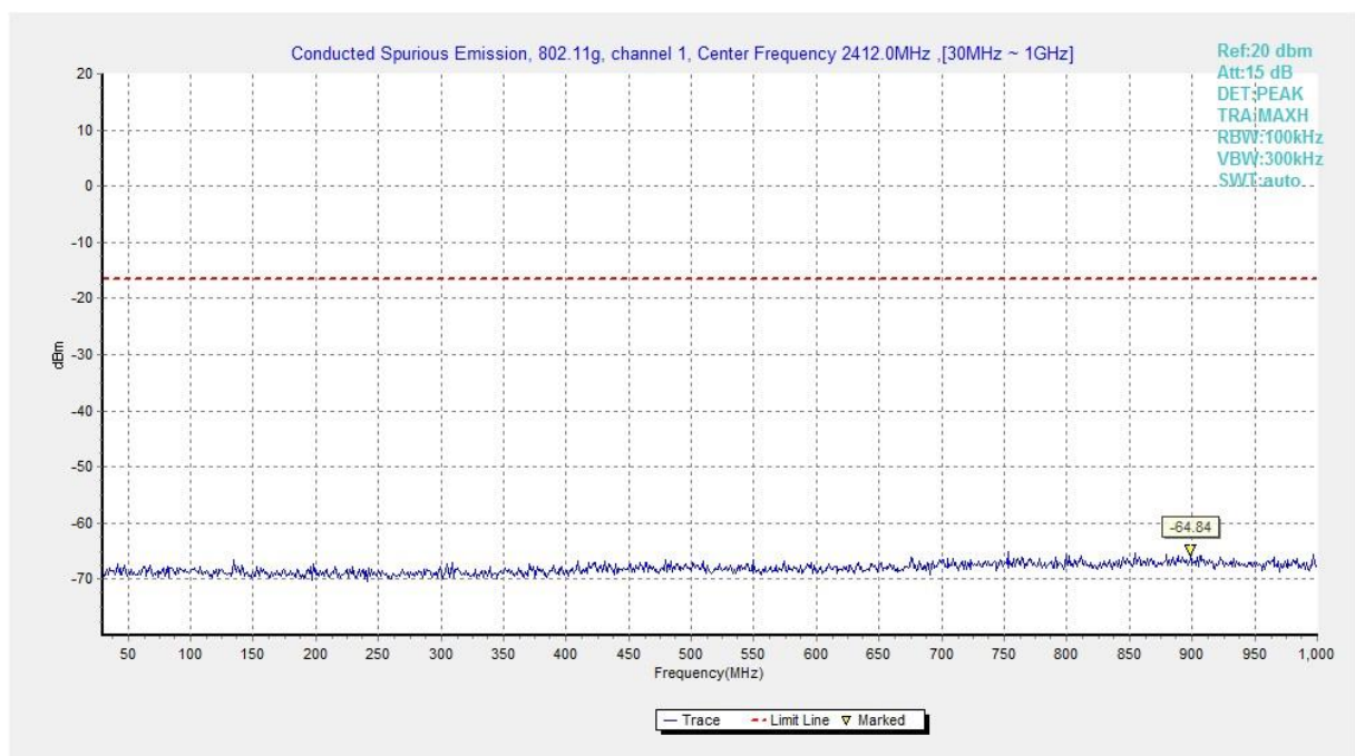
Fig.A.6.1.170 Transmitter Spurious Emission - Conducted (802.11g, Ch1, 30 MHz-1 GHz)
