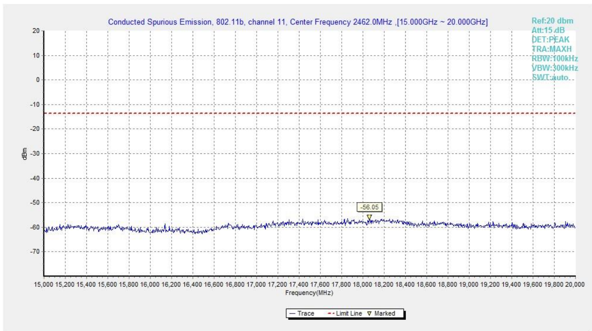
Fig.A.6.1.167 Transmitter Spurious Emission - Conducted (802.11b, Ch11, 15 GHz-20 GHz)
