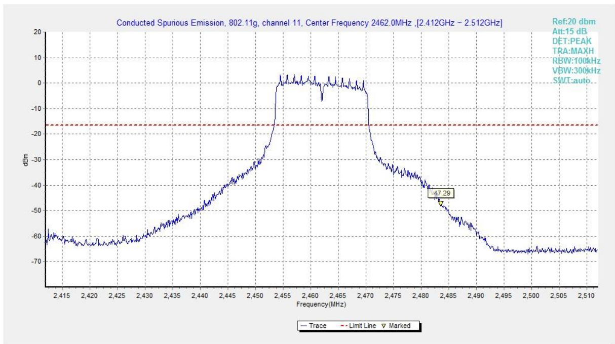
Fig.A.6.1.185 Transmitter Spurious Emission - Conducted (802.11g, Ch11, Center Frequency)
