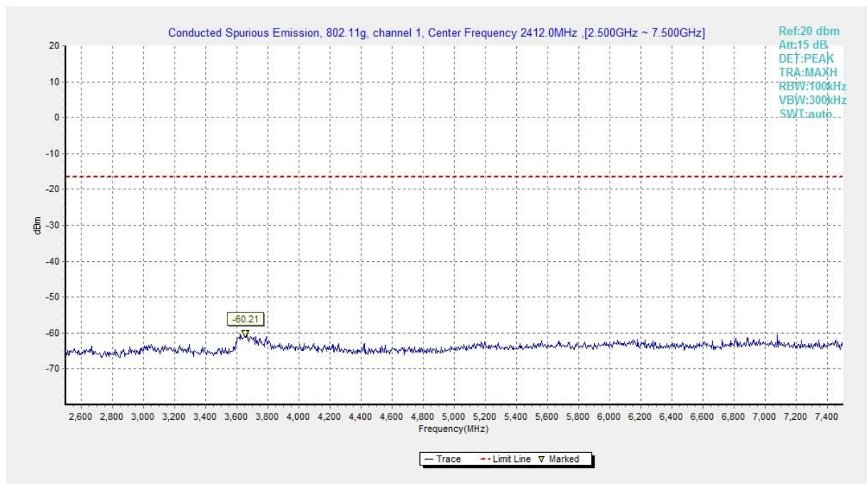
Fig.A.6.1.172 Transmitter Spurious Emission - Conducted (802.11g, Ch1, 2.5 GHz-7.5 GHz)
