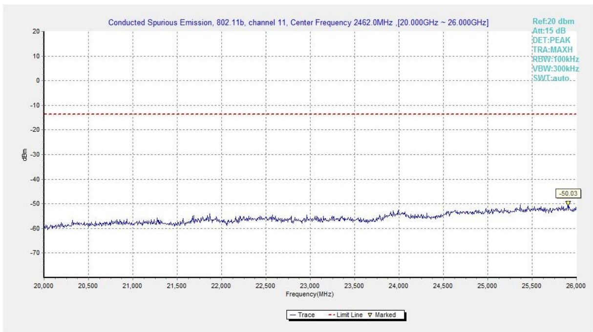
Fig.A.6.1.168 Transmitter Spurious Emission - Conducted (802.11b, Ch11, 20 GHz-26 GHz)
