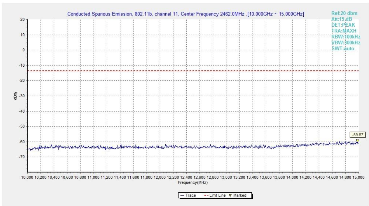
Fig.A.6.1.166 Transmitter Spurious Emission - Conducted (802.11b, Ch11, 10 GHz-15 GHz)
