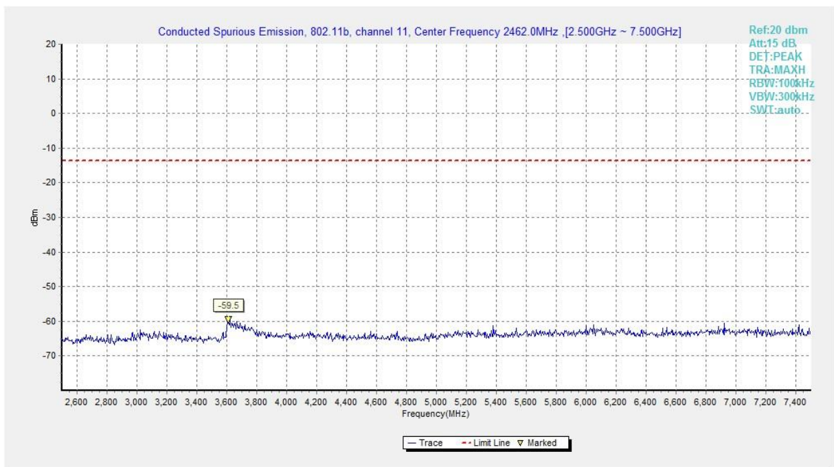
Fig.A.6.1.164 Transmitter Spurious Emission - Conducted (802.11b, Ch11, 2.5 GHz-7.5 GHz)
