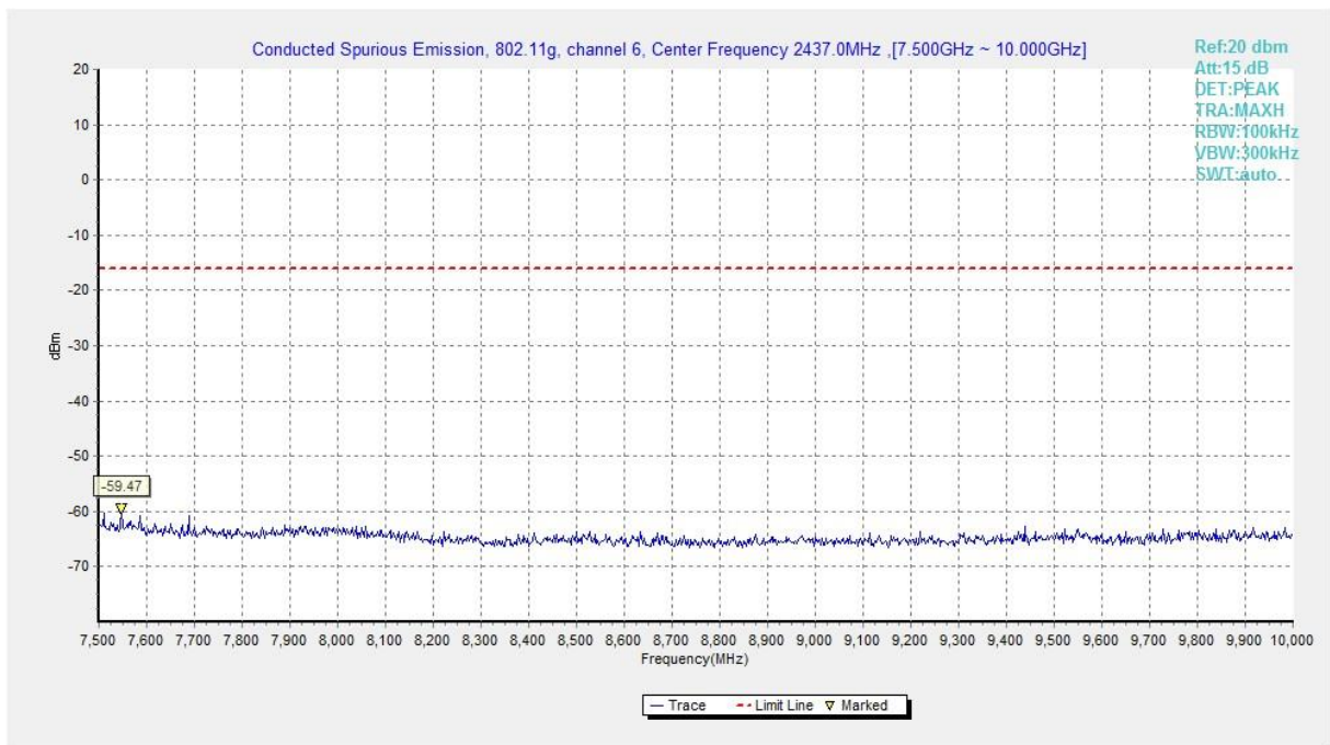
Fig.A.6.1.181 Transmitter Spurious Emission - Conducted (802.11g, Ch6, 7.5 GHz-10 GHz)
