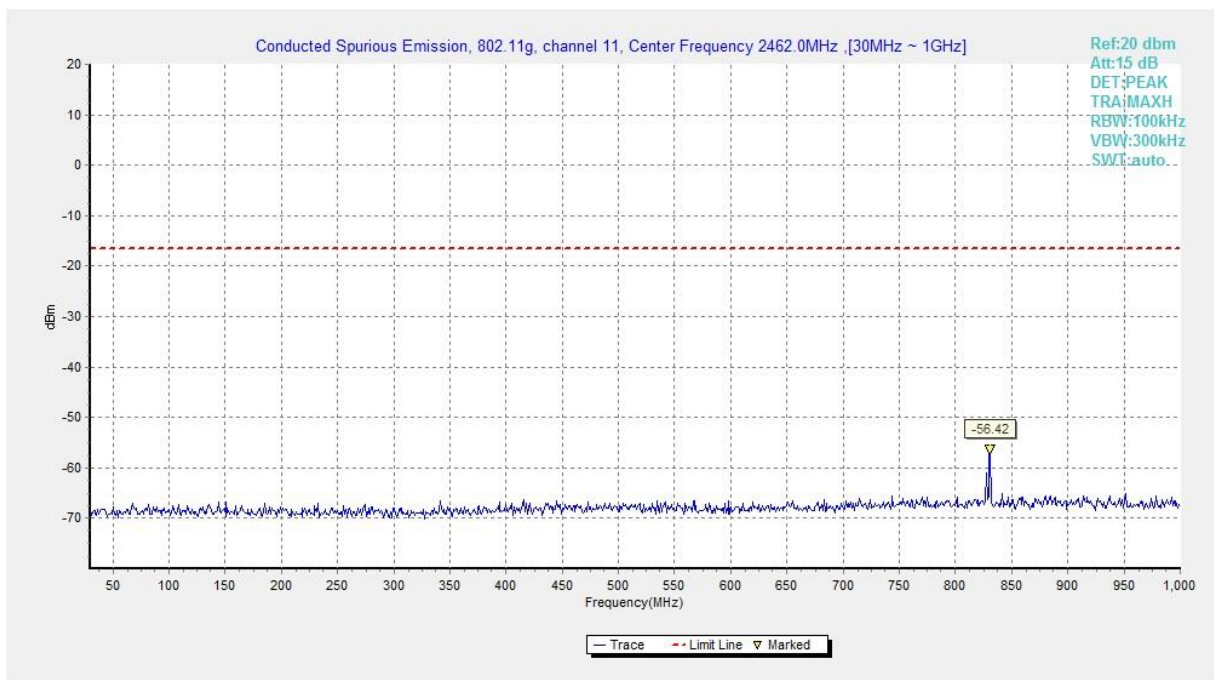
Fig.A.6.1.186 Transmitter Spurious Emission - Conducted (802.11g, Ch11, 30 MHz-1 GHz)
