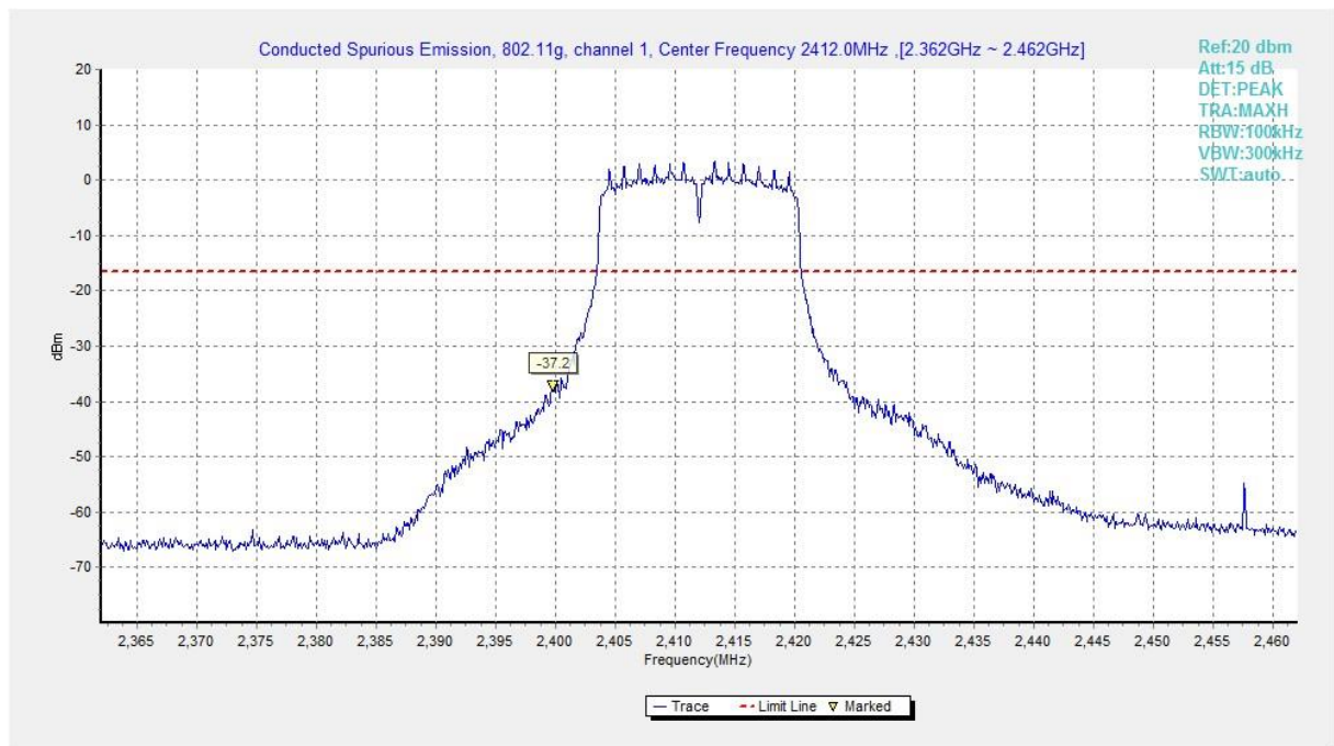
Fig.A.6.1.169 Transmitter Spurious Emission - Conducted (802.11g, Ch1, Center Frequency)
