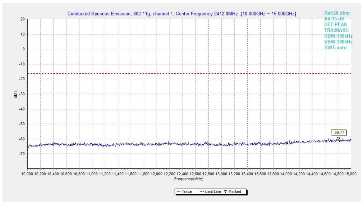
Fig.A.6.1.174 Transmitter Spurious Emission - Conducted (802.11g, Ch1, 10 GHz-15 GHz)
