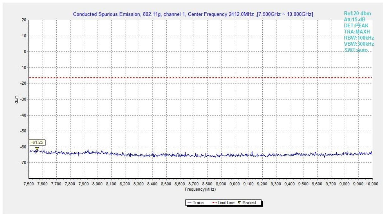
Fig.A.6.1.173 Transmitter Spurious Emission - Conducted (802.11g, Ch1, 7.5 GHz-10 GHz)
