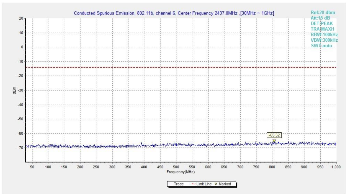
Fig.A.6.1.154 Transmitter Spurious Emission - Conducted (802.11b, Ch6, 30 MHz-1 GHz)
