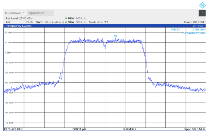
Figure 8.4-34: HDR-Bandwidth 20MHz conducted spurious emission reference level, 2422 MHz
