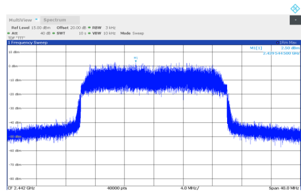
Figure 8.5-13: HDR- Bandwidth 20MHz Power spectral density, 2442 MHz
