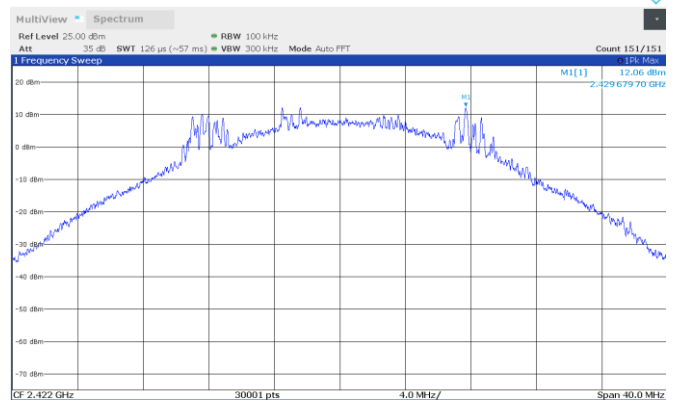
Figure 8.4-30: TSM-Bandwidth 20MHz conducted spurious emission reference level, 2422 MHz
