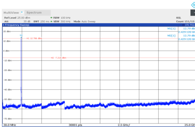
Figure 8.4-33: HDR-Bandwidth 20MHz conducted spurious emission, 2422 MHz
