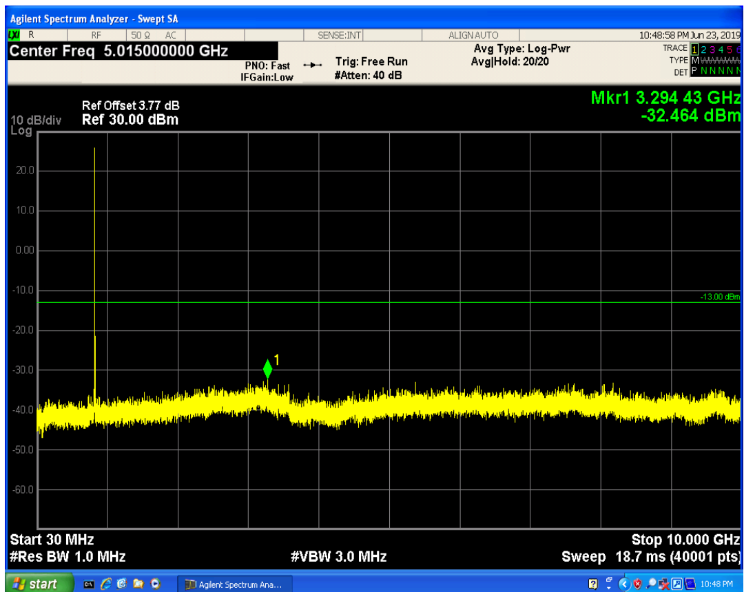
LTE Band5 QPSK BW=3MHz Channel=20635 RB Size=1 Position=#Mid
