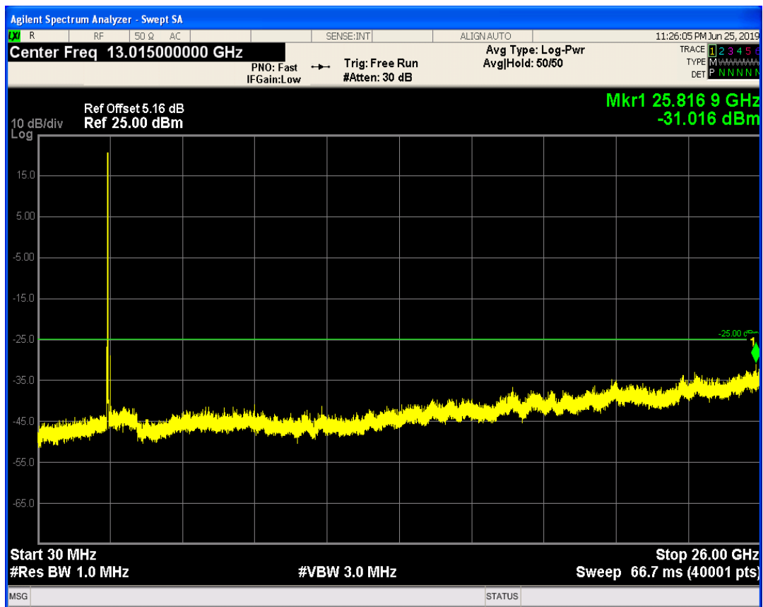
LTE Band41 QPSK BW=15MHz Channel=40115 RB Size=36 Position=#Max
