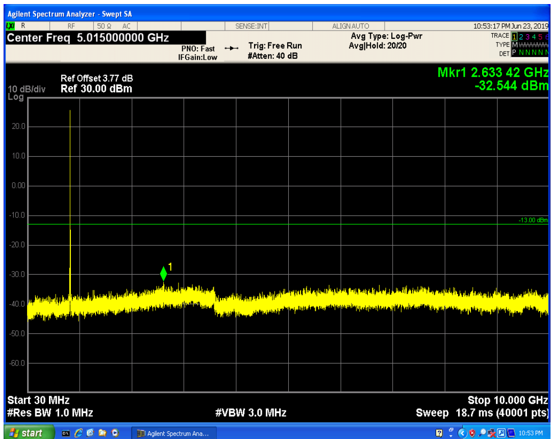
LTE Band5 QAM16 BW=5MHz Channel=20625 RB Size=12 Position=#Max
