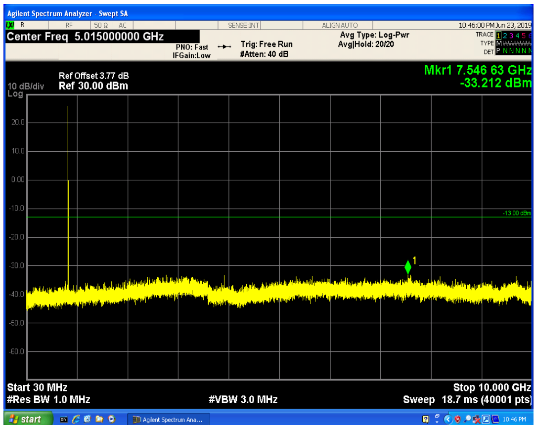
LTE Band5 QPSK BW=1.4MHz Channel=20643 RB Size=3 Position=#0
