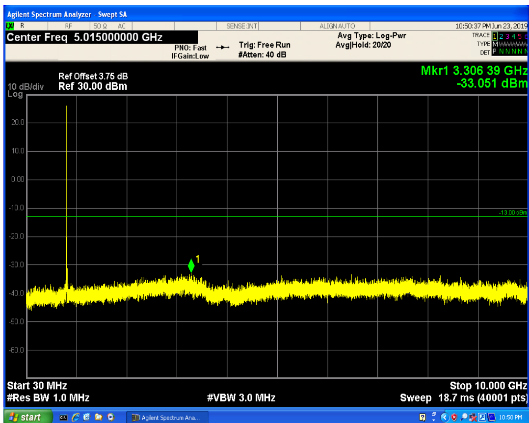
LTE Band5 QPSK BW=5MHz Channel=20425 RB Size=1 Position=#Mid
