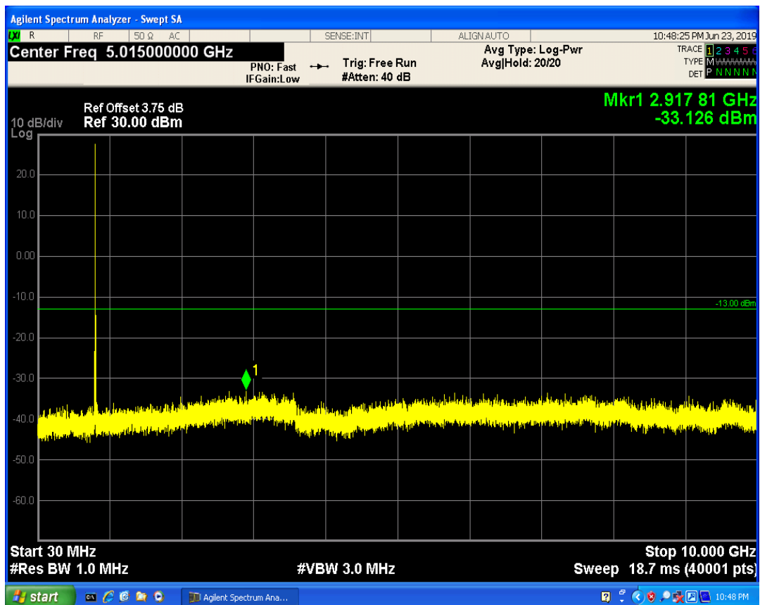
LTE Band5 QAM16 BW=3MHz Channel=20415 RB Size=8 Position=#0
