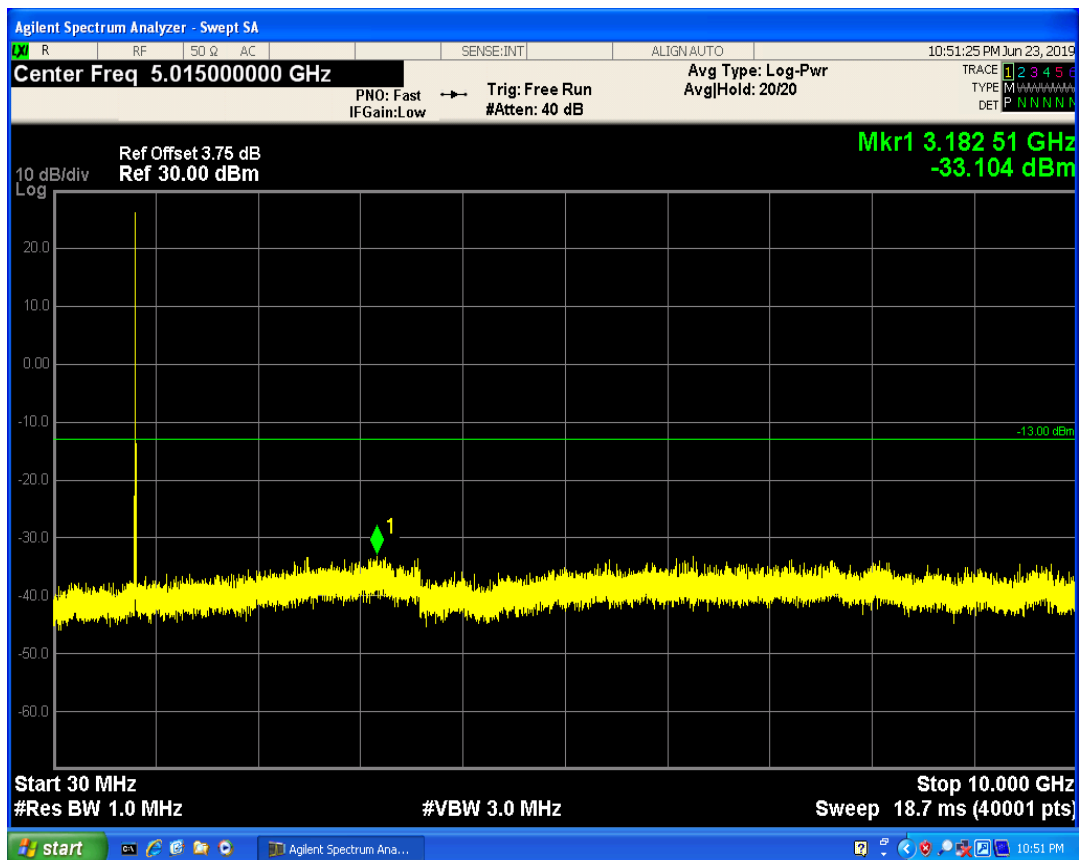
LTE Band5 QAM16 BW=5MHz Channel=20425 RB Size=1 Position=#Mid
