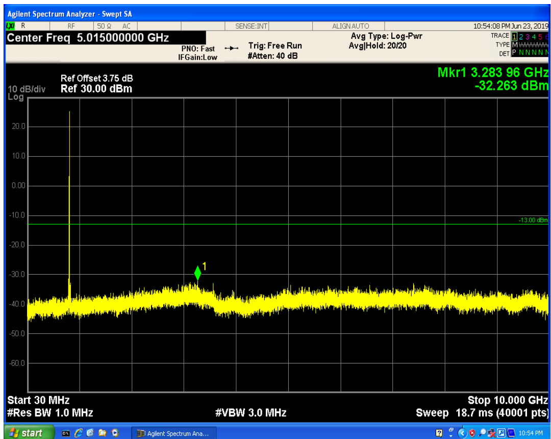
LTE Band5 QPSK BW=10MHz Channel=20450 RB Size=25 Position=#0
