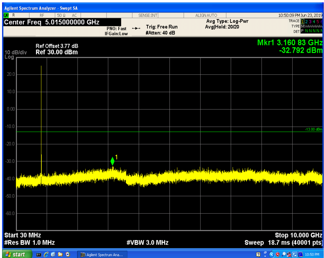
LTE Band5 QAM16 BW=3MHz Channel=20635 RB Size=8 Position=#Max
