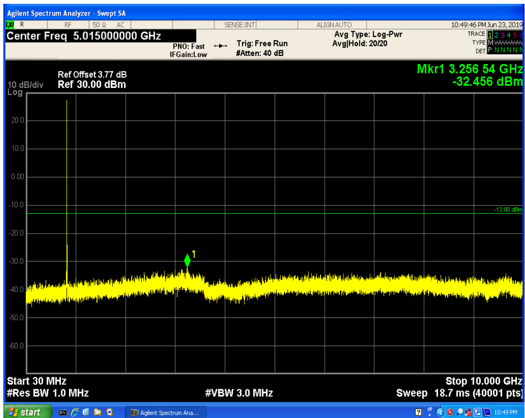
LTE Band5 QAM16 BW=3MHz Channel=20635 RB Size=1 Position=#Mid
