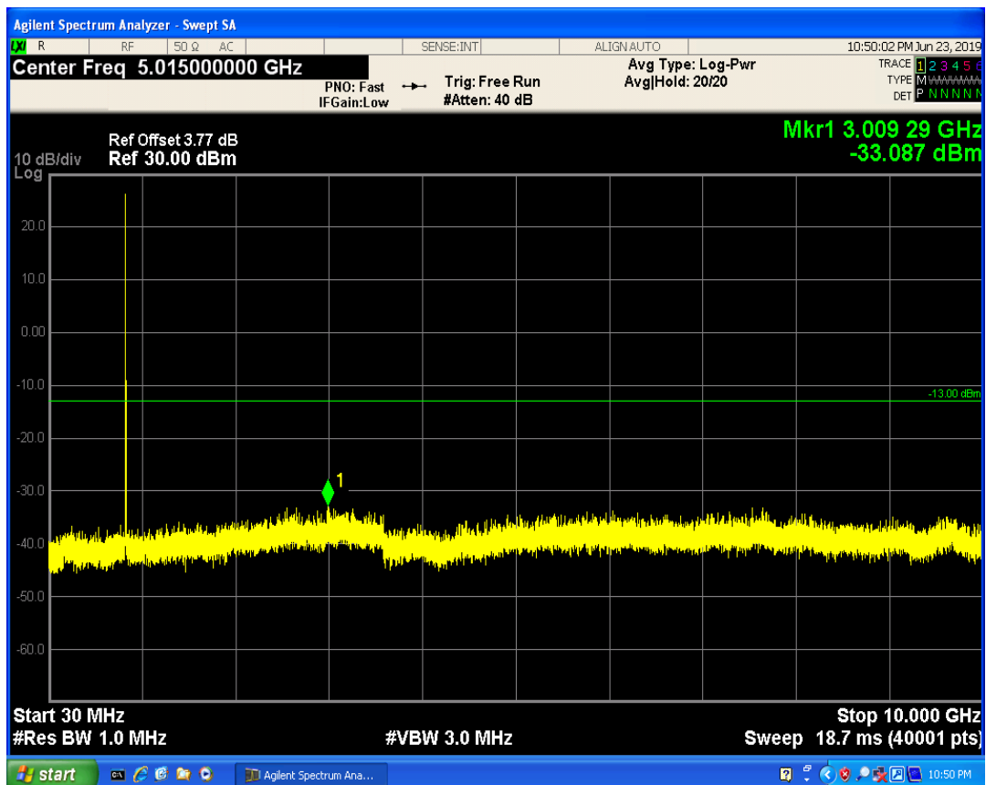
LTE Band5 QAM16 BW=3MHz Channel=20635 RB Size=8 Position=#0
