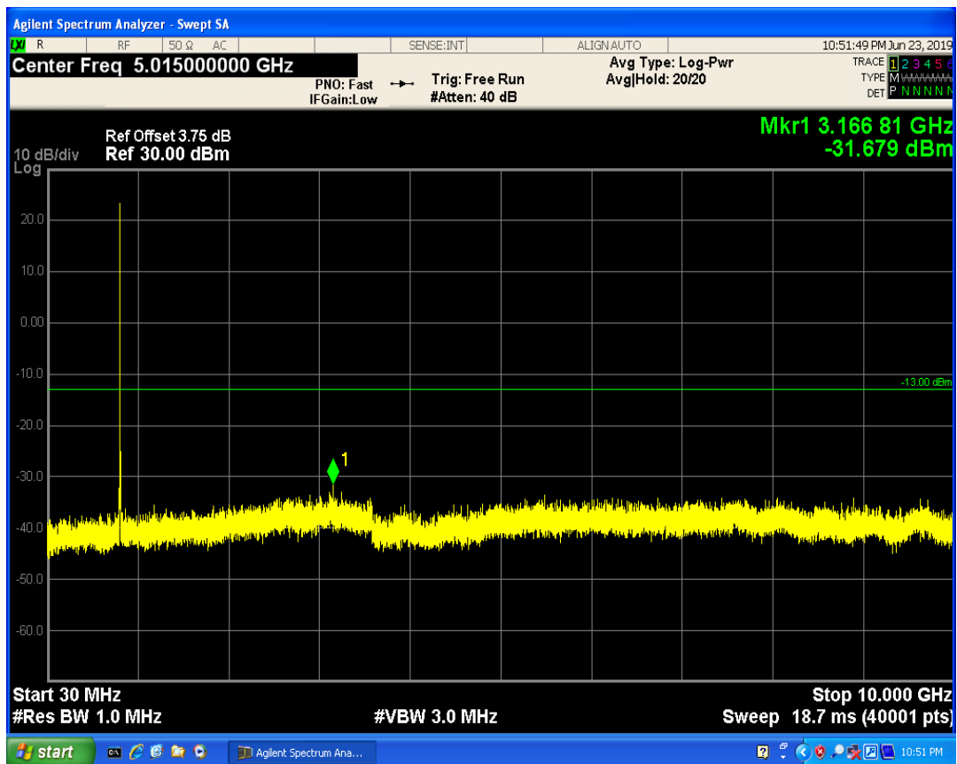
LTE Band5 QAM16 BW=5MHz Channel=20425 RB Size=12 Position=#Max
