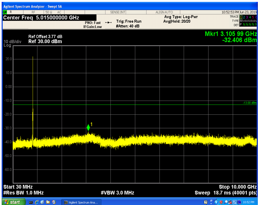
LTE Band5 QAM16 BW=5MHz Channel=20625 RB Size=1 Position=#Mid
