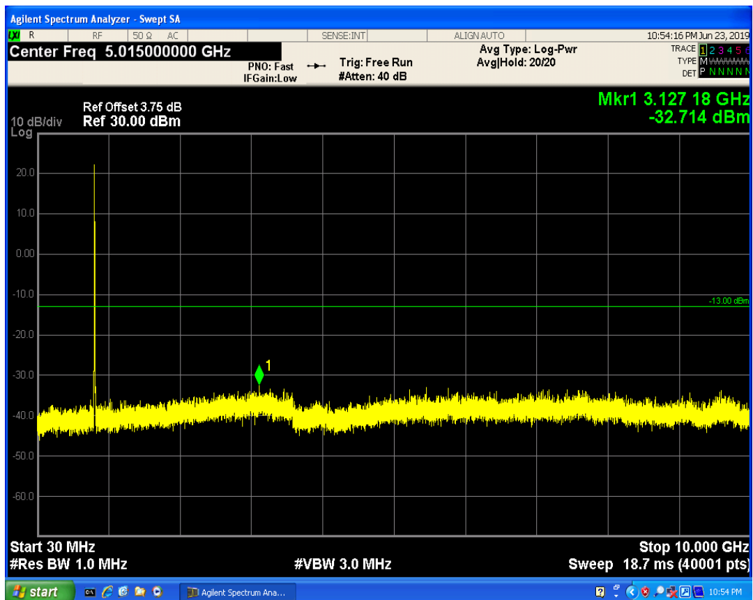
LTE Band5 QPSK BW=10MHz Channel=20450 RB Size=25 Position=#Max
