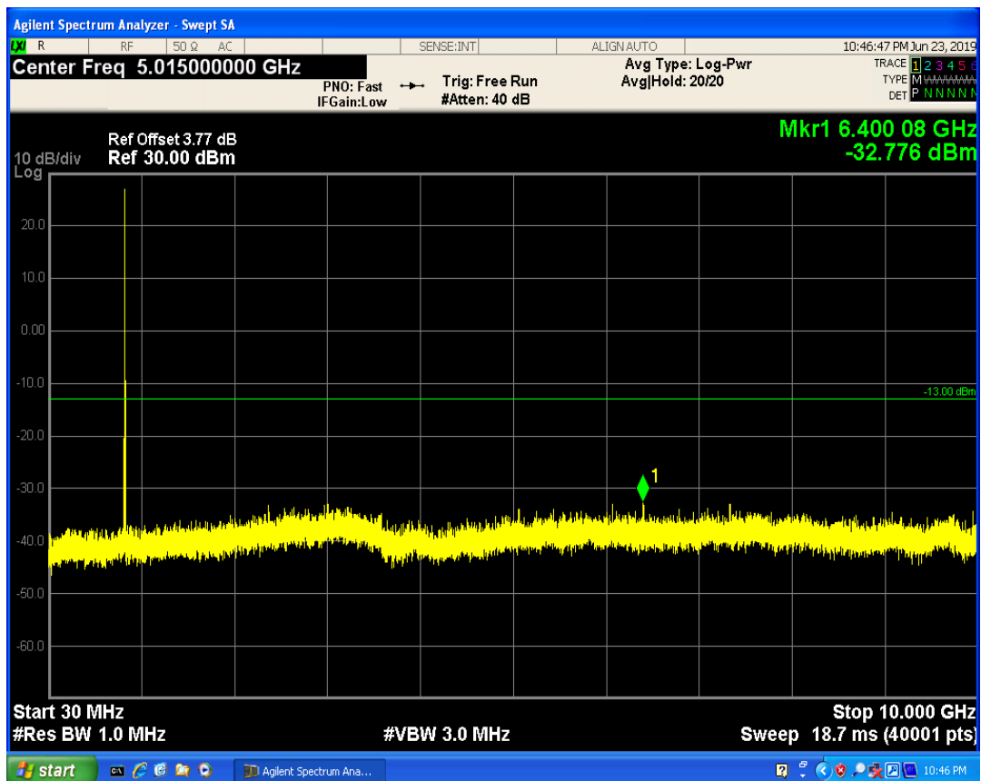
LTE Band5 QAM16 BW=1.4MHz Channel=20643 RB Size=3 Position=#Max
