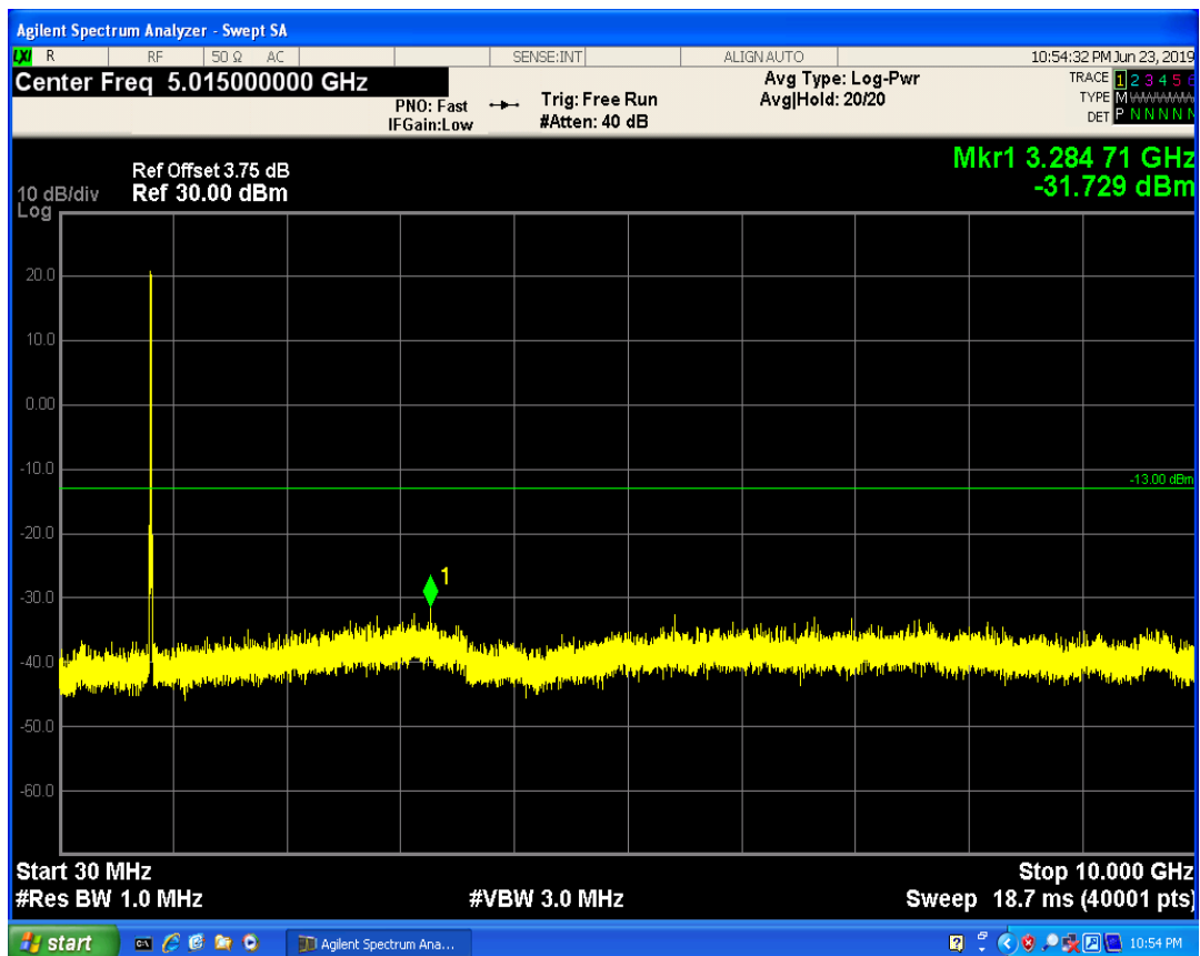
LTE Band5 QAM16 BW=10MHz Channel=20450 RB Size=1 Position=#Mid
