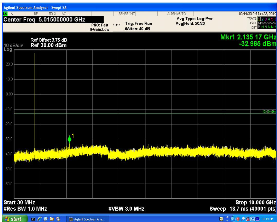
LTE Band5 QPSK BW=1.4MHz Channel=20407 RB Size=3 Position=#Max
