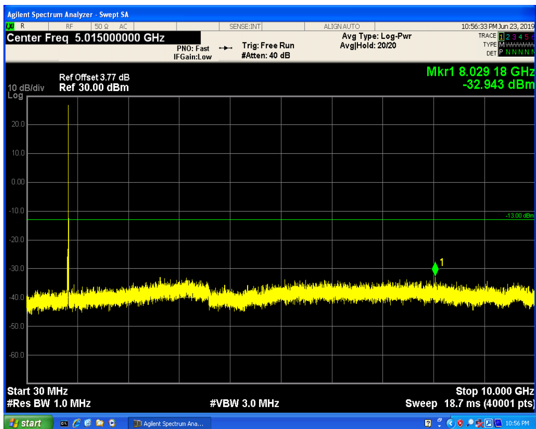
LTE Band5 QAM16 BW=10MHz Channel=20600 RB Size=25 Position=#0
