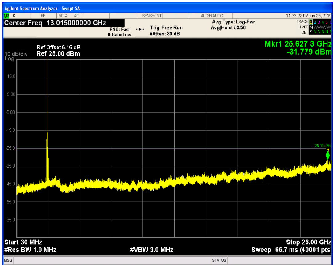
LTE Band41 QPSK BW=20MHz Channel=40140 RB Size=1 Position=#Max
