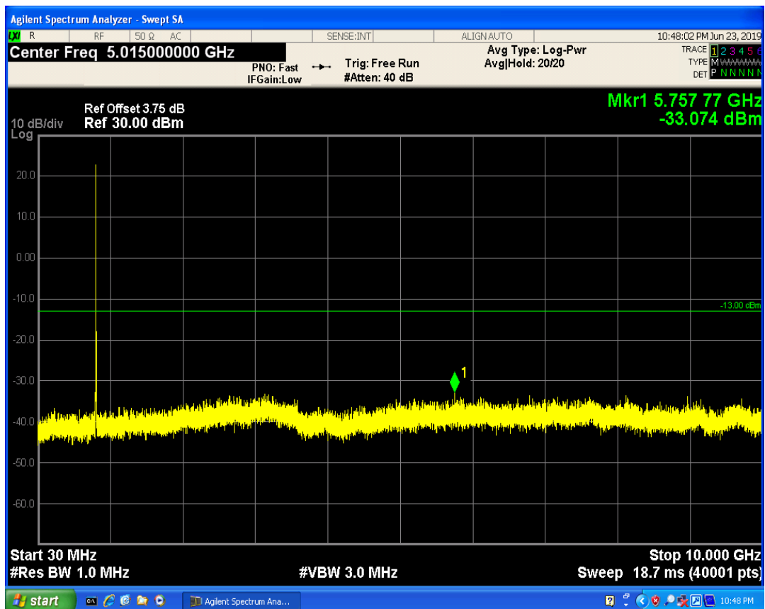
LTE Band5 QAM16 BW=3MHz Channel=20415 RB Size=1 Position=#Mid
