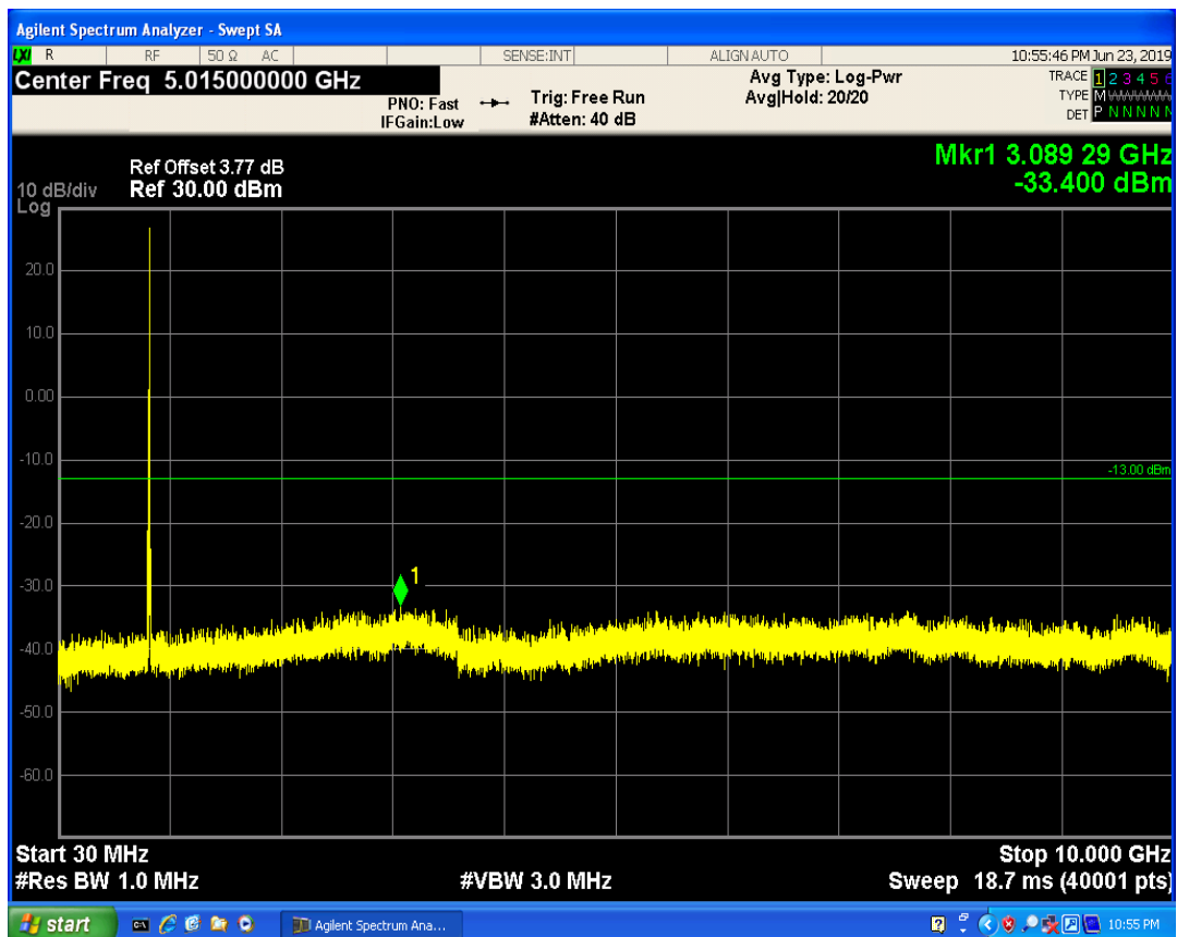
LTE Band5 QPSK BW=10MHz Channel=20600 RB Size=25 Position=#0
