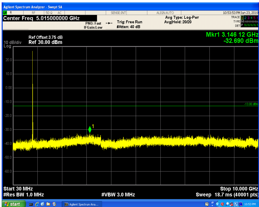
LTE Band5 QPSK BW=10MHz Channel=20450 RB Size=1 Position=#Mid
