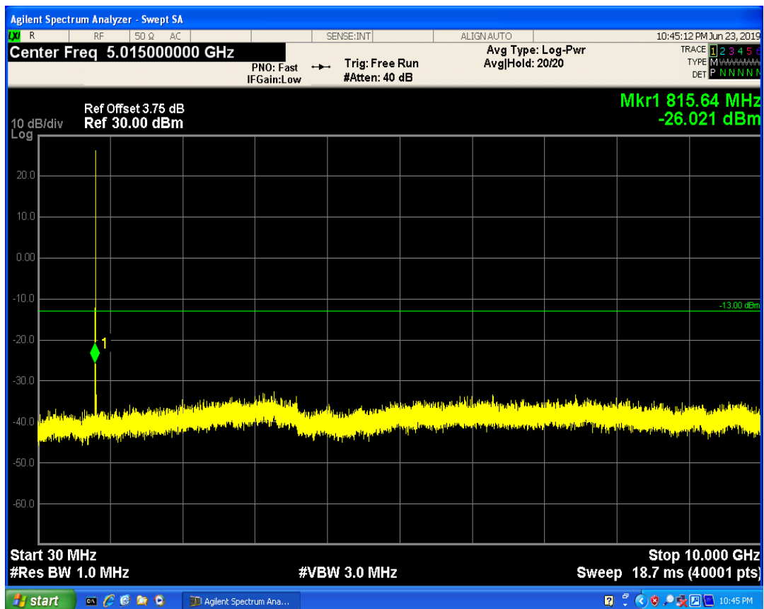
LTE Band5 QAM16 BW=1.4MHz Channel=20407 RB Size=3 Position=#0
