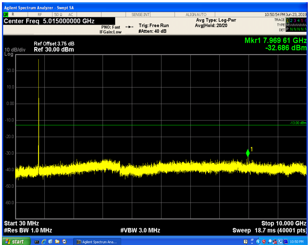
LTE Band5 QPSK BW=5MHz Channel=20425 RB Size=12 Position=#Max
