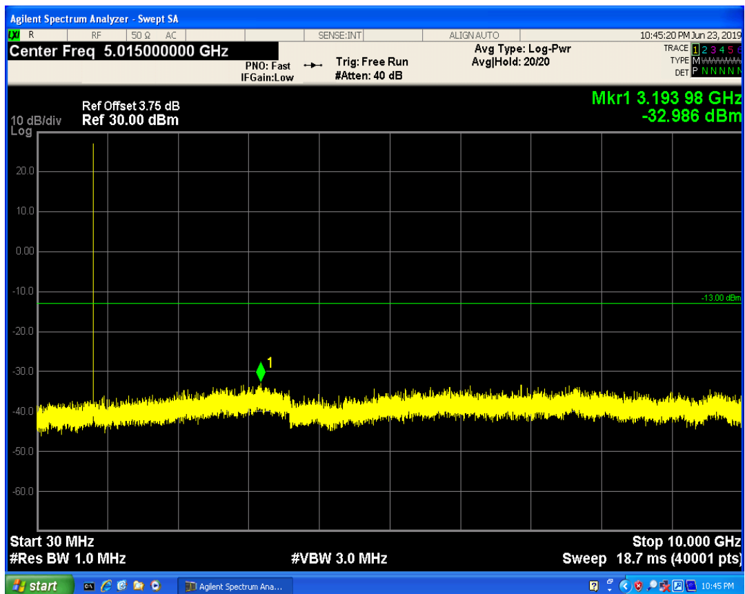
LTE Band5 QAM16 BW=1.4MHz Channel=20407 RB Size=3 Position=#Max
