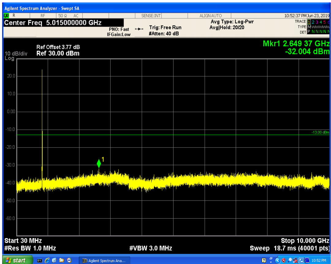
LTE Band5 QPSK BW=5MHz Channel=20625 RB Size=12 Position=#Max
