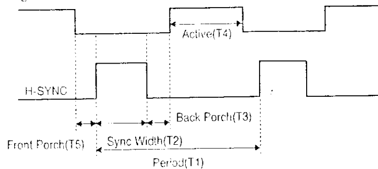
( FIG.1 H-SYNC )
