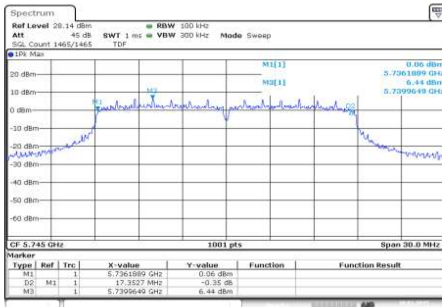
Plot 4: OFDM/n-mode, single antenna, antenna 1, 5745 MHz
