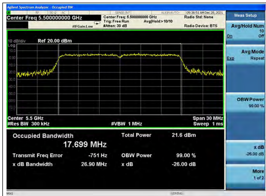
(Channel 100, 5500MHz, 802.11n (HT20))
