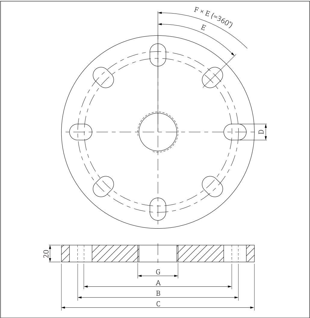
36 Dimensions of UNI flange, engineering unit: mm
