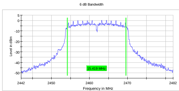
DTS BW, 2462 MHz, 802.11g 6M
