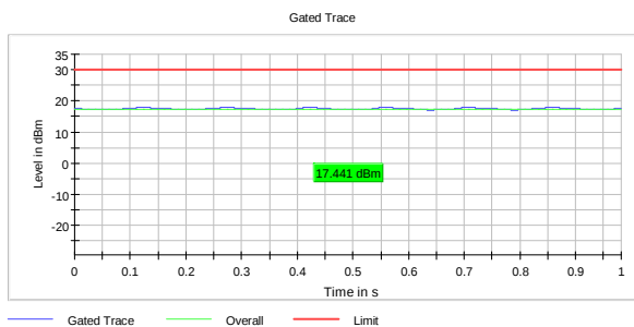
RMS Power, 2457 MHz, 802.11b 1M
