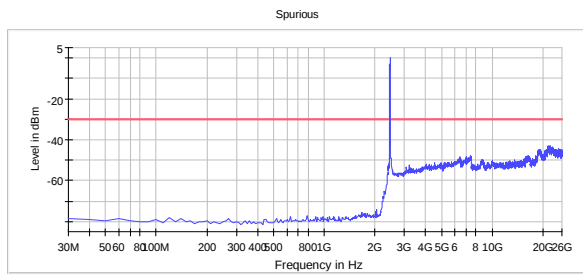
Conducted Emissions Ch11, 802.11n MCS0 SISO
