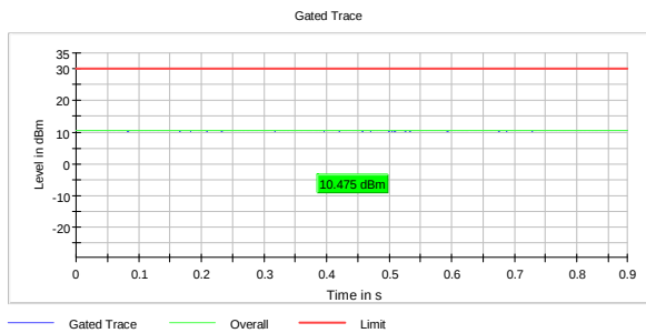
RMS Power, 2452 MHz, 802.11n HT40 SISO MCS0
