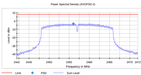
PSD, 2457 MHz, 802.11n MIMO MCS8 -3.29
