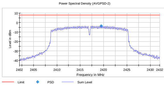
PSD, 2417 MHz, 802.11g 6M -3.56
