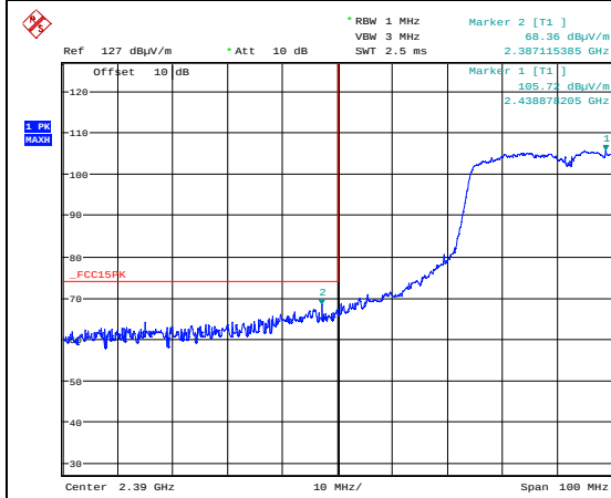
Band Edge, 2427 MHz, 802.11n HT40 MCS0, Max: Ant 0, Peak PL14
