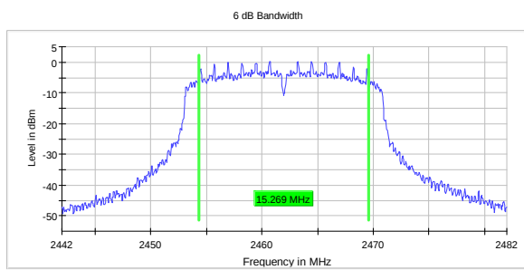
DTS BW, 2462 MHz, 802.11n SISO MCS0
