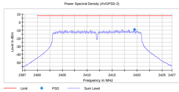
PSD, 2412 MHz, 802.11n MIMO MCS15 -9.17
