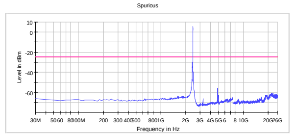
Conducted Emissions Ch06, 802.11n MCS8 MIMO
