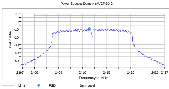
PSD, 2412 MHz, 802.11g 6M -9.50
