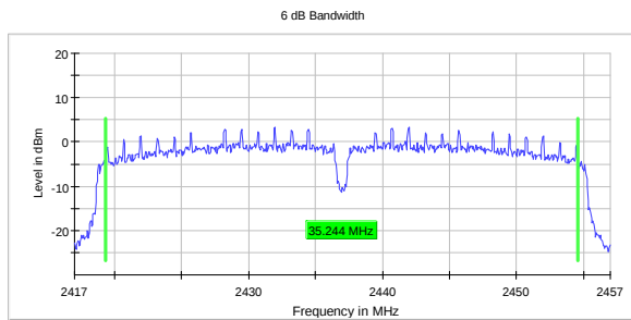
DTS BW, 2437 MHz, 802.11n HT40 SISO MCS0
