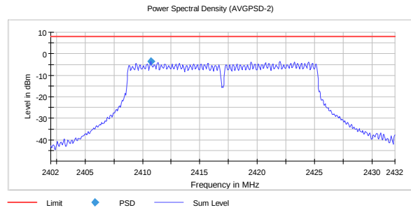
PSD, 2417 MHz, 802.11g 54M -3.52
