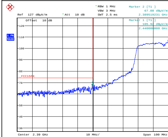
Band Edge, 2432 MHz, 802.11n HT40 MCS0, Max: Ant 0, Peak PL16
