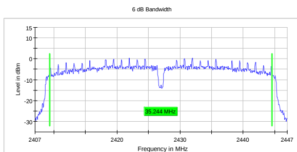
DTS BW, 2427 MHz, 802.11n HT40 MIMO MCS8
