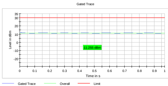
RMS Power, 2462 MHz, 802.11b 1M
