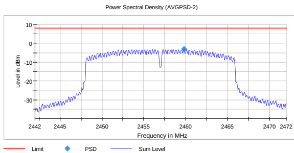
PSD, 2457 MHz, 802.11n SISO MCS0 -2.86
