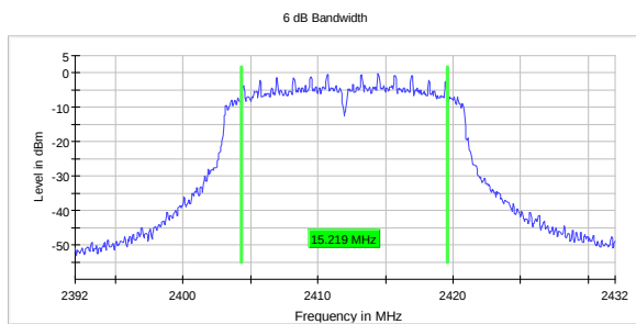
DTS BW, 2412 MHz, 802.11n SISO MCS0
