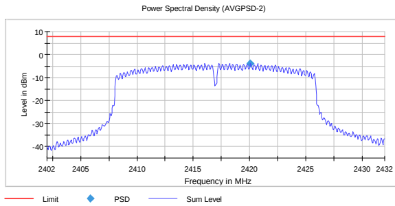
PSD, 2417 MHz, 802.11n SISO MCS0 -3.93
