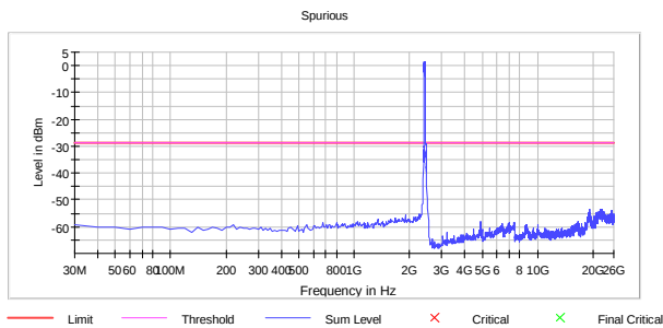
Conducted Emissions Ch07 802.11n HT40 MCS0 SISO
