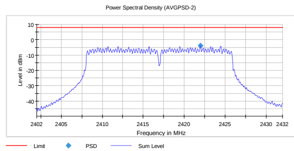
PSD, 2417 MHz, 802.11n MIMO MCS15 -3.78
