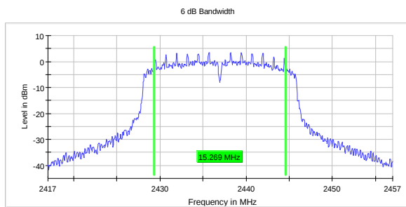
DTS BW, 2437 MHz, 802.11n MIMO MCS8
