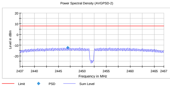
PSD, 2452 MHz, 802.11n HT40 MIMO MCS8 -12.4
