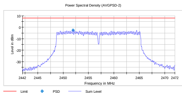
PSD, 2457 MHz, 802.11g 54M -2.66
