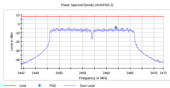
PSD, 2457 MHz, 802.11n MIMO MCS15 -4.13
