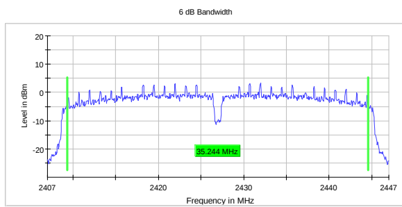
DTS BW, 2427 MHz, 802.11n HT40 SISO MCS0
