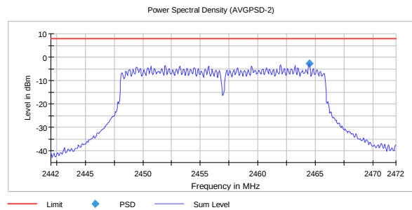
PSD, 2457 MHz, 802.11n SISO MCS7 -2.72
