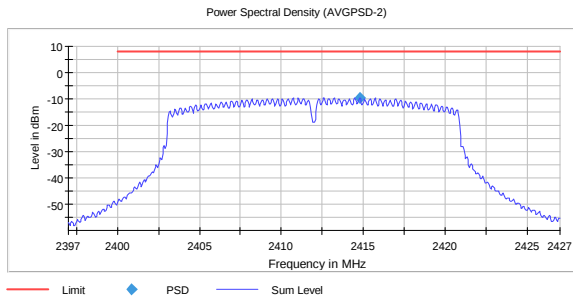
PSD, 2412 MHz, 802.11n MIMO MCS8 -9.63
