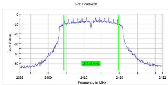
DTS BW, 2412 MHz, 802.11n MIMO MCS8
