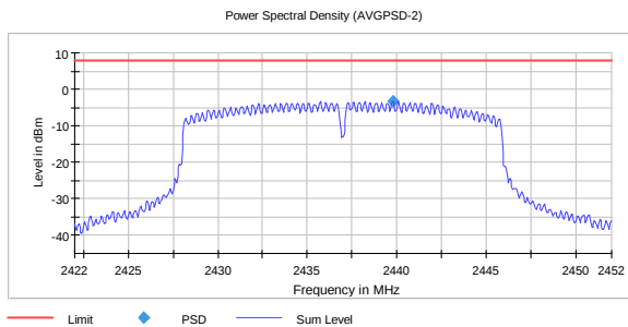
PSD, 2437 MHz, 802.11n SISO MCS0 -3.30
