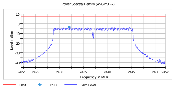
PSD, 2437 MHz, 802.11g 54M -3.31
