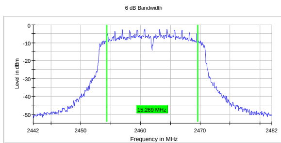
DTS BW, 2462 MHz, 802.11n MIMO MCS8
