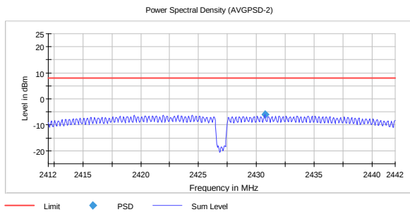
PSD, 2427 MHz, 802.11n HT40 MIMO MCS8 -6.1
