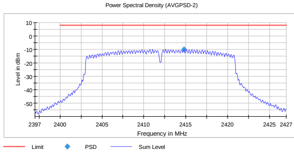
PSD, 2412 MHz, 802.11n SISO MCS0 -9.96
