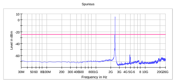
Conducted Emissions Ch06, 802.11g 6M
