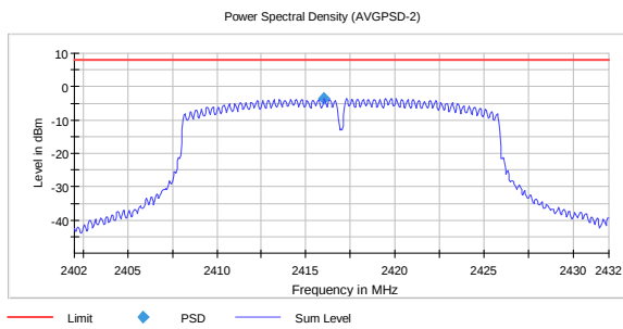
PSD, 2417 MHz, 802.11n MIMO MCS8 -3.55
