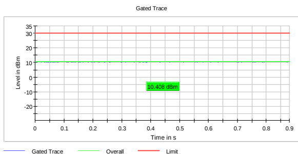
RMS Power, 2422 MHz, 802.11n HT40 MIMO MCS8
