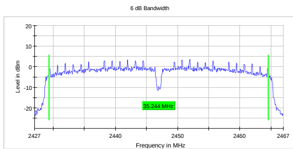
DTS BW, 2447 MHz, 802.11n HT40 SISO MCS0
