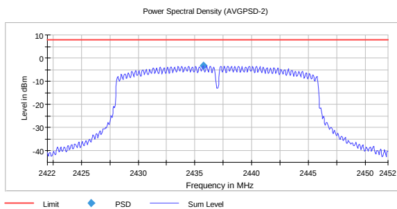
PSD, 2437 MHz, 802.11n MIMO MCS8 -3.24
