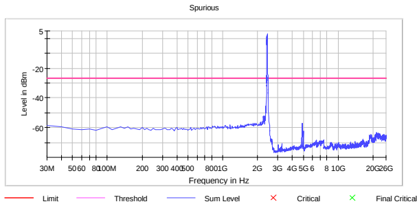
Conducted Emissions Ch06 802.11n HT40 MCS0 SISO
