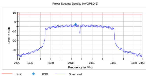
PSD, 2437 MHz, 802.11g 6M -3.05
