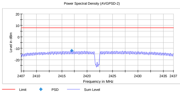
PSD, 2422 MHz, 802.11n HT40 MIMO MCS8 -12.1
