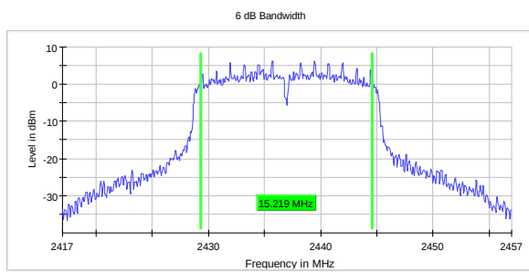
DTS BW, 2437 MHz, 802.11g 6M
