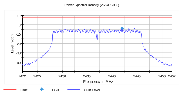
PSD, 2437 MHz, 802.11n MIMO MCS15 -3.69
