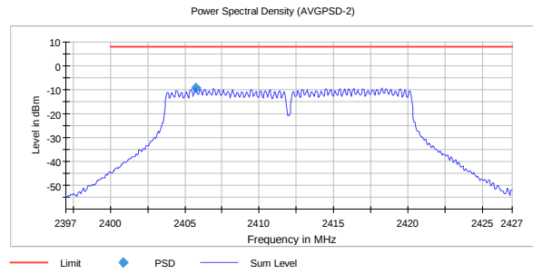
PSD, 2412 MHz, 802.11g 54M -9.33
