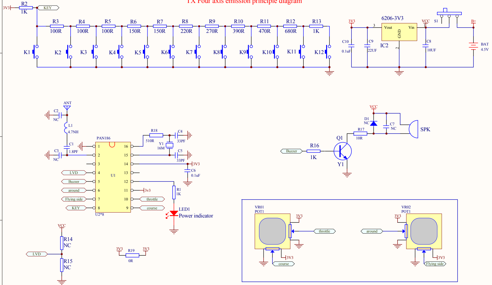
TX Four axis emission principle diagram
