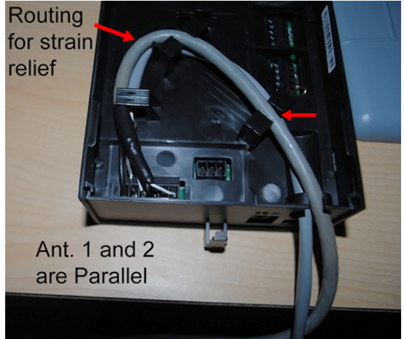
Figure 2: Antenna Wiring, Primary Connection (Cable Routing on right)
