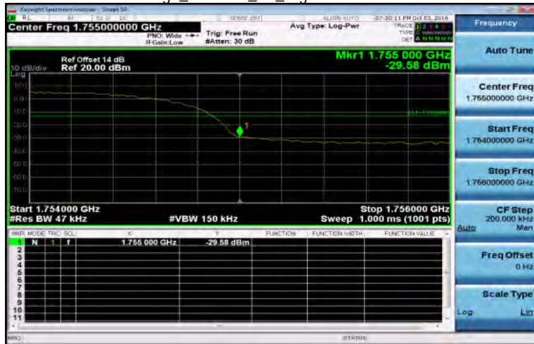
Band Edge_WCDMA_B4_HighCH1513-1752.6
