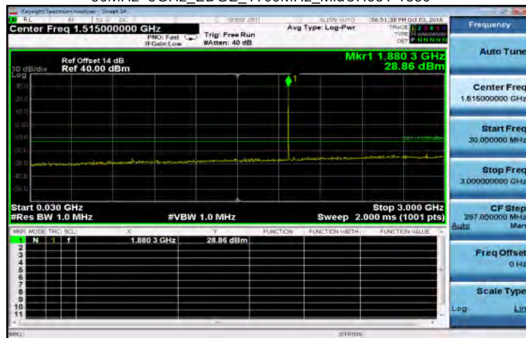
30MHz~3GHz_EDGE_1900MHz_MidCH661-1880
