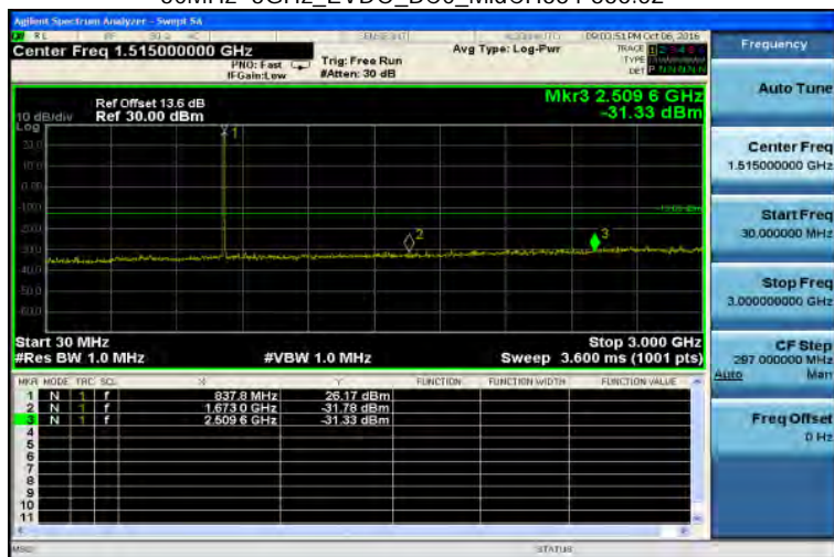
30MHz~3GHz_EVDO_BC0_MidCH384-836.52
