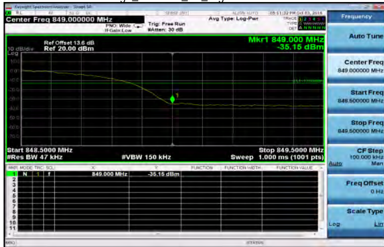
Band Edge_WCDMA_B5_HighCH4233-846.6
