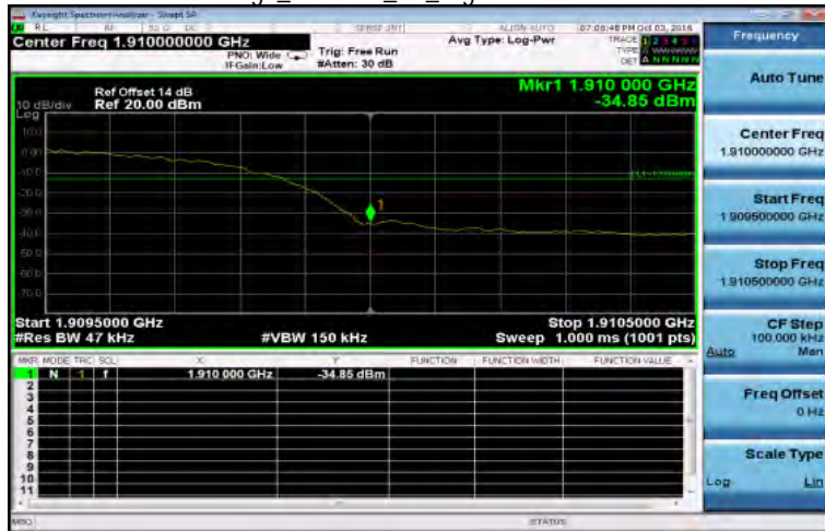
Band Edge_WCDMA_B2_HighCH9538-1907.6
