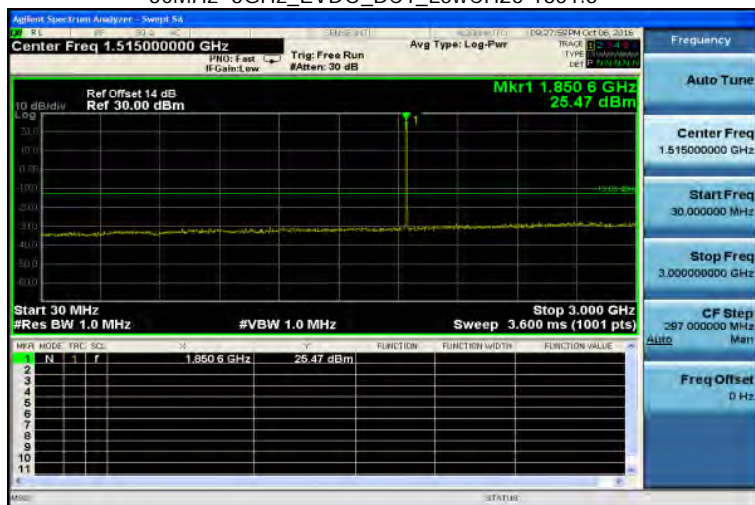
30MHz~3GHz_EVDO_BC1_LowCH25-1851.3
