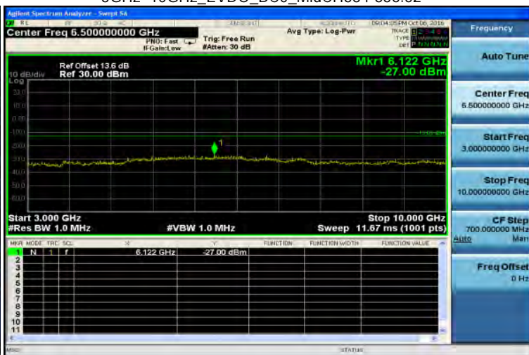
3GHz~10GHz_EVDO_BC0_MidCH384-836.52
