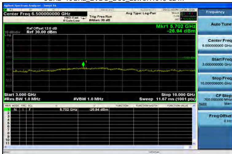
3GHz~10GHz_EVDO_BC0_LowCH1013-824.7
