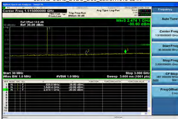
30MHz~3GHz_EVDO_BC0_LowCH1013-824.7
