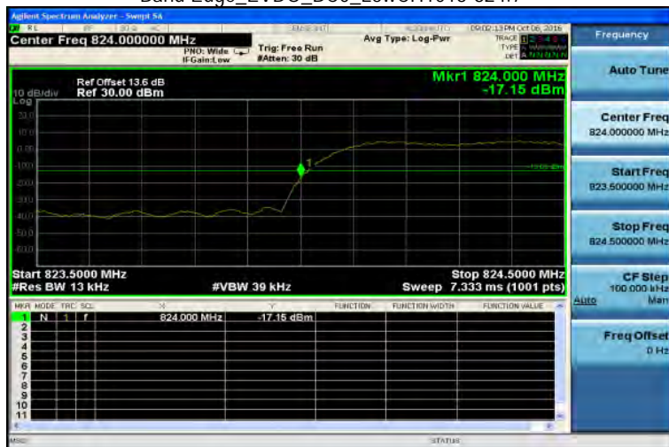
Band Edge_EVDO_BC0_LowCH1013-824.7
