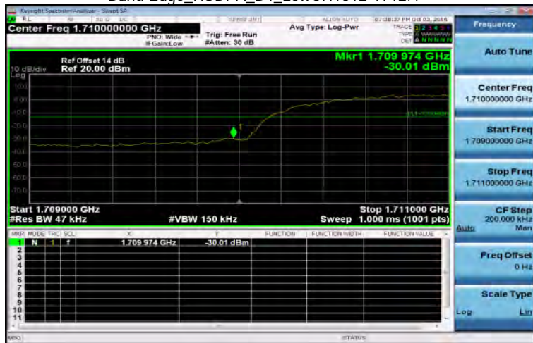
Band Edge_HSDPA_B4_LowCH1312-1712.4
