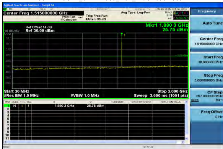
30MHz~3GHz_CDMA2000_BC1_MidCH600-1880
