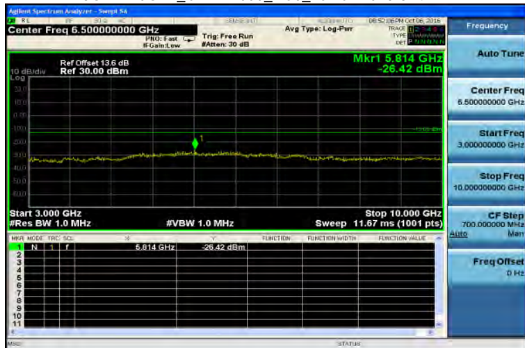
3GHz-10GHz_CDMA2000_BC0_LowCH1013-824.7
