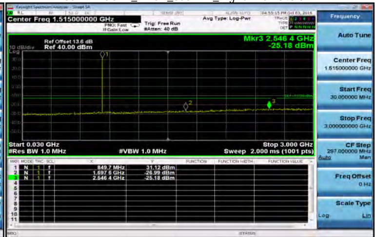
30MHz-3GHz_EDGE_850MHz_HighCH251-848.8
