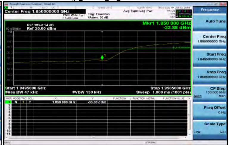
Band Edge_HSUPA_B2_LowCH9262-1852.4
