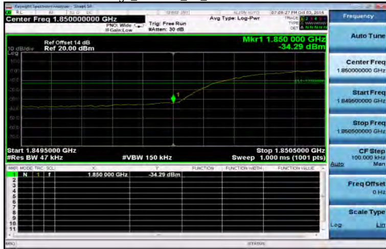
Band Edge_WCDMA_B2_LowCH9262-1852.4
