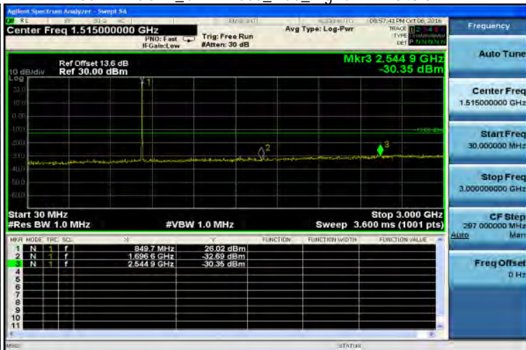
30MHz-3GHz_CDMA2000_BC0_HighCH777-848.31
