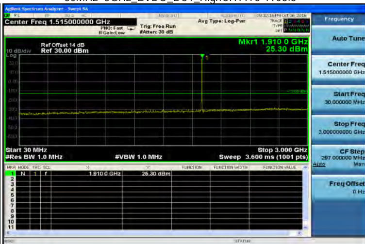
30MHz~3GHz_EVDO_BC1_HighCH1175-1908.8
