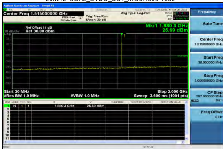
30MHz~3GHz_EVDO_BC1_MidCH600-1880
