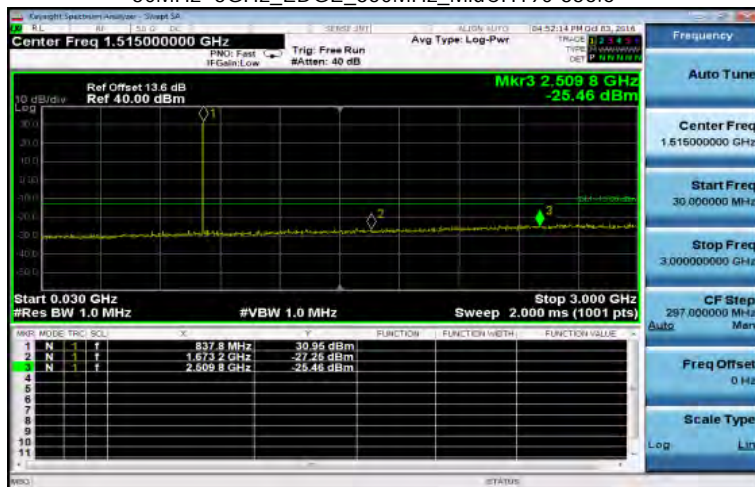
30MHz-3GHz_EDGE_850MHz_MidCH190-836.6
