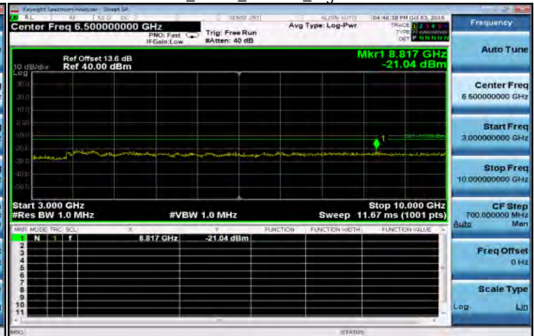
3GHz-10GHz_GPRS_850MHz_HighCH251-848.8
