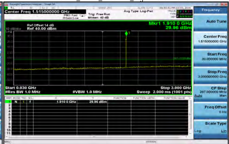
30MHz~3GHz_EDGE_1900MHz_HighCH810-1909.8
