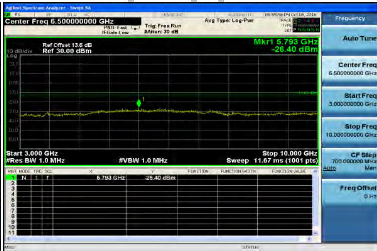
3GHz-10GHz_CDMA2000_BC0_MidCH384-836.52
