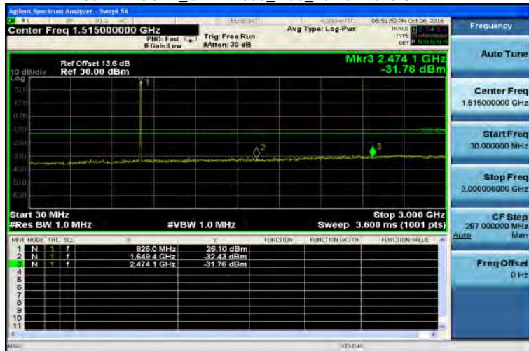
30MHz-3GHz_CDMA2000_BC0_LowCH1013-824.7
