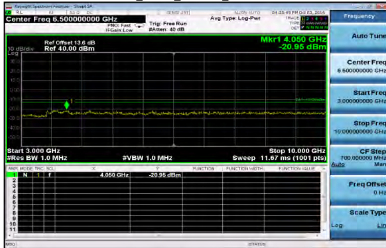
3GHz-10GHz_GPRS_850MHz_LowCH128-824.2
