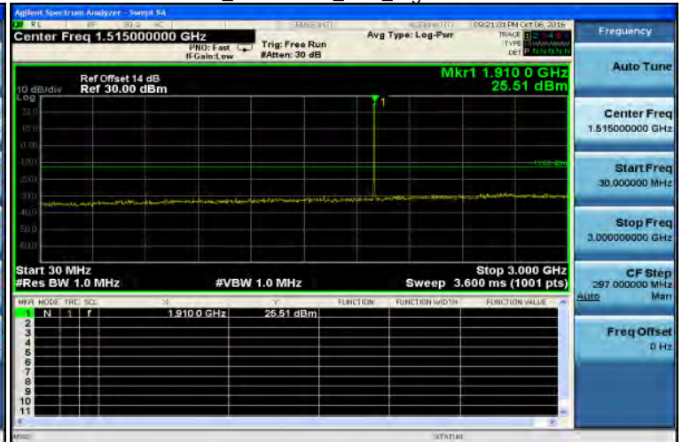
30MHz~3GHz_CDMA2000_BC1_HighCH1175-1908.8
