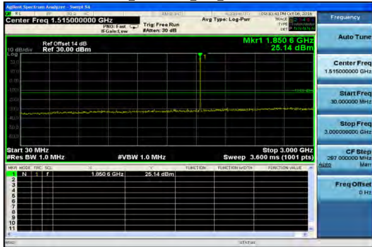
30MHz~3GHz_CDMA2000_BC1_LowCH25-1851.3
