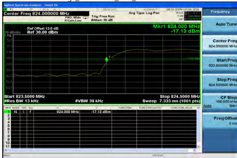
Band Edge_CDMA2000_BC0_LowCH1013-824.7
