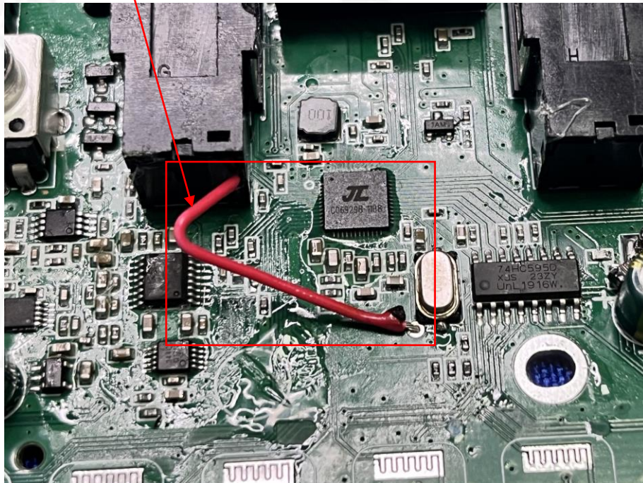
BT/BLE Antenna
