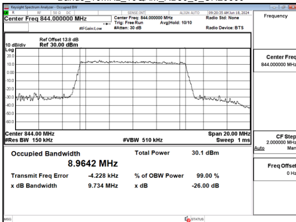
Band5_10MHz_16QAM_RB50_0_CH20600
