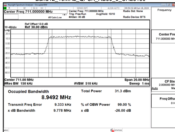
Band12_10MHz_QPSK_RB50_0_CH23130
