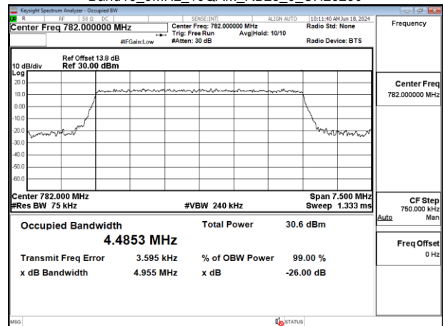
Band13_5MHz_16QAM_RB25_0_CH23255
