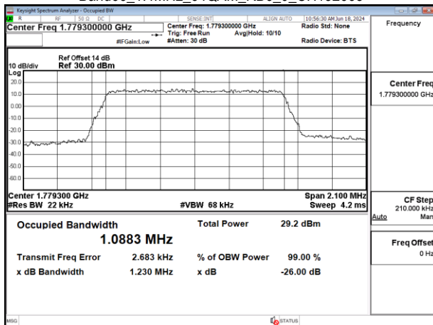
Band66_1.4MHz_64QAM_RB6_0_CH132665
