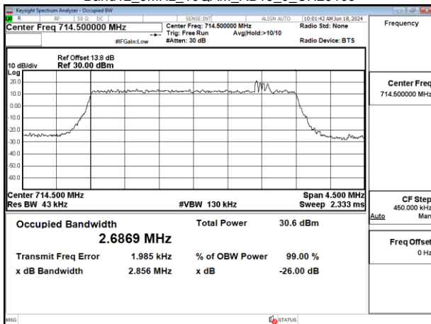
Band12_3MHz_16QAM_RB15_0_CH23165
