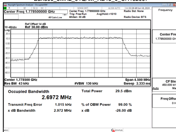
Band66_3MHz_64QAM_RB15_0_CH132657
