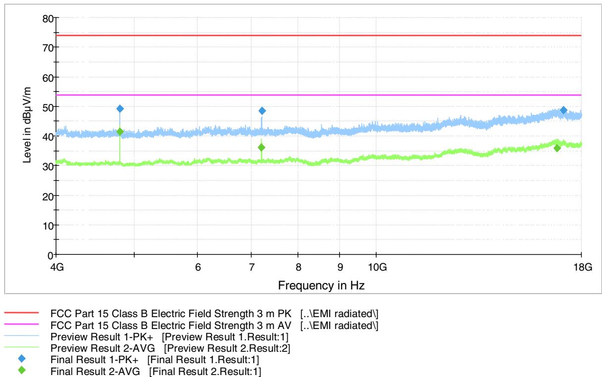
Figure 24: Low channel 4 GHz – 18 GHz
