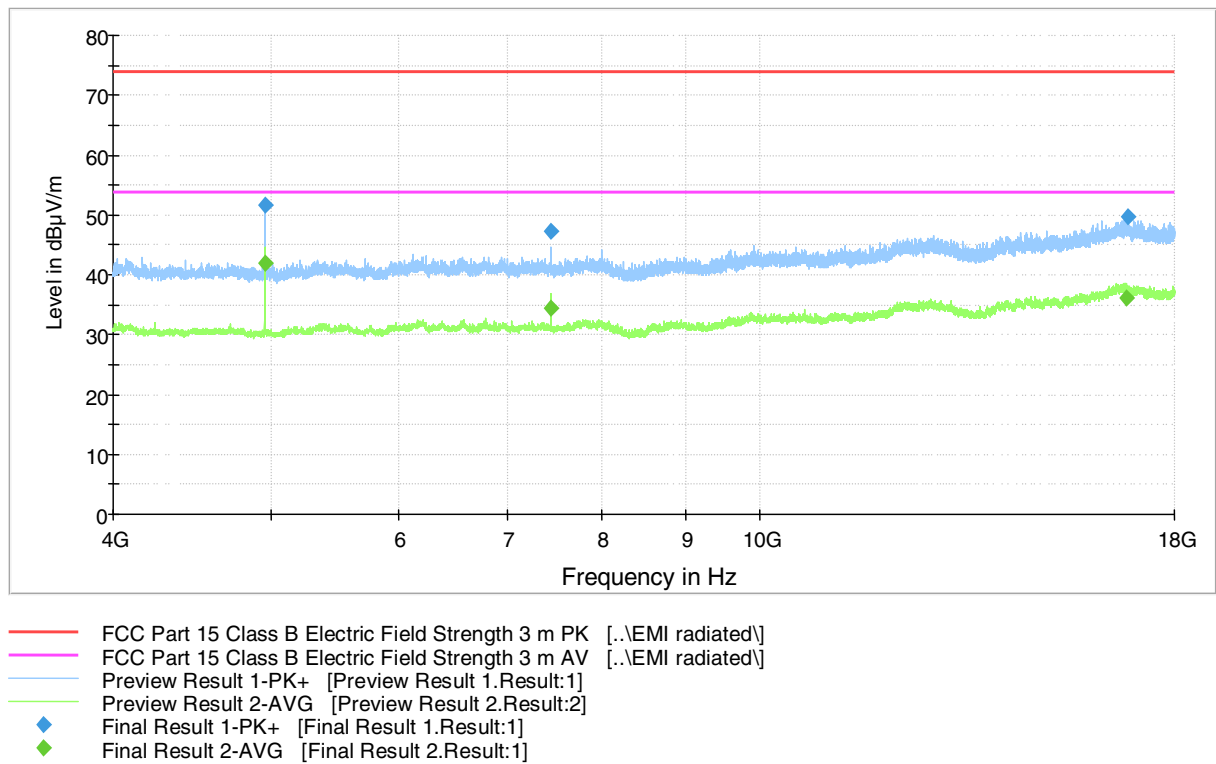
Figure 32: High channel 4 GHz – 18 GHz
