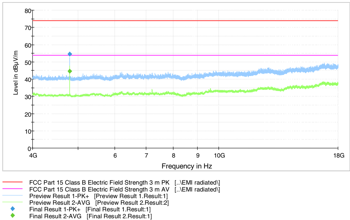
Figure 10: Low channel 4 GHz – 18 GHz
