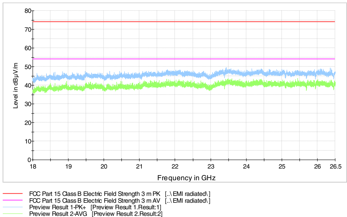
Figure 11: Low channel 18 GHz – 26.5 GHz
