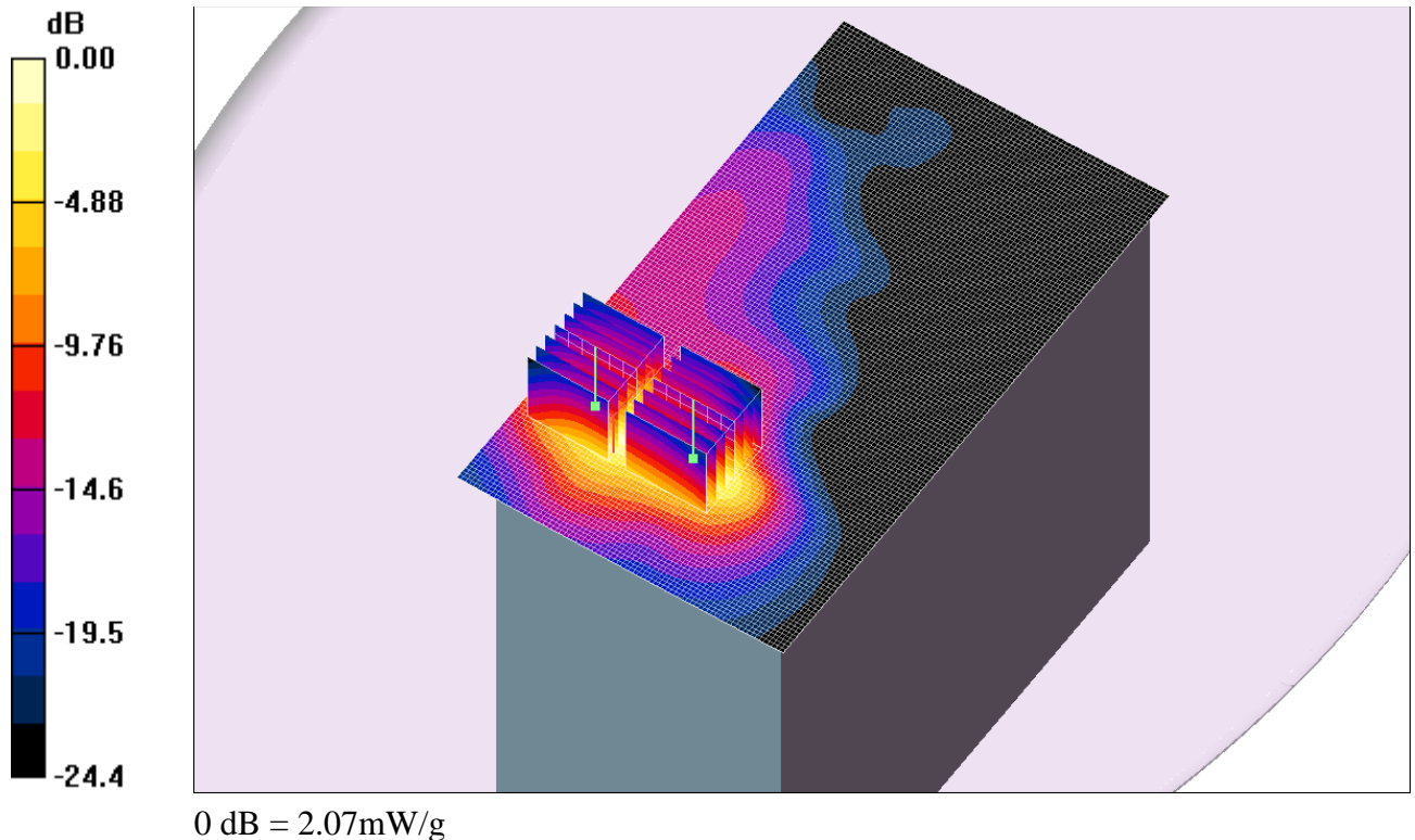
Fig. 1: SAR distribution for 802.11b at 11Mbps: channel 11 (2462 MHz), front side at 0cm
