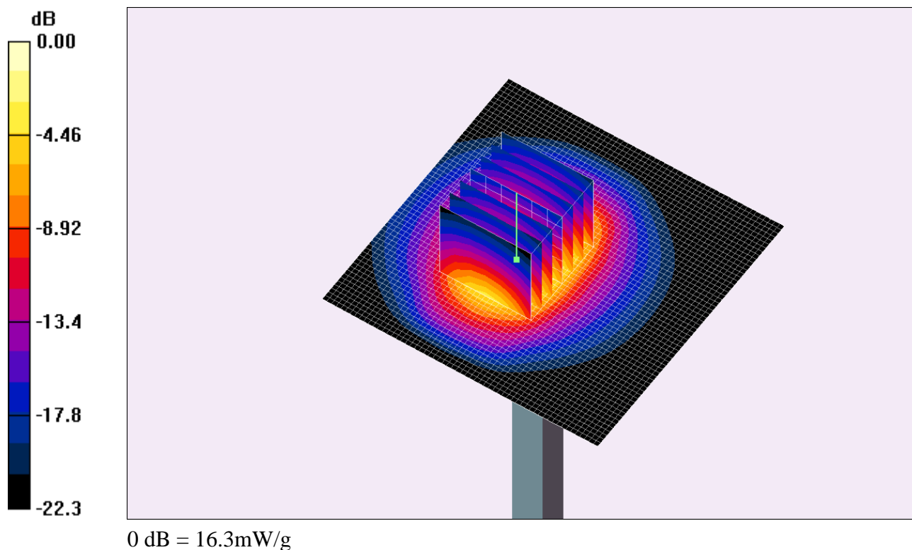
Fig. 5: 2450MHz system check result
