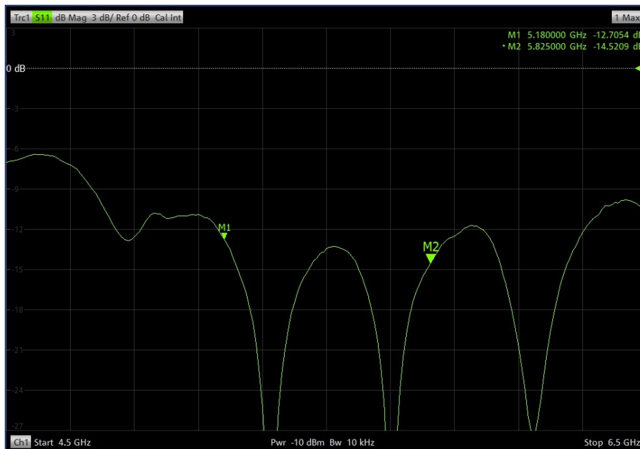
Antenna 4 (5 GHz / ch1)
