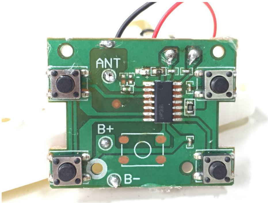
Internal View
