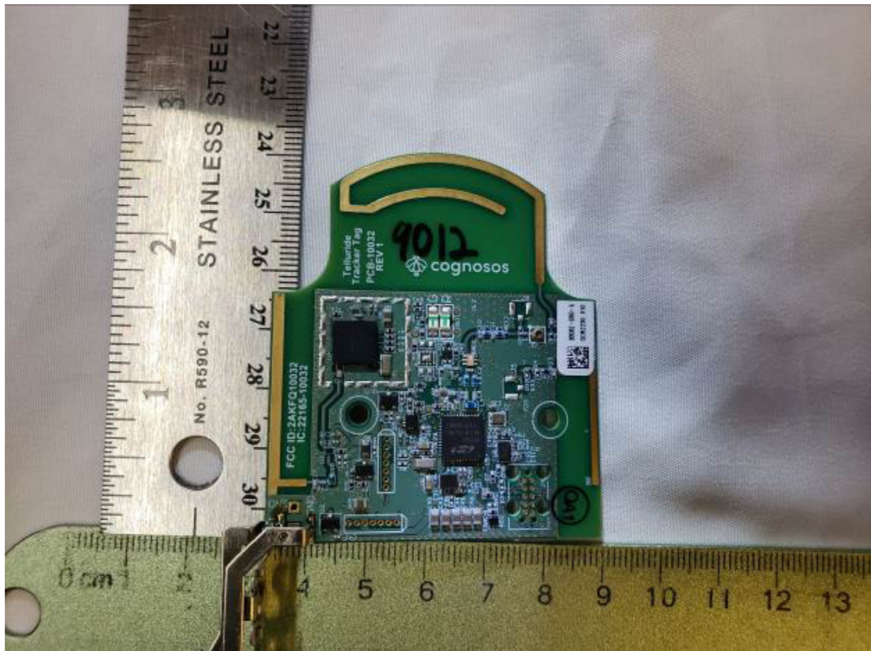
Figure 7. Radio Module External Top View
