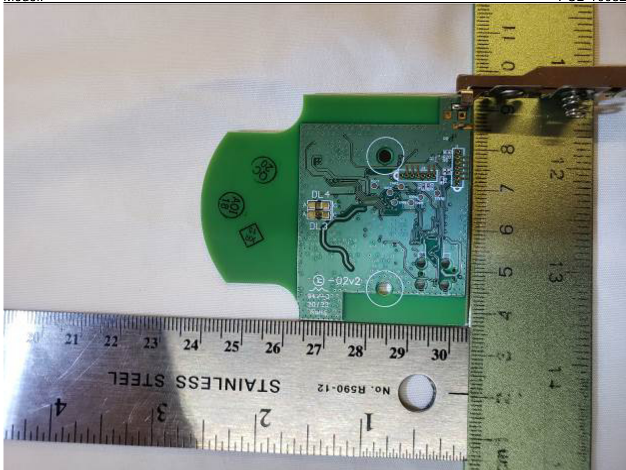
Figure 8. Radio Module External Bottom View
