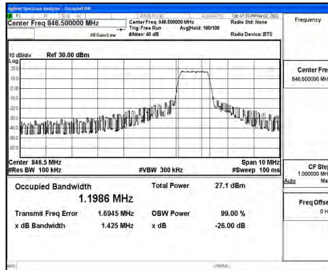
Band26-5MHz-QPSK-27015-6-0-High-1.1986-1.425-PASS
