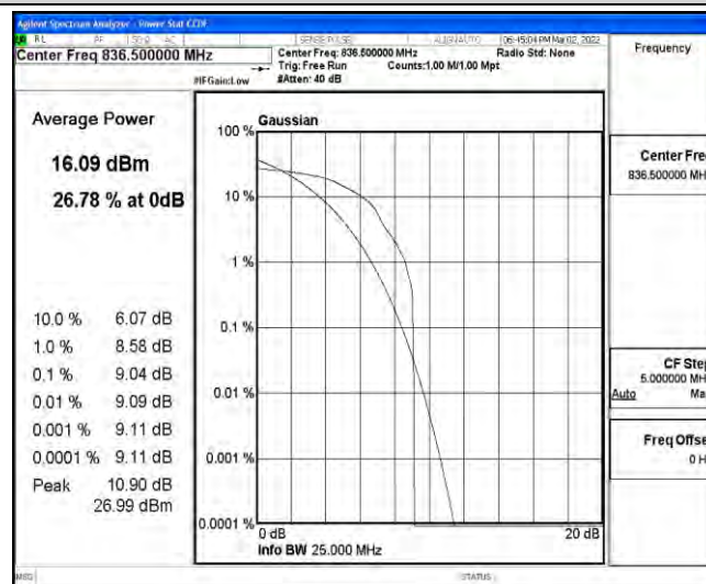
Band26-5MHz-16QAM-26915-1-0-Low-9.04-=<13-PASS
