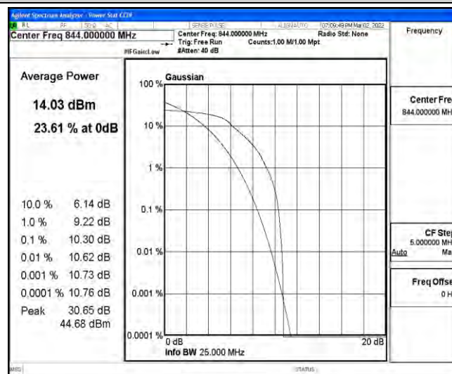
Band26-10MHz-QPSK-26990-6-0-High-10.30-<=13-PASS
