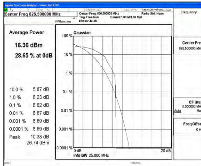
Band26-5MHz-16QAM-26815-1-0-Low-8.62-=<13-PASS
