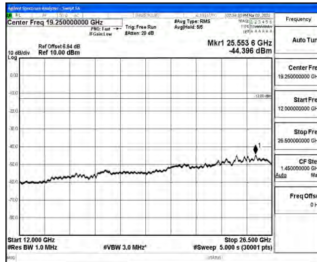
Band26-10MHz-16QAM-26840-1-0-Low-12000-26500--44.4-PASS
