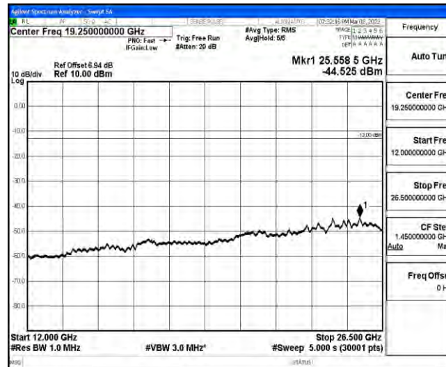
Band26-10MHz-QPSK-26840-1-0-Low-12000-26500--44.53-PASS
