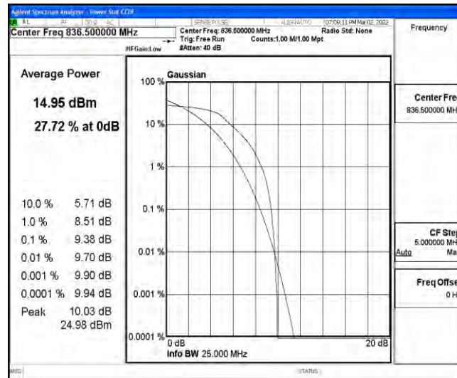
Band26-10MHz-QPSK-26915-6-0-Low-9.38-<=13-PASS
