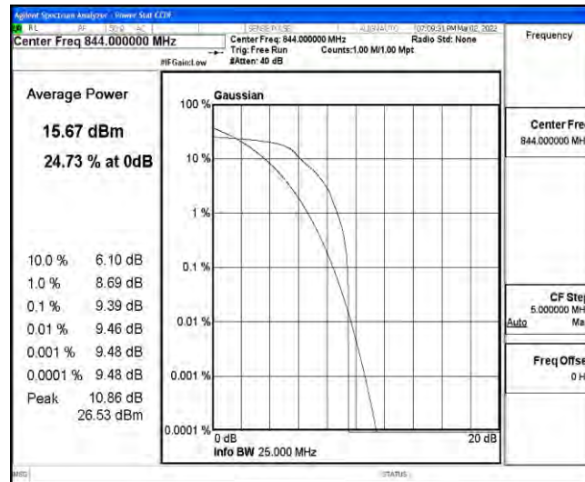
Band26-10MHz-QPSK-26990-1-0-High-9.39-<=13-PASS
