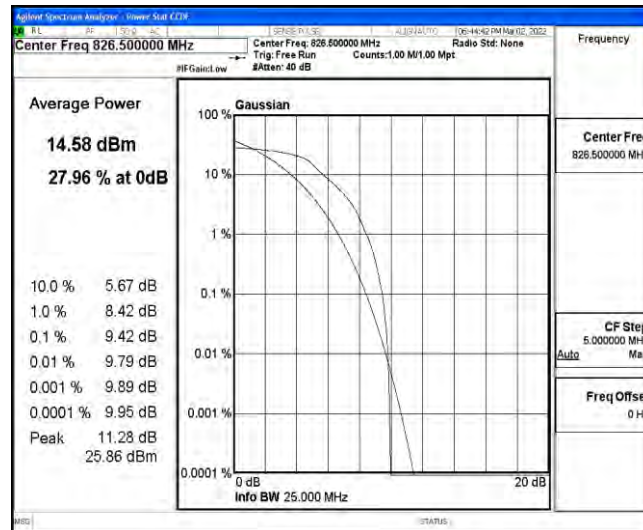
Band26-5MHz-16QAM-26815-6-0-Low-9.42-=<13-PASS
