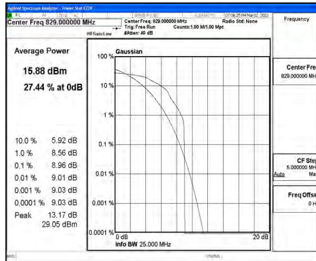
Band26-10MHz-16QAM-26840-1-0-Low-8.96-<=13-PASS
