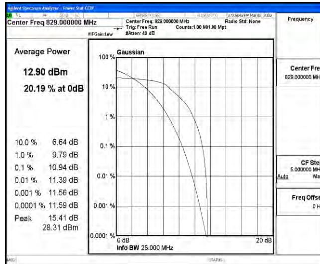
Band26-10MHz-16QAM-26840-6-0-Low-10.94-<=13-PASS
