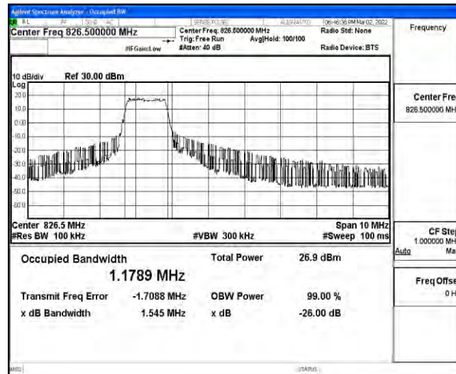
Band26-5MHz-16QAM-26815-6-0-Low-1.1789-1.545-PASS
