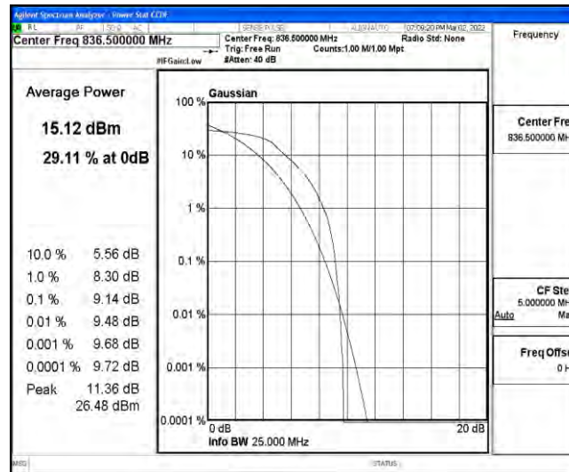
Band26-10MHz-16QAM-26915-6-0-Low-9.14-<=13-PASS
