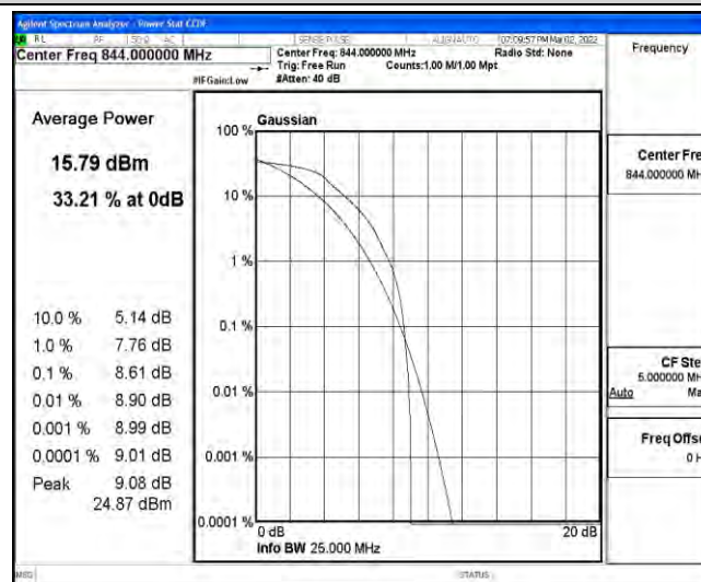
Band26-10MHz-16QAM-26990-6-0-High-8.61-<=13-PASS
