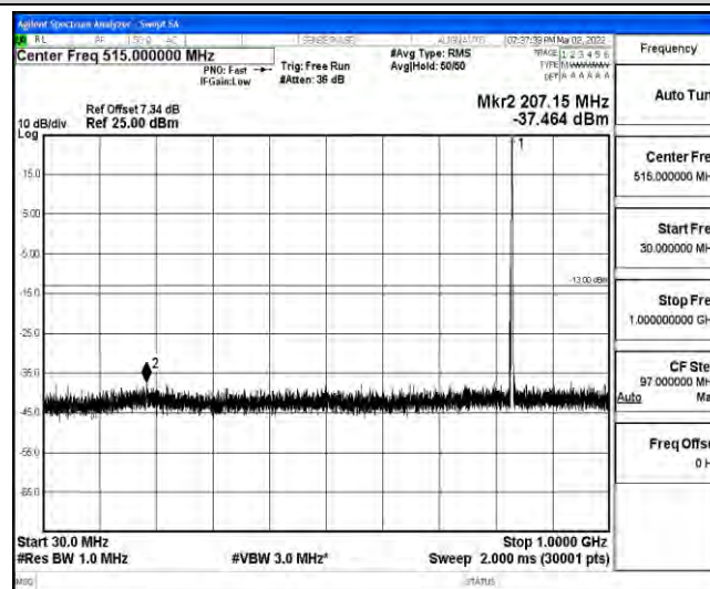
Band26-10MHz-16QAM-26915-1-0-Low-30-1000--37.46-PASS
