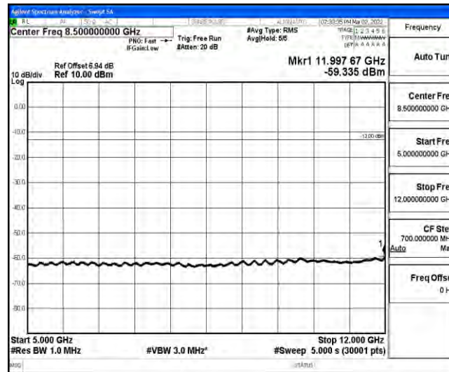
Band26-10MHz-16QAM-26840-1-0-Low-5000-12000--59.34-PASS
