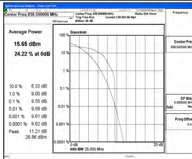
Band26-10MHz-16QAM-26915-1-0-Low-9.55-<=13-PASS
