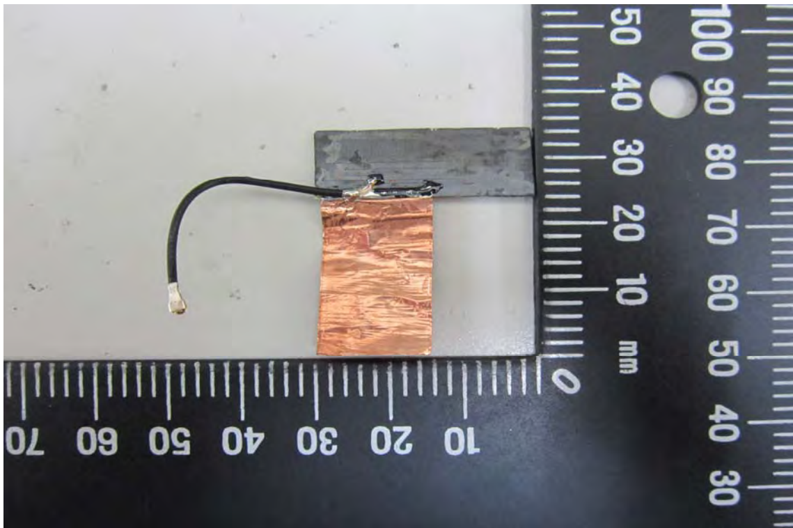
Antenna Main - 1
