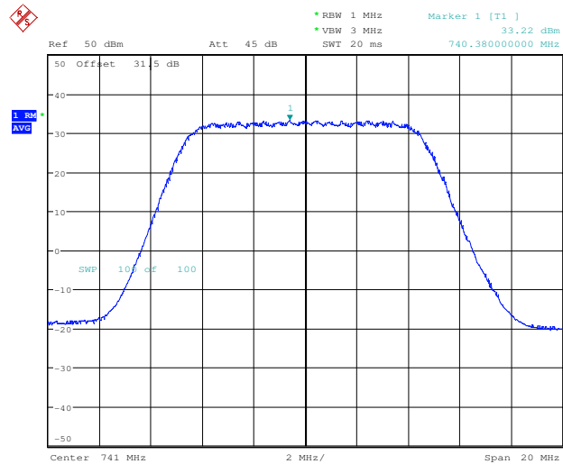
Plot 7.2.24 Maximum output power test results at high frequency, 64QAM modulation RF Output #2, 10 MHz
