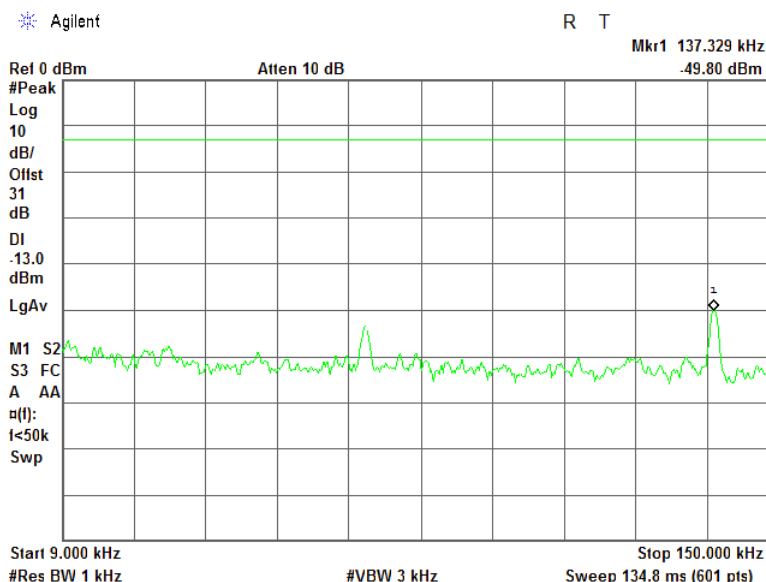
Plot 7.4.14 Spurious emission measurements in 9 - 150 kHz range at mid carrier frequency, RF# 2
