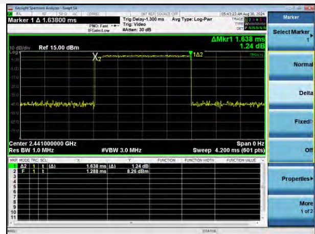
8-DPSK 3DH1
