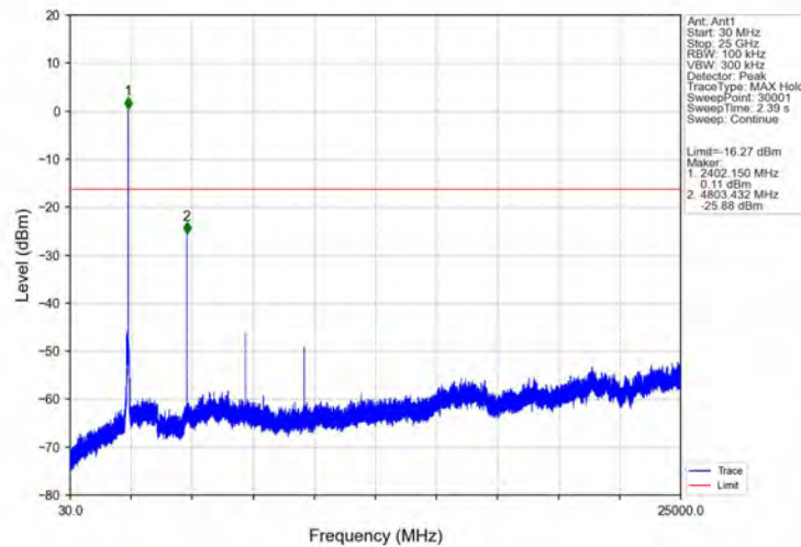
8DPSK_3DH5_LCH_2402MHz_Ant1_NTNV
