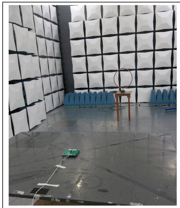
Loop Antenna
