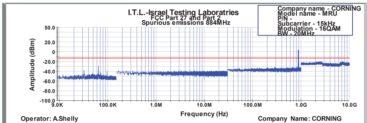
Figure 538: Spurious Emissions at Antenna Terminal 16QAM 20MHz B.W.; 884.0MHz, 15kHz
