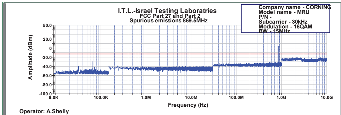
Figure 530: Spurious Emissions at Antenna Terminal 16QAM 15MHz B.W.; 869.5MHz, 30kHz
