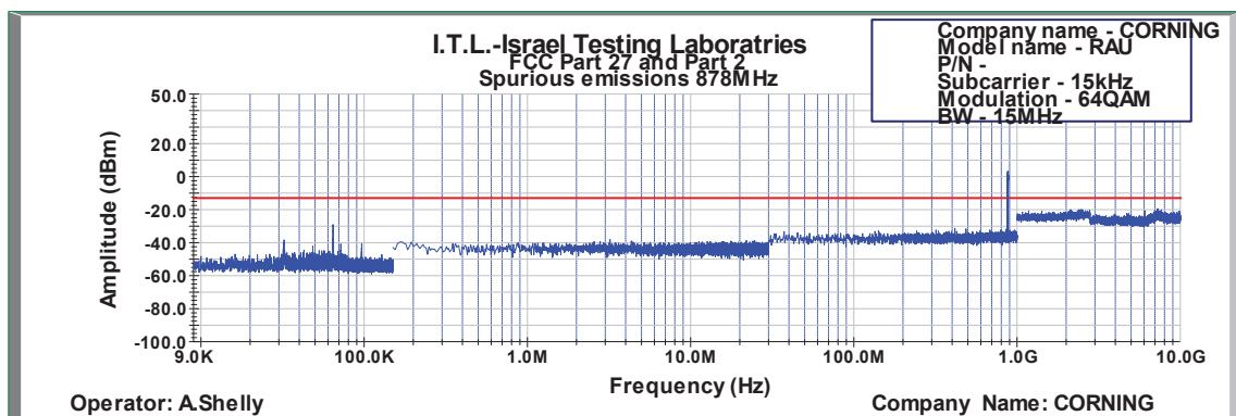
Figure 570: Spurious Emissions at Antenna Terminal 64QAM 15MHz B.W.; 878.0MHz, 15kHz
