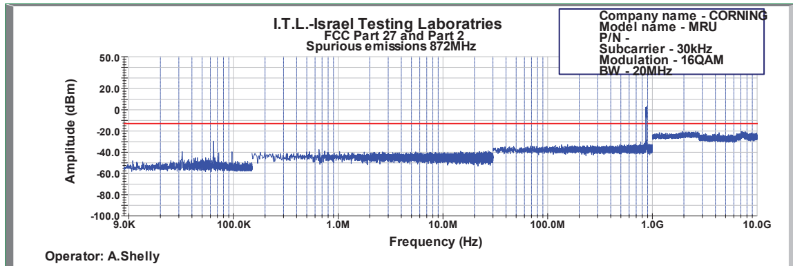
Figure 539: Spurious Emissions at Antenna Terminal 16QAM 20MHz B.W.; 872.0MHz, 30kHz
