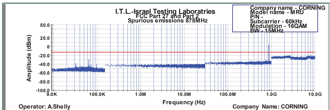
Figure 534: Spurious Emissions at Antenna Terminal 16QAM 15MHz B.W.; 878.0MHz, 60kHz
