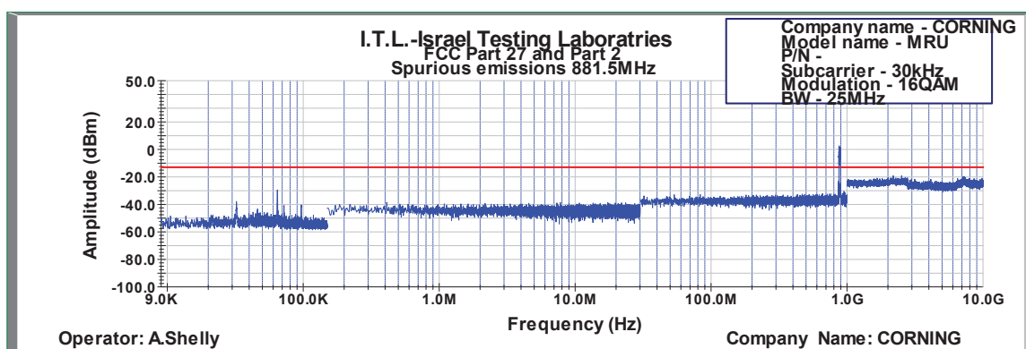
Figure 550: Spurious Emissions at Antenna Terminal 16QAM 25MHz B.W.; 881.5MHz, 30kHz
