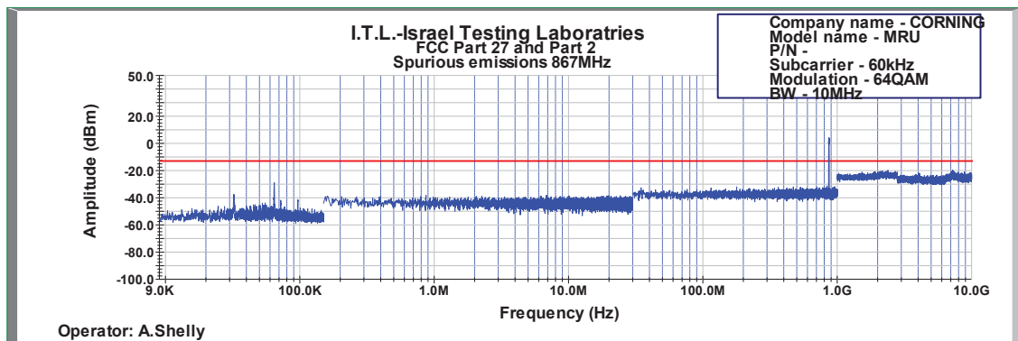
Figure 566: Spurious Emissions at Antenna Terminal 64QAM 10MHz B.W.; 867.0MHz, 60kHz
