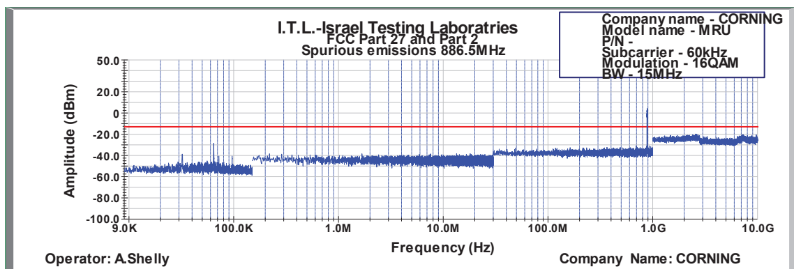
Figure 535: Spurious Emissions at Antenna Terminal 16QAM 15MHz B.W.; 886.5MHz, 60kHz
