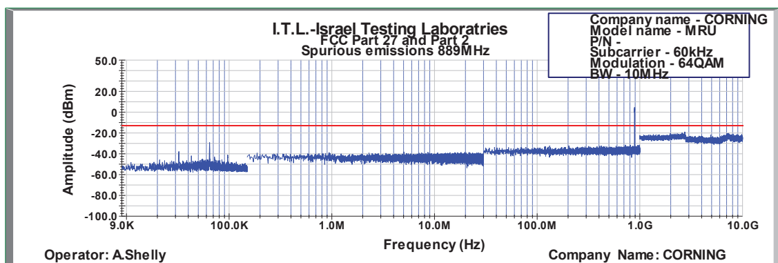
Figure 568: Spurious Emissions at Antenna Terminal 64QAM 10MHz B.W.; 889.0MHz, 60kHz
