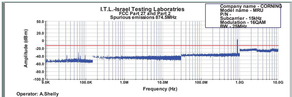
Figure 545: Spurious Emissions at Antenna Terminal 16QAM 25MHz B.W.; 874.5MHz, 15kHz
