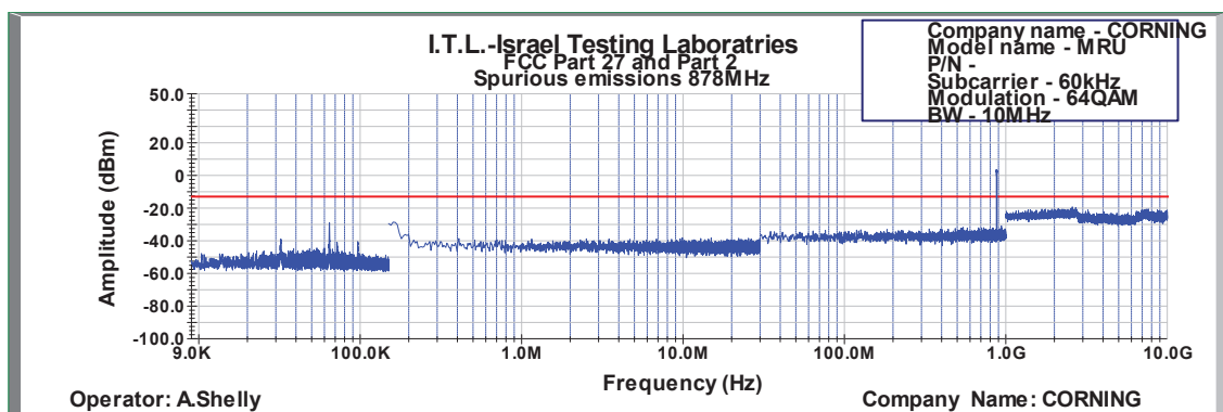
Figure 567: Spurious Emissions at Antenna Terminal 64QAM 10MHz B.W.; 878.0MHz, 60kHz
