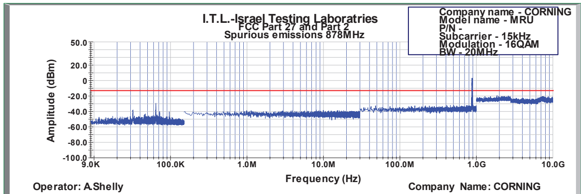
Figure 537: Spurious Emissions at Antenna Terminal 16QAM 20MHz B.W.; 878.0MHz, 15kHz
