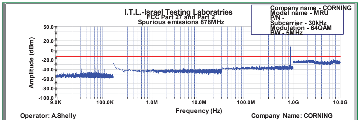
Figure 558: Spurious Emissions at Antenna Terminal 64QAM 5MHz B.W.; 878.0MHz, 30kHz
