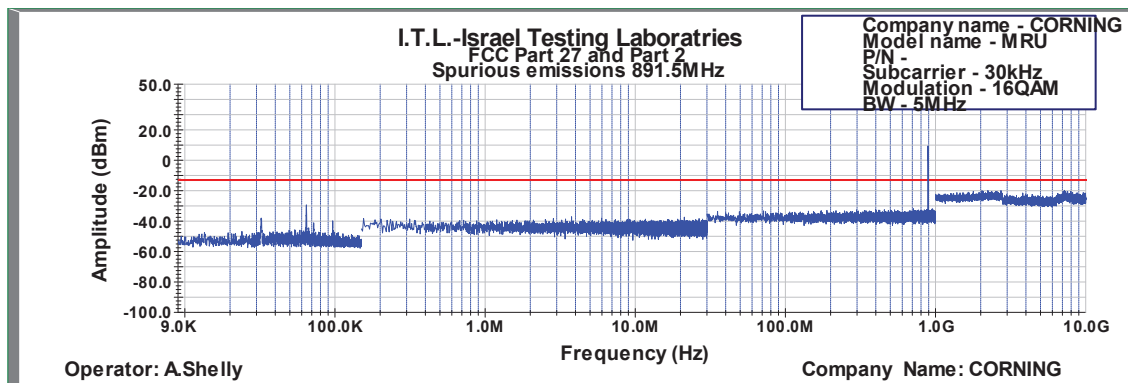
Figure 517: Spurious Emissions at Antenna Terminal 16QAM 5MHz; 891.5MHz, 30kHz
