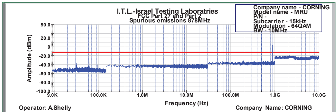
Figure 561: Spurious Emissions at Antenna Terminal 64QAM 10MHz B.W.; 878.0MHz, 15kHz
