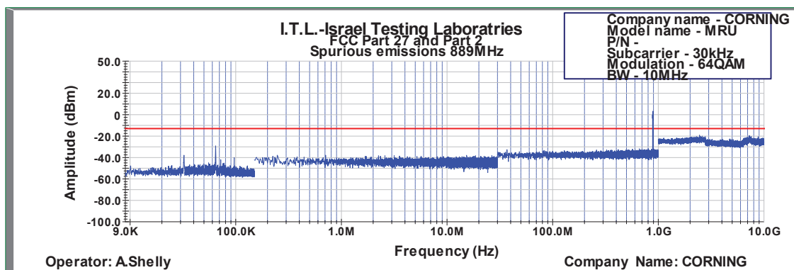
Figure 565: Spurious Emissions at Antenna Terminal 64QAM 10MHz B.W.; 889.0MHz, 30kHz
