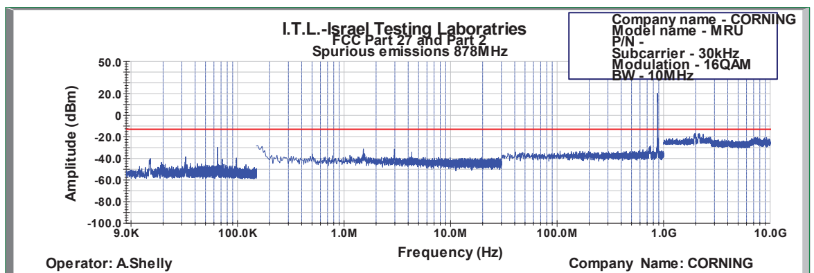
Figure 522: Spurious Emissions at Antenna Terminal 16QAM 10MHz B.W.; 878.0MHz, 30kHz
