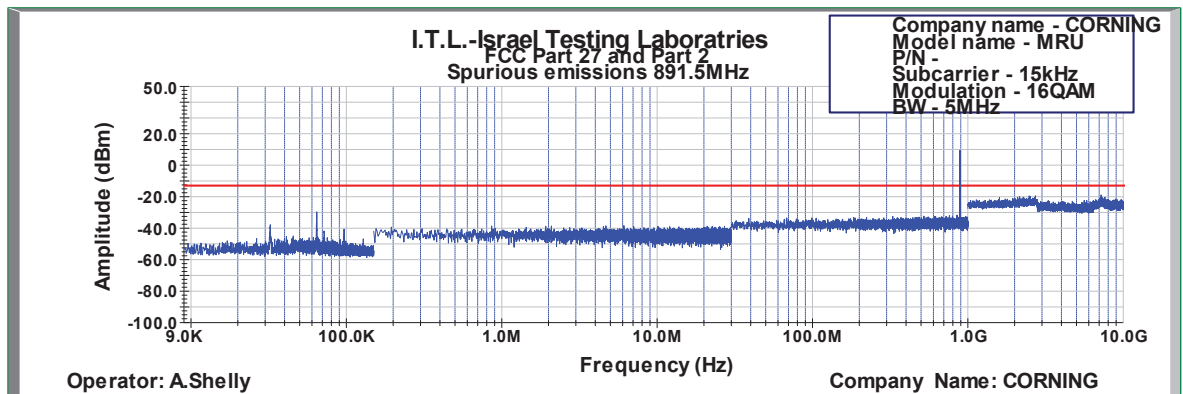
Figure 514: Spurious Emissions at Antenna Terminal 16QAM 5MHz B.W.; 891.5MHz, 15kHz
