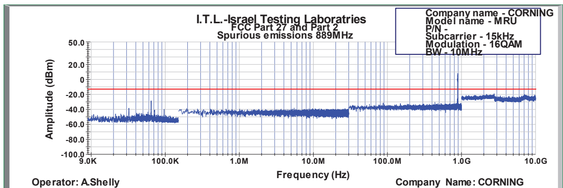
Figure 520: Spurious Emissions at Antenna Terminal 16QAM 10MHz B.W.; 889.0MHz, 15kHz
