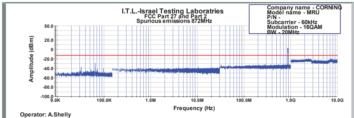
Figure 542: Spurious Emissions at Antenna Terminal 16QAM 20MHz B.W.; 872.0MHz, 60kHz
