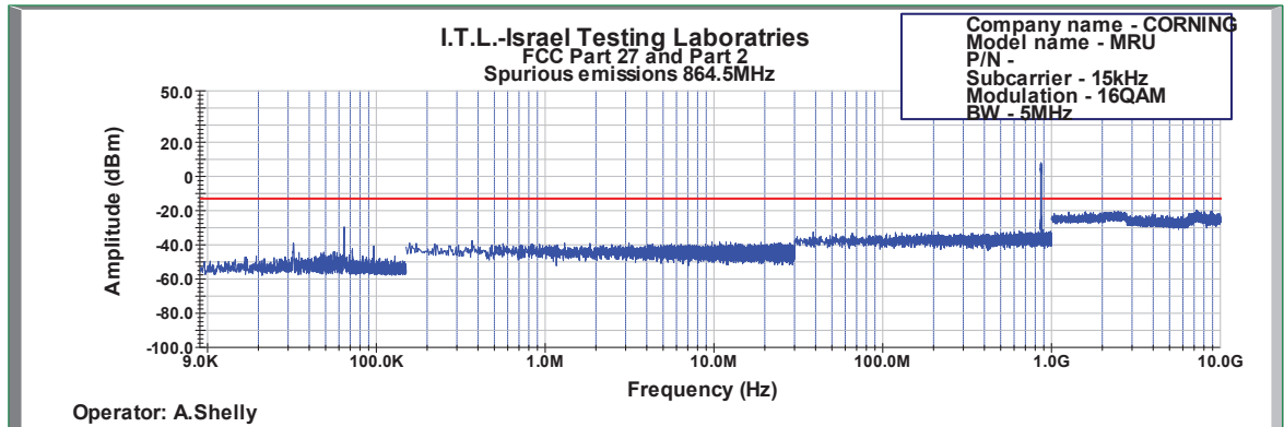
Figure 512: Spurious Emissions at Antenna Terminal 16QAM 5MHz B.W.; 864.5MHz, 15kHz
