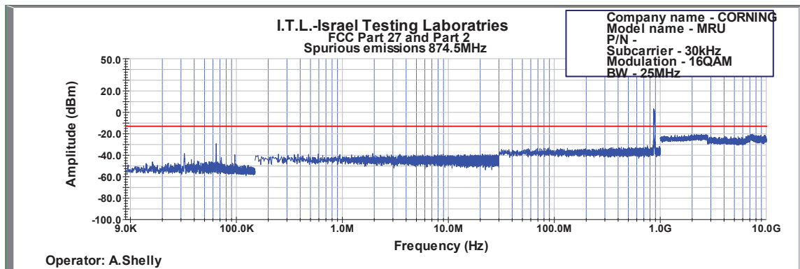
Figure 548: Spurious Emissions at Antenna Terminal 16QAM 25MHz B.W.; 874.5MHz, 30kHz
