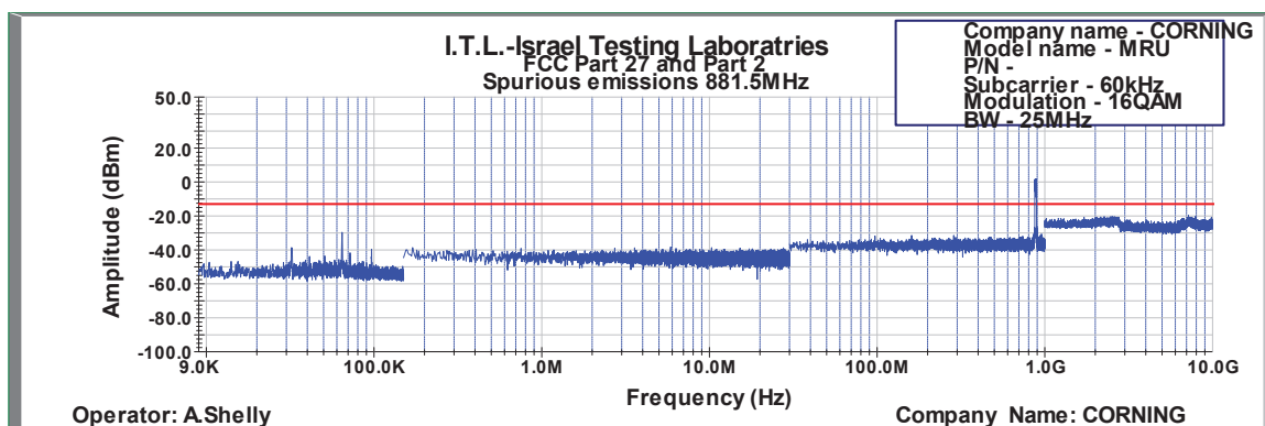
Figure 553: Spurious Emissions at Antenna Terminal 16QAM 25MHz B.W.; 881.5MHz, 60kHz
