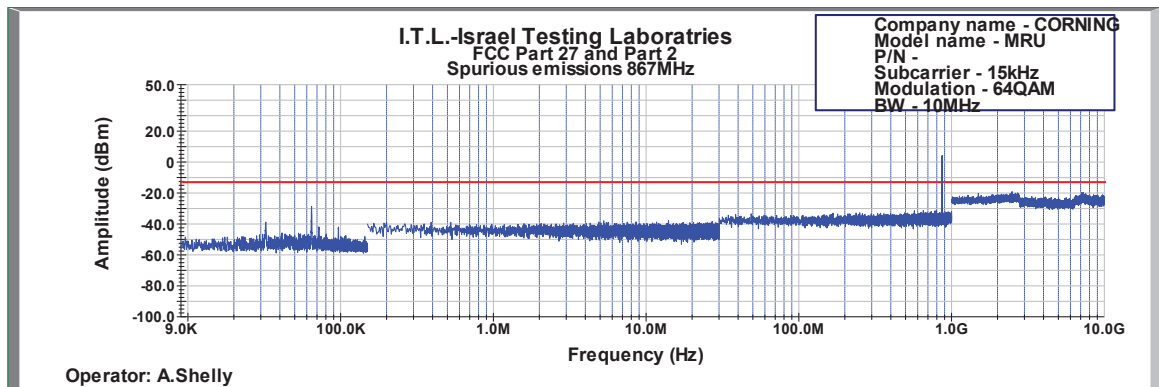
Figure 560: Spurious Emissions at Antenna Terminal 64QAM 10MHz B.W.; 867.0MHz, 15kHz
