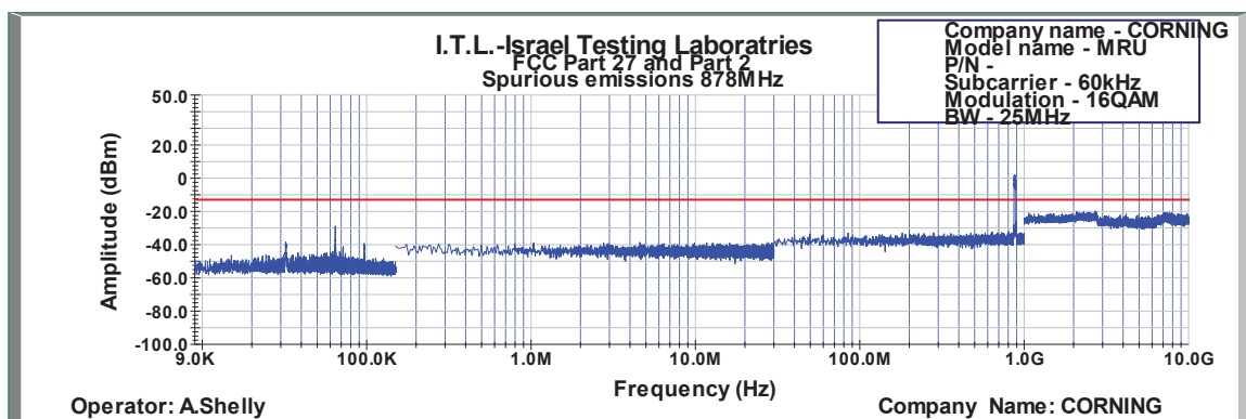
Figure 552: Spurious Emissions at Antenna Terminal 16QAM 25MHz B.W.; 878.0MHz, 60kHz
