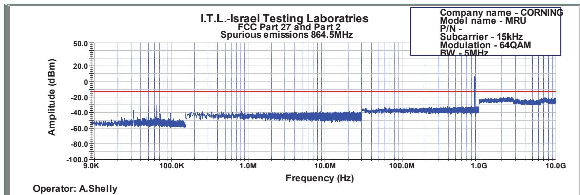
Figure 554: Spurious Emissions at Antenna Terminal 64QAM 5MHz B.W.; 864.5MHz, 15kHz
