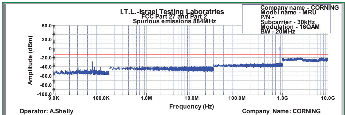
Figure 541: Spurious Emissions at Antenna Terminal 16QAM 20MHz B.W.; 884.0MHz, 30kHz
