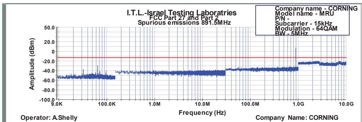
Figure 556: Spurious Emissions at Antenna Terminal 64QAM 5MHz B.W.; 891.5MHz, 15kHz
