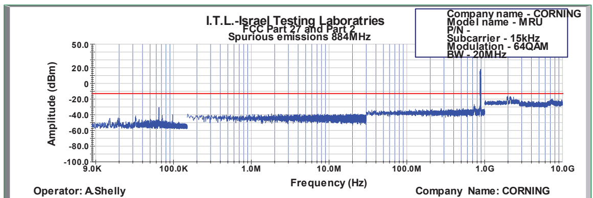
Figure 580: Spurious Emissions at Antenna Terminal 64QAM 20MHz B.W.; 884.0MHz, 15kHz
