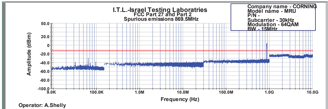
Figure 572: Spurious Emissions at Antenna Terminal 64QAM 15MHz B.W.; 869.5MHz, 30kHz
