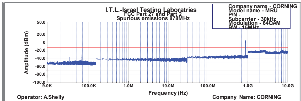
Figure 573: Spurious Emissions at Antenna Terminal 64QAM 15MHz B.W.; 878.0MHz, 30kHz
