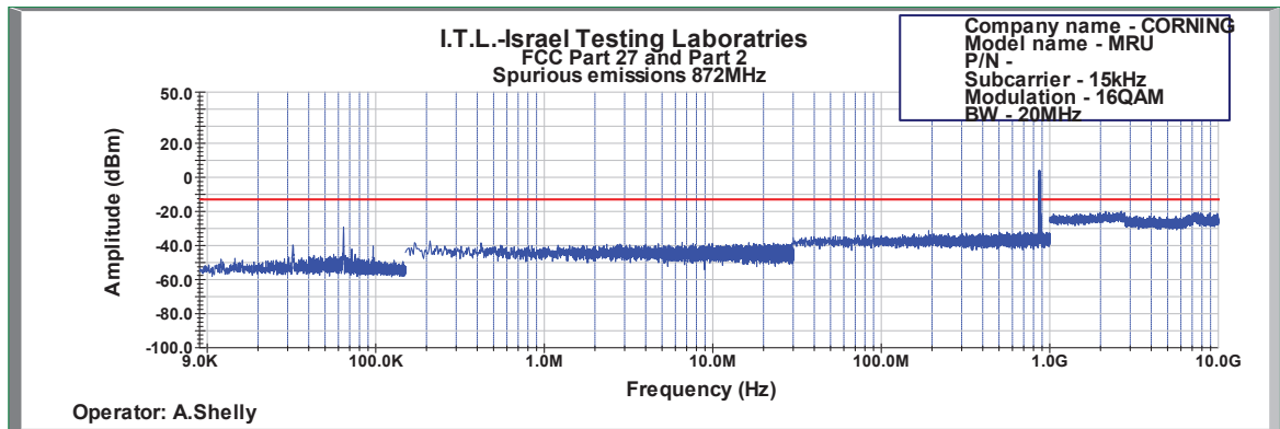
Figure 536: Spurious Emissions at Antenna Terminal 16QAM 20MHz B.W.; 872.0MHz, 15kHz
