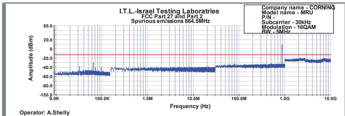
Figure 515: Spurious Emissions at Antenna Terminal 16QAM 5MHz B.W.; 864.5MHz, 30kHz
