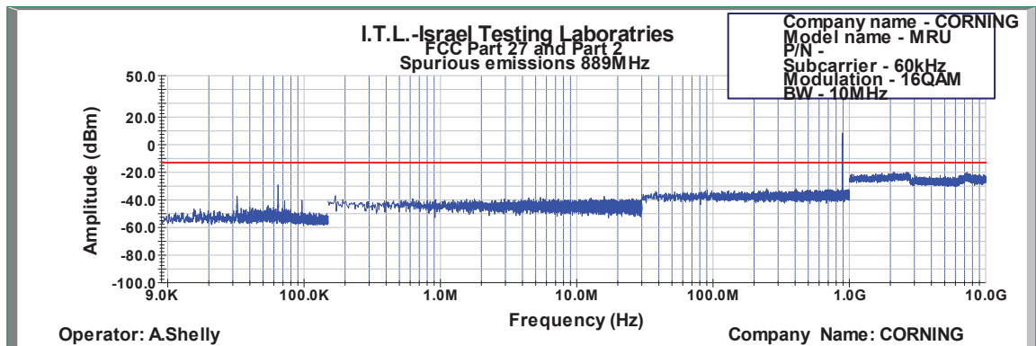
Figure 526: Spurious Emissions at Antenna Terminal 16QAM 10MHz B.W.; 889.0MHz, 60kHz
