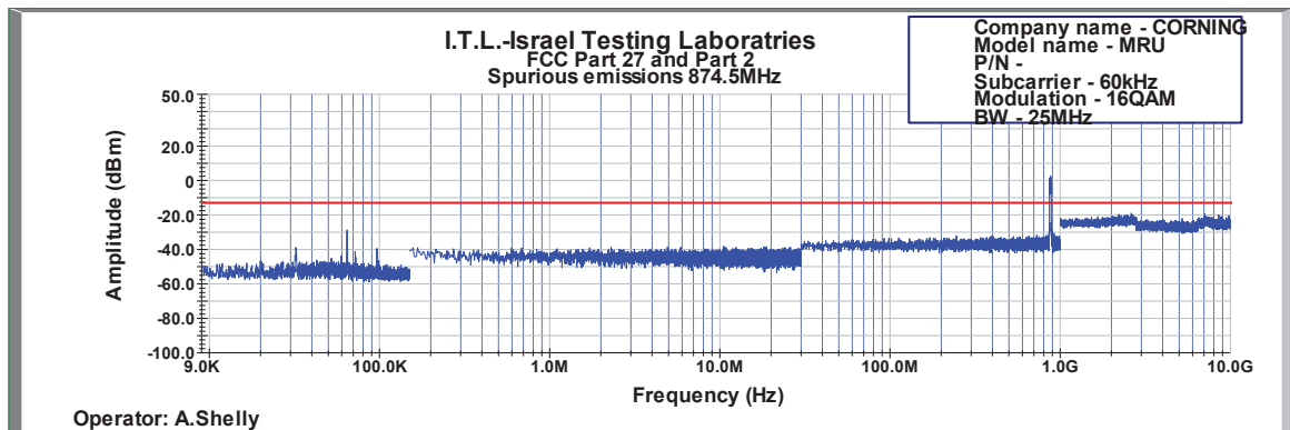
Figure 551: Spurious Emissions at Antenna Terminal 16QAM 25MHz B.W.; 874.5MHz, 60kHz
