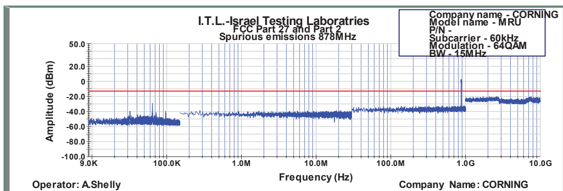
Figure 576: Spurious Emissions at Antenna Terminal 64QAM 15MHz B.W.; 878.0MHz, 60kHz
