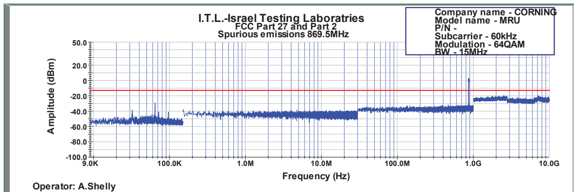
Figure 575: Spurious Emissions at Antenna Terminal 64QAM 15MHz B.W.; 869.5MHz, 60kHz
