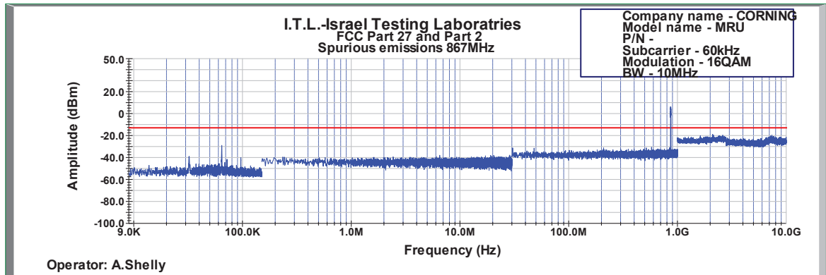
Figure 524: Spurious Emissions at Antenna Terminal 16QAM 10MHz B.W.; 867.0MHz, 60kHz
