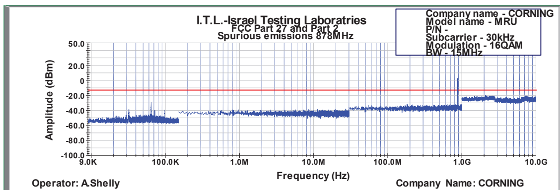
Figure 531: Spurious Emissions at Antenna Terminal 16QAM 15MHz B.W.; 878.0MHz, 30kHz
