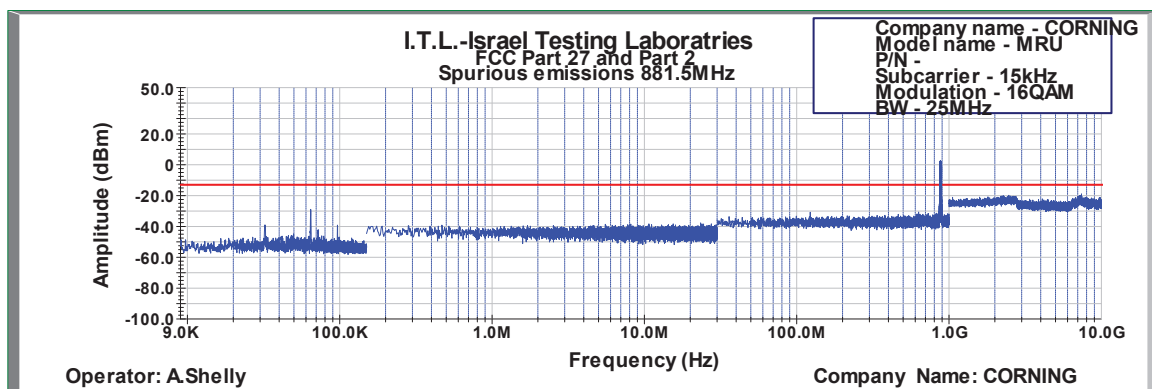
Figure 547: Spurious Emissions at Antenna Terminal 16QAM 25MHz B.W.; 881.5MHz, 15kHz
