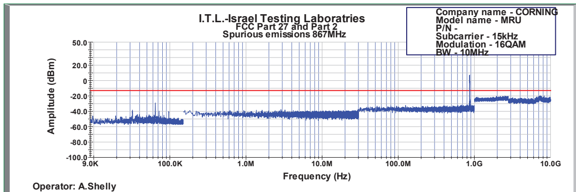
Figure 518: Spurious Emissions at Antenna Terminal 16QAM 10MHz B.W.; 867.0MHz, 15kHz
