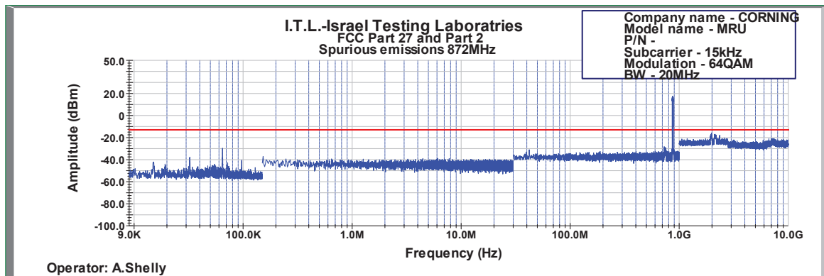
Figure 578: Spurious Emissions at Antenna Terminal 64QAM 20MHz B.W.; 872.0MHz, 15kHz
