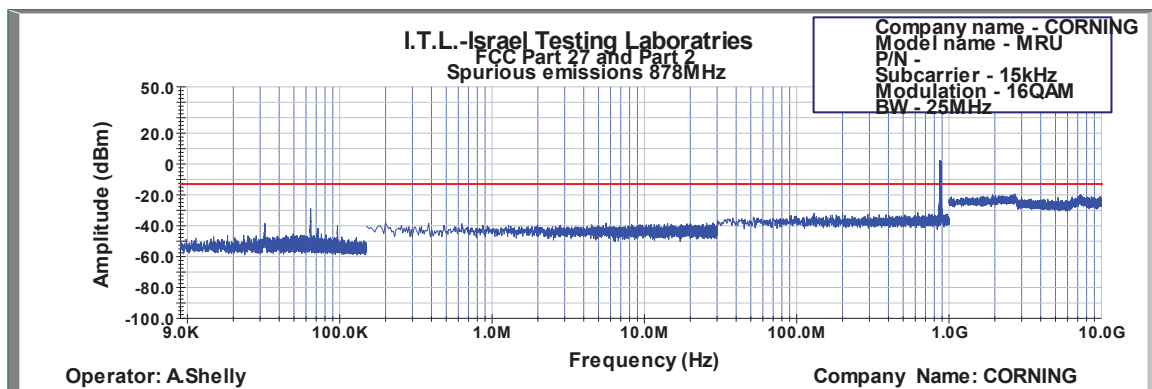
Figure 546: Spurious Emissions at Antenna Terminal 16QAM 25MHz B.W.; 878.5MHz, 15kHz
