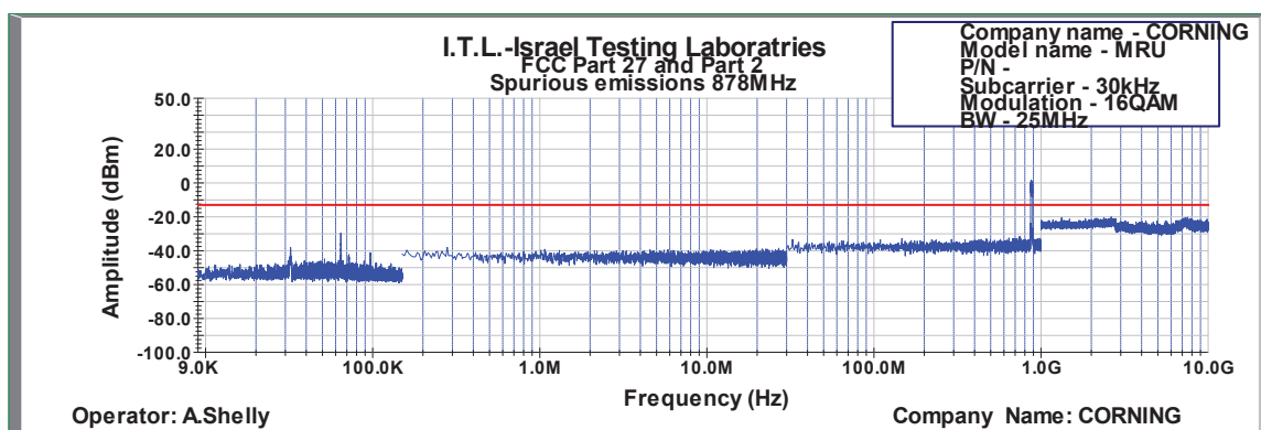
Figure 549: Spurious Emissions at Antenna Terminal 16QAM 25MHz B.W.; 878.0MHz, 30kHz
