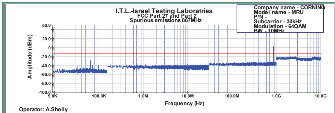
Figure 563: Spurious Emissions at Antenna Terminal 64QAM 10MHz B.W.; 867.0MHz, 30kHz
