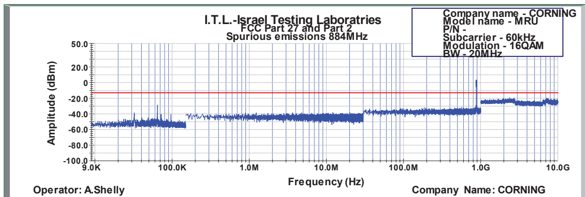
Figure 544: Spurious Emissions at Antenna Terminal 16QAM 20MHz B.W.; 884.0MHz, 60kHz
