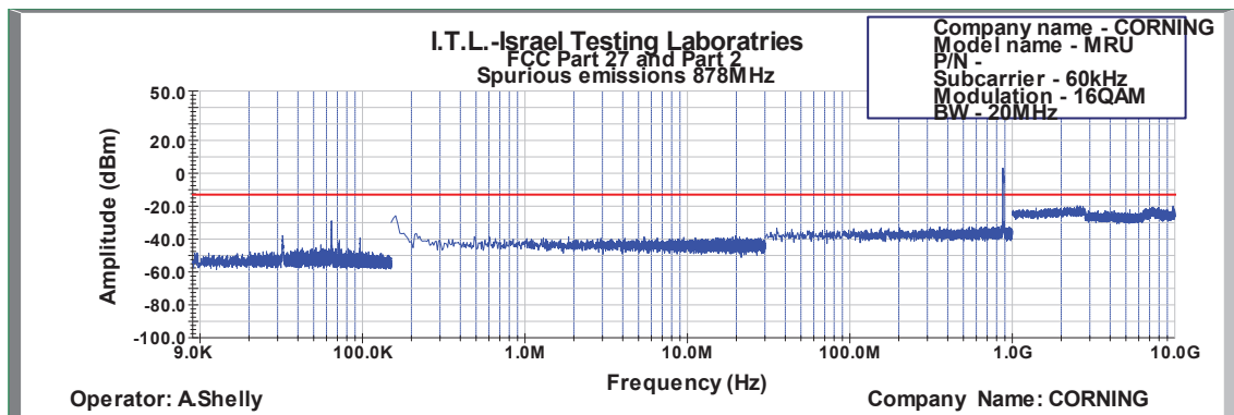
Figure 543: Spurious Emissions at Antenna Terminal 16QAM 20MHz B.W.; 878.0MHz, 60kHz
