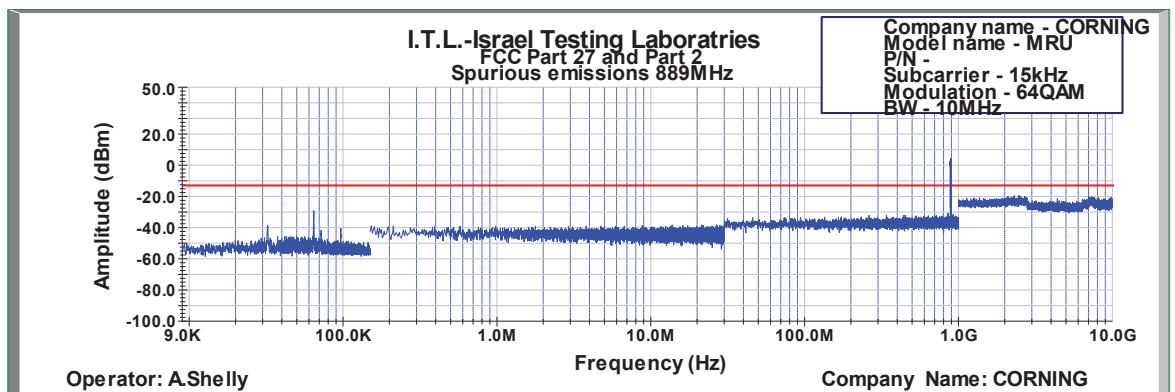
Figure 562: Spurious Emissions at Antenna Terminal 64QAM 10MHz B.W.; 889.0MHz, 15kHz
