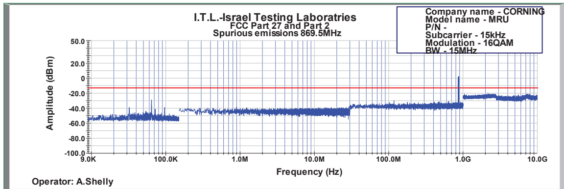
Figure 527: Spurious Emissions at Antenna Terminal 16QAM 15MHz B.W.; 869.5MHz, 15kHz
