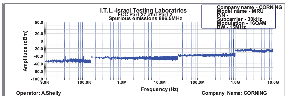
Figure 532: Spurious Emissions at Antenna Terminal 16QAM 15MHz B.W.; 886.5MHz, 30kHz
