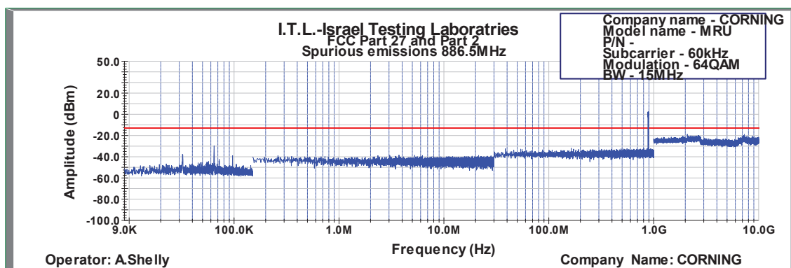
Figure 577: Spurious Emissions at Antenna Terminal 64QAM 15MHz B.W.; 886.5MHz, 60kHz
