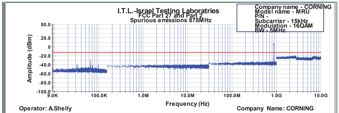
Figure 513: Spurious Emissions at Antenna Terminal 16QAM 5MHz B.W.; 878MHz, 15kHz
