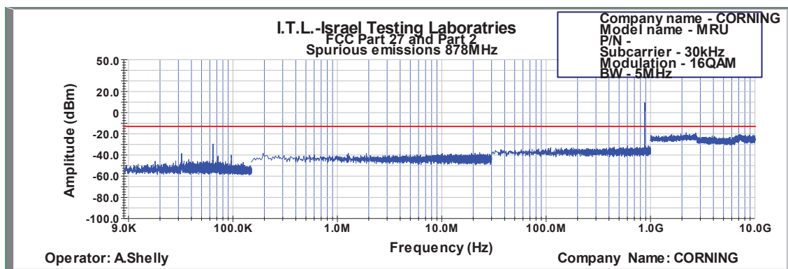
Figure 516: Spurious Emissions at Antenna Terminal 16QAM 5MHz B.W.; 878MHz, 30kHz
