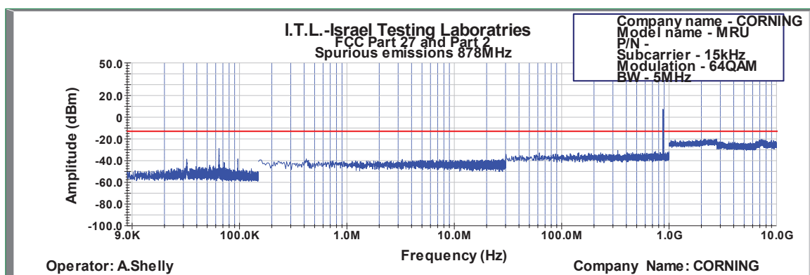
Figure 555: Spurious Emissions at Antenna Terminal 64QAM 5MHz B.W.; 878.0MHz, 15kHz
