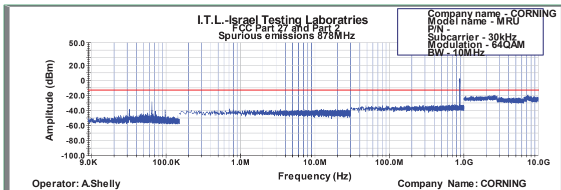
Figure 564: Spurious Emissions at Antenna Terminal 64QAM 10MHz B.W.; 878.0MHz, 30kHz
