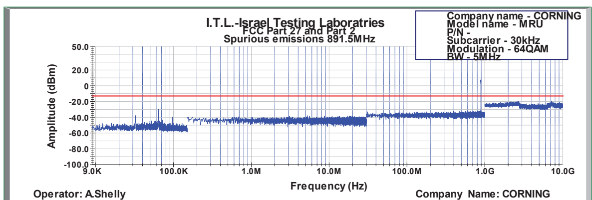
Figure 559: Spurious Emissions at Antenna Terminal 64QAM 5MHz B.W.; 891.5MHz, 30kHz
