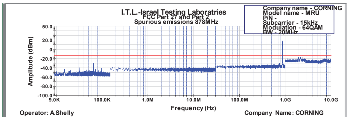
Figure 579: Spurious Emissions at Antenna Terminal 64QAM 20MHz B.W.; 878.0MHz, 15kHz
