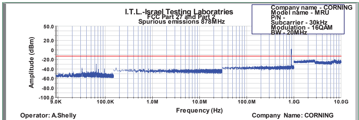
Figure 540: Spurious Emissions at Antenna Terminal 16QAM 20MHz B.W.; 878.0MHz, 30kHz
