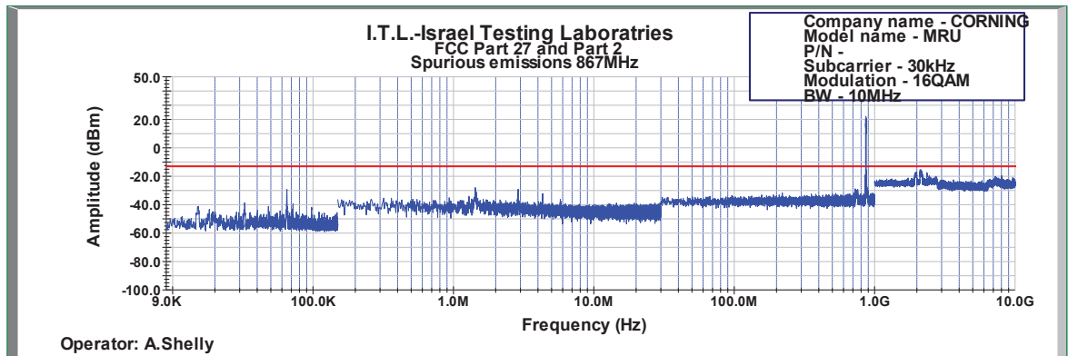
Figure 521: Spurious Emissions at Antenna Terminal 16QAM 10MHz B.W.; 867.0MHz, 30kHz
