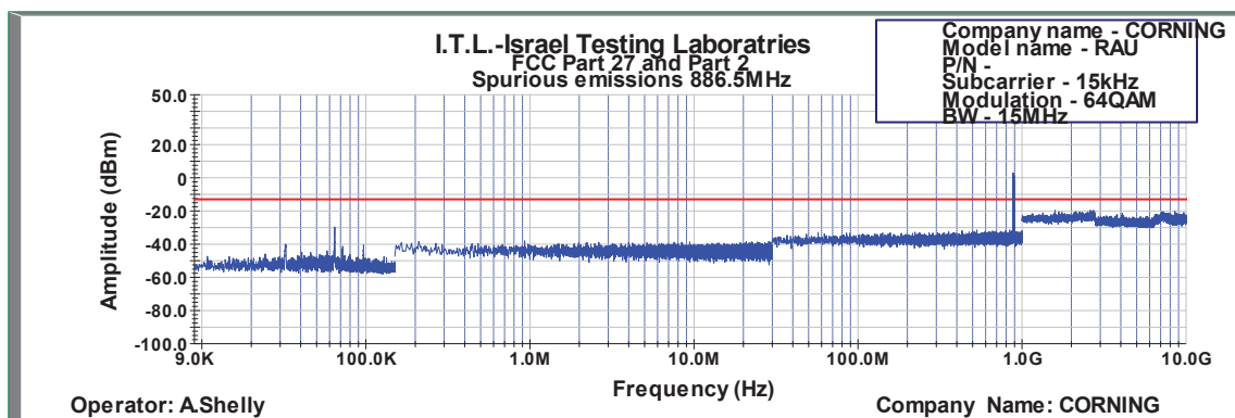
Figure 571: Spurious Emissions at Antenna Terminal 64QAM 15MHz B.W.; 886.5MHz, 15kHz
