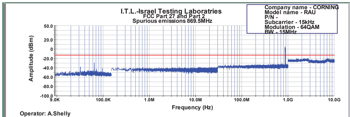
Figure 569: Spurious Emissions at Antenna Terminal 64QAM 15MHz B.W.; 869.5MHz, 15kHz
