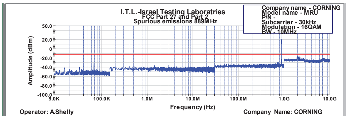
Figure 523: Spurious Emissions at Antenna Terminal 16QAM 10MHz B.W.; 889.0MHz, 30kHz
