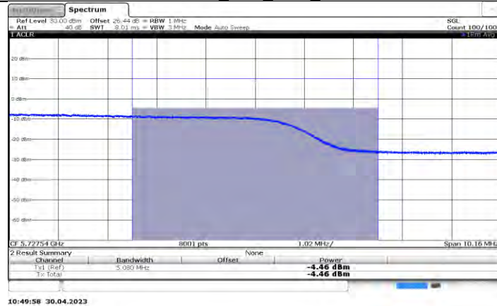
11N40SISO_Ant1_5710_UNII-3
