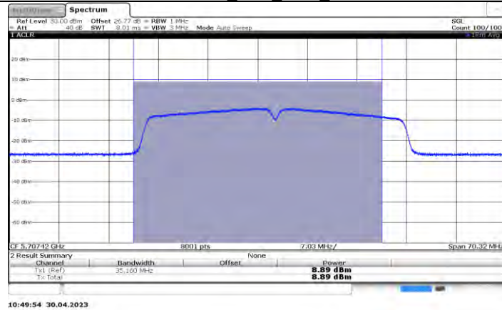
11N40SISO_Ant1_5710_UNII-2C
