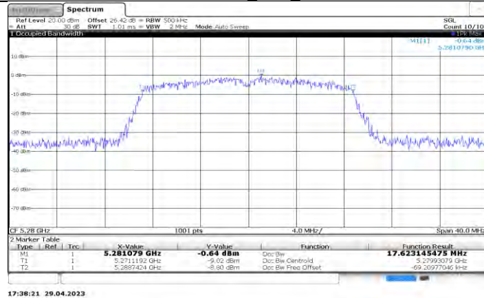
11N20SISO_Ant1_5280
