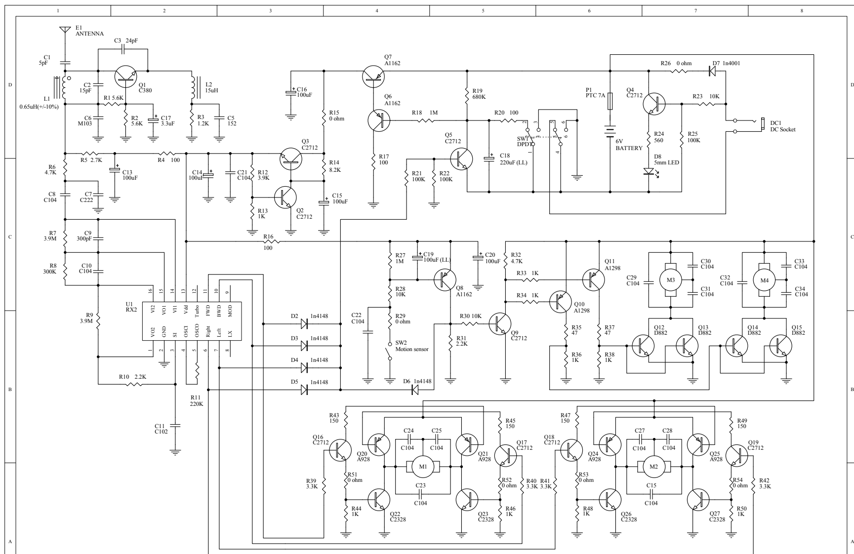
SPIN MASTER #14126 Wall Racer - Receiver (49.860MHz) Circuit Diagram
