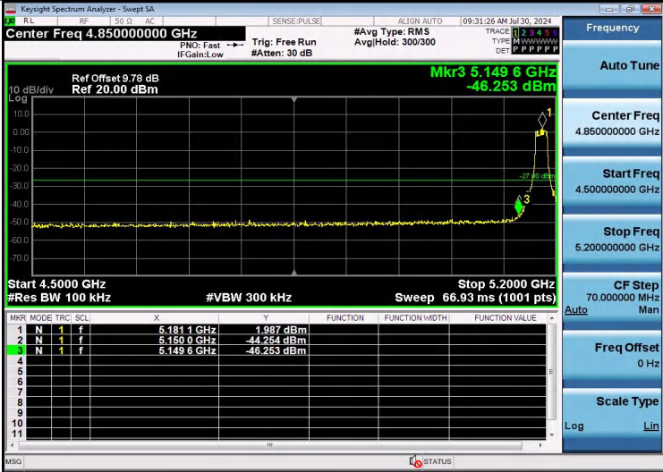
11A-Ant1-5180-PASS
