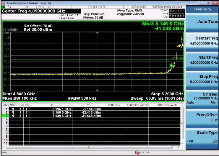
11N40SISO-Ant1-5190-PASS
