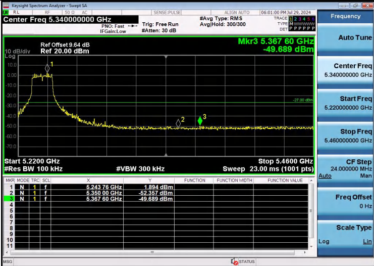
11A-Ant1-5240-PASS
