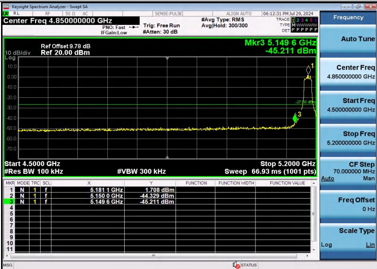
11N20SISO-Ant1-5180-PASS
