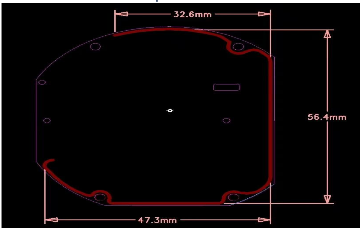
monopole antenna
