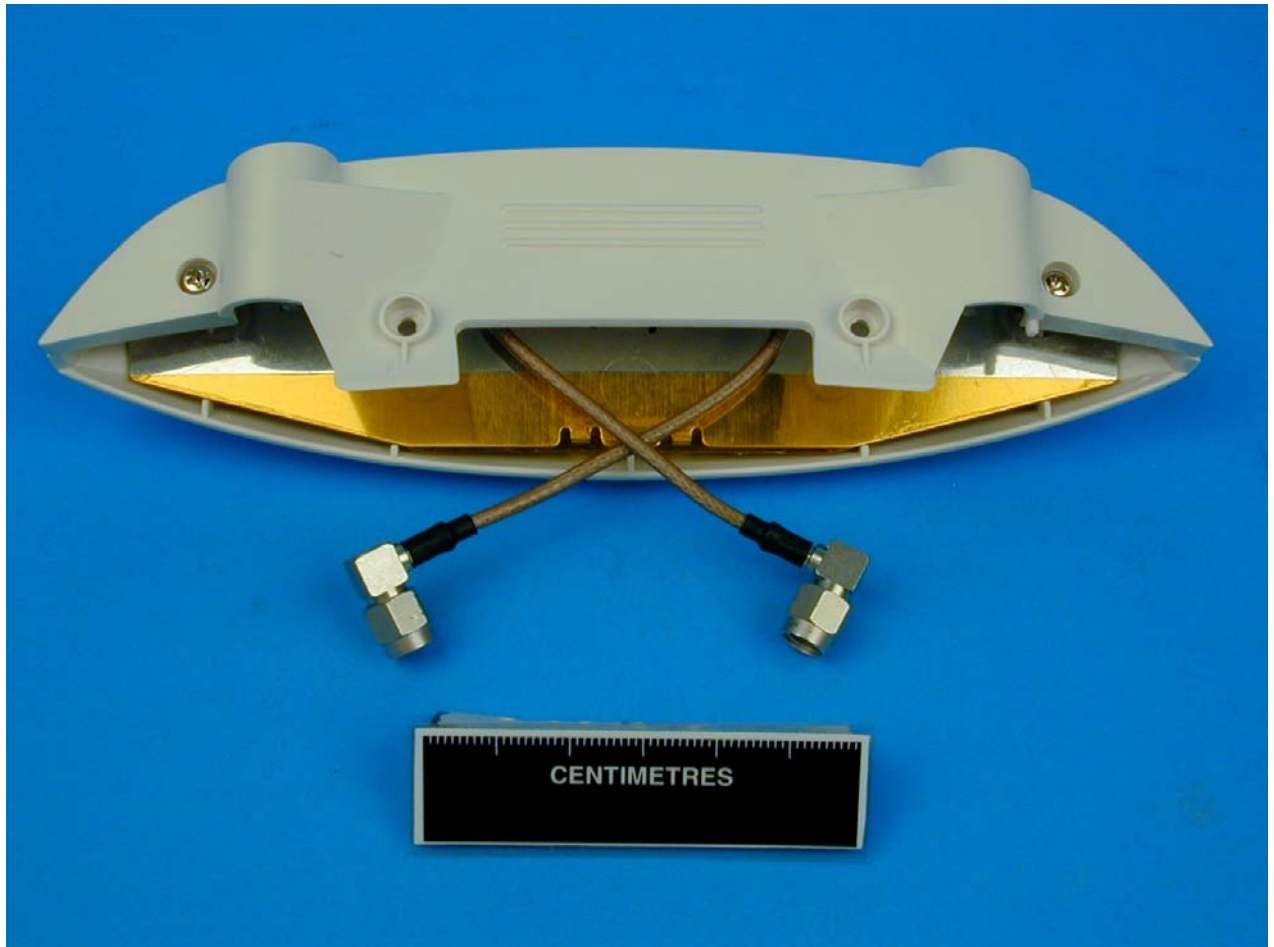
Photograph 9 Internal View Symbol WSAP 5030 Access Port Integral Antenna (5.15-5.25GHz only)
