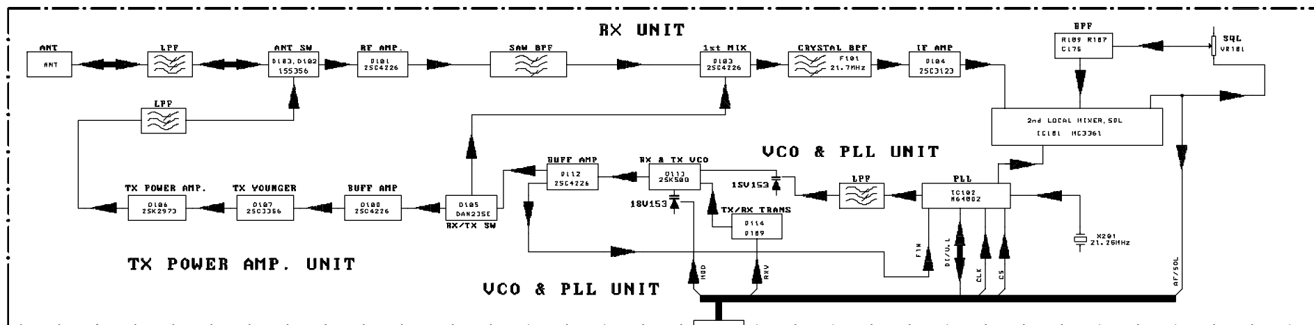
21-1850 BLOCK DIAGRAM ISSUE 3 APR/11/2000
