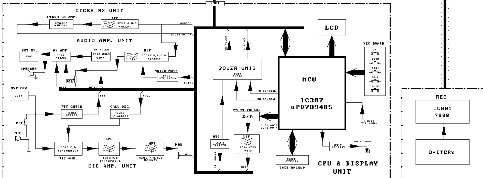
21-1850 BLOCK DIAGRAM ISSUE 3 APR/11/2000
