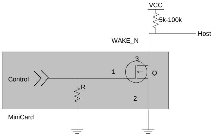
Figure 3-4: Recommended WAKE_N Connection
