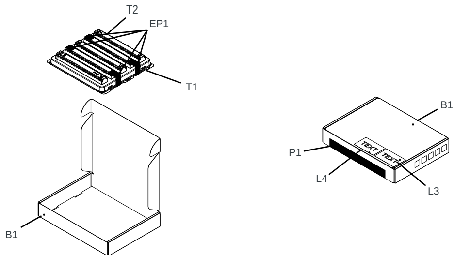
Figure 10-2: Shipping Package
