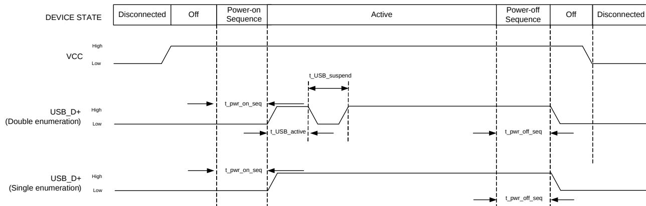
Figure 5-1: Signal Timing (USB Enumeration)
