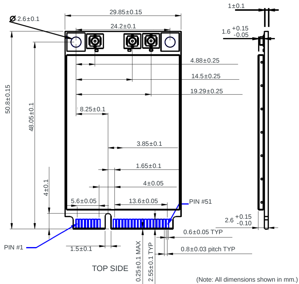
Figure 6-2: Dimensioned View
