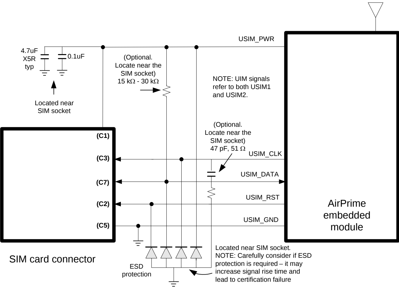
Figure 3-2: SIM Application Interface (applies to both SIM interfaces)
