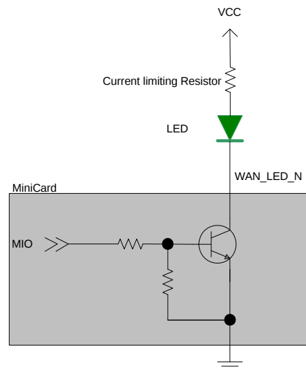
Figure 3-5: Example LED
