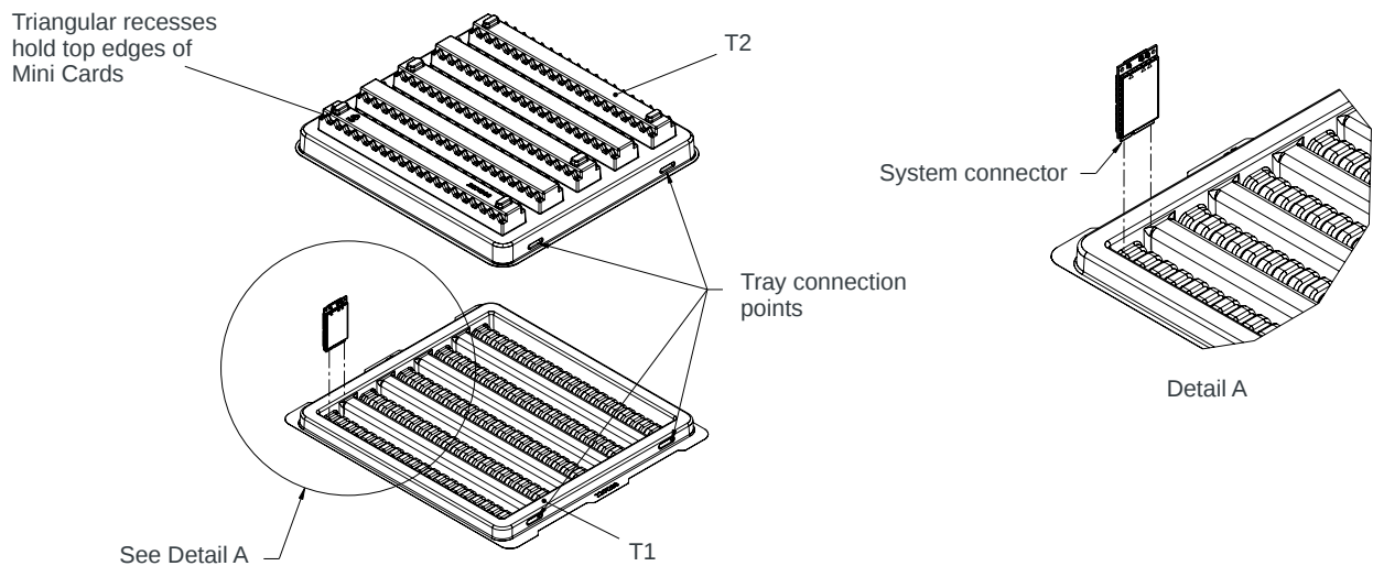
Figure 10-1: Device Placement in Module Tray
