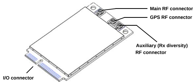
Figure 4-1: Module Connectors
