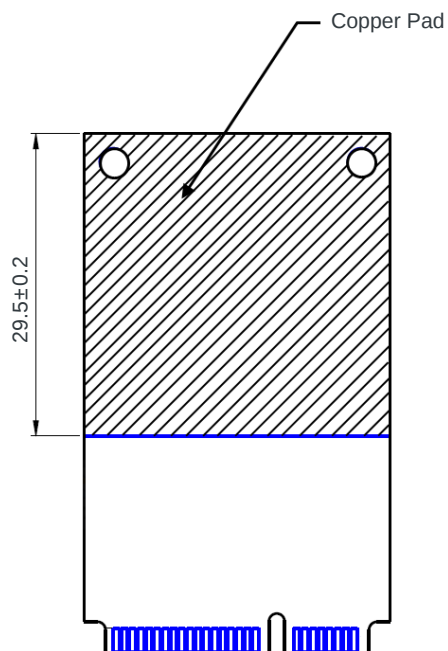
Figure 6-5: Copper Pad Location on Bottom Side of Module
