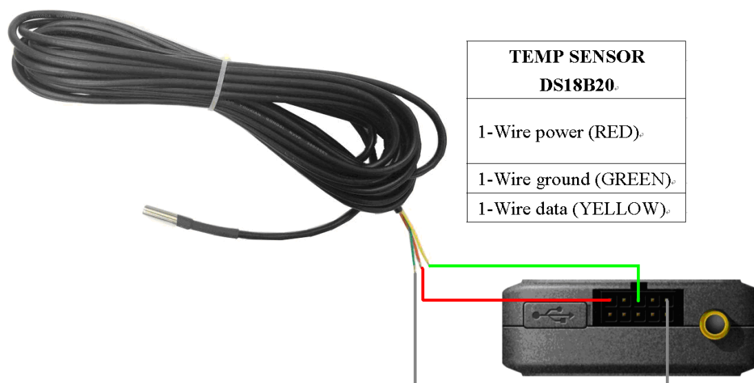
Figure 15. Typical Connection with Temperature Sensor
