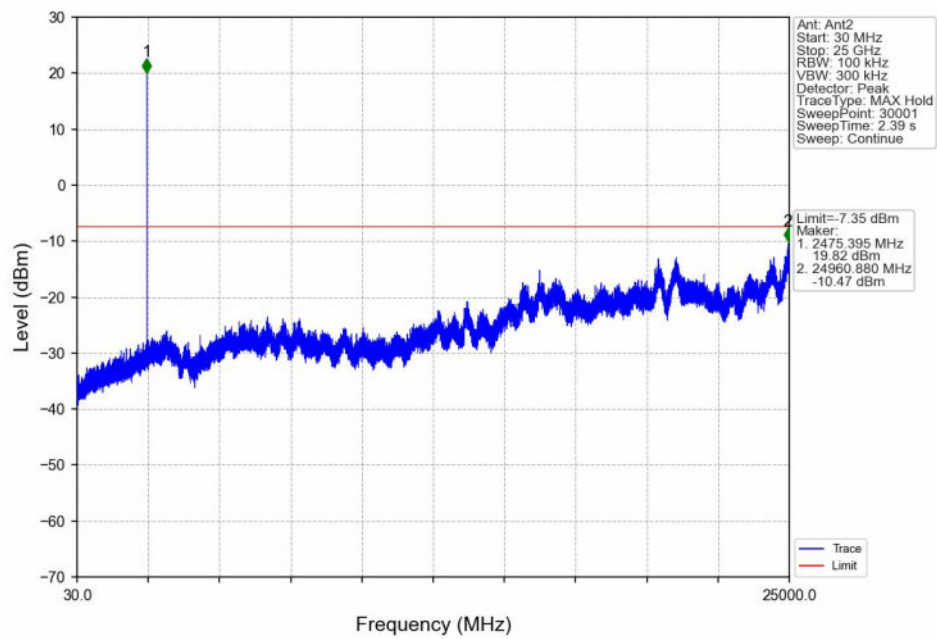
QPSK_HCH_2475.5MHz_Ant2_NTNV
