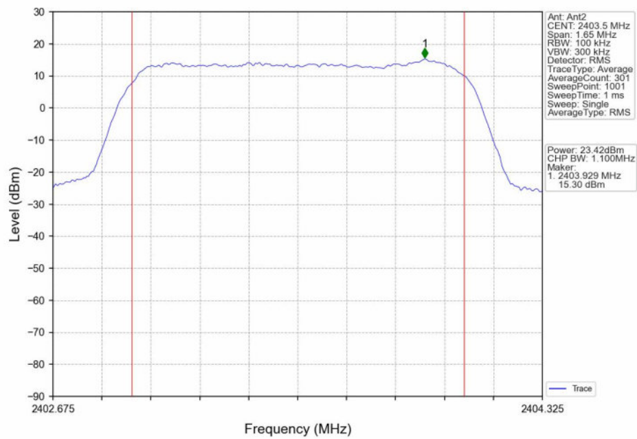
16QAM_LCH_2403.5MHz_Ant2_NTNV
