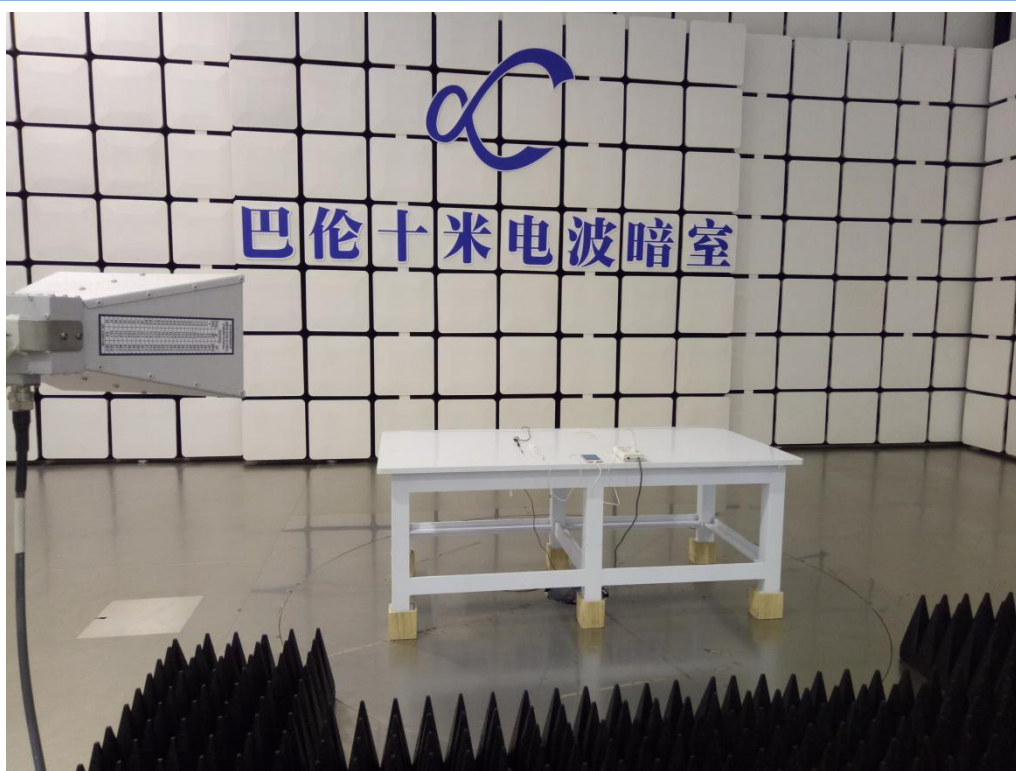
Radiated Test Photo 10
