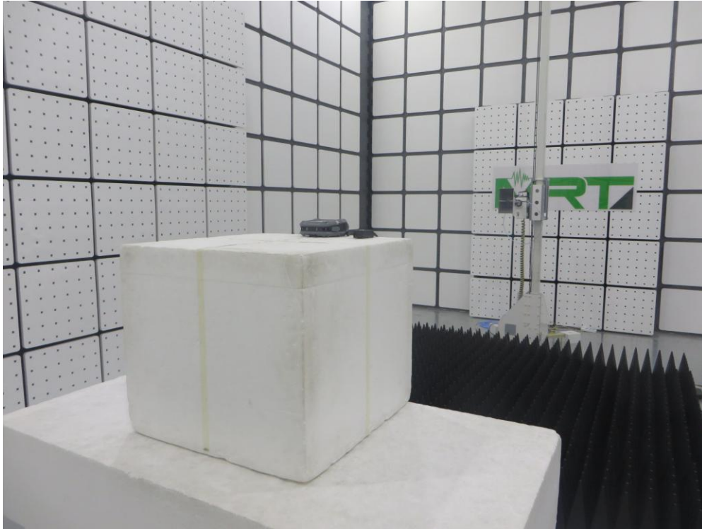
Description: Radiated Emission Test Setup for 1GHz ~ 18GHz (Host Model: RP4D)
