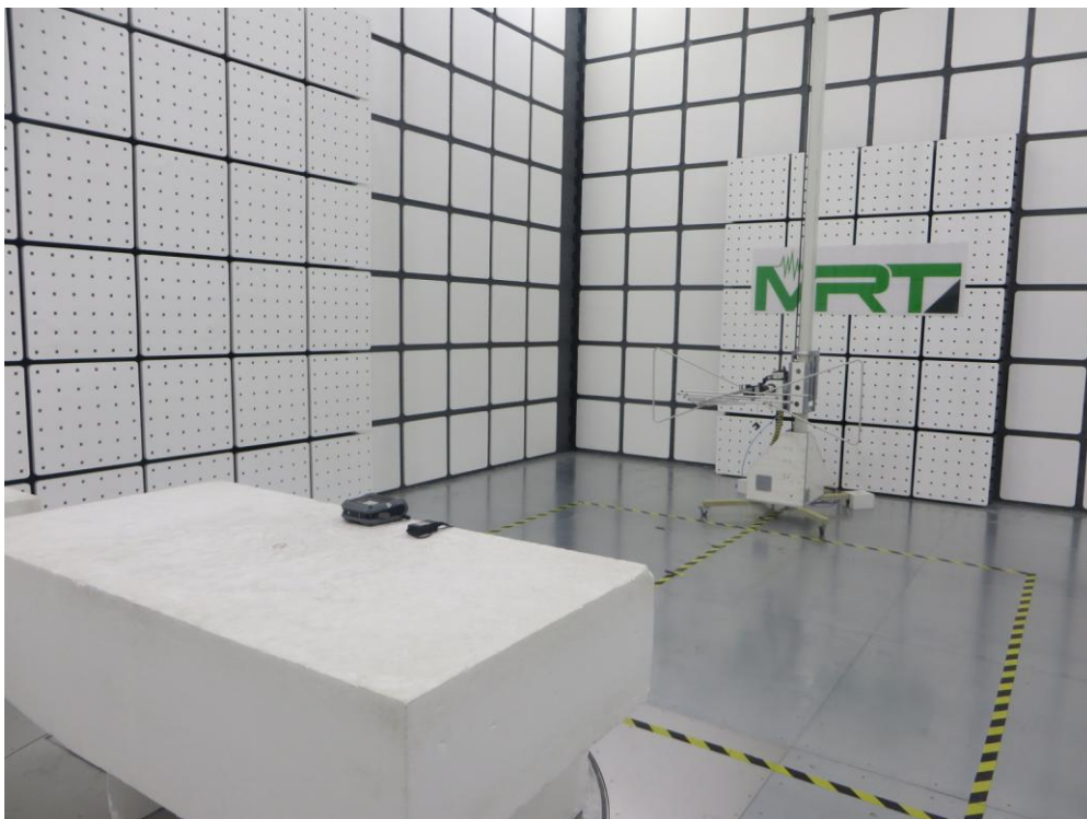
Description: Radiated Emission Test Setup for 30MHz ~ 1GHz (Host Model: RP4D)
