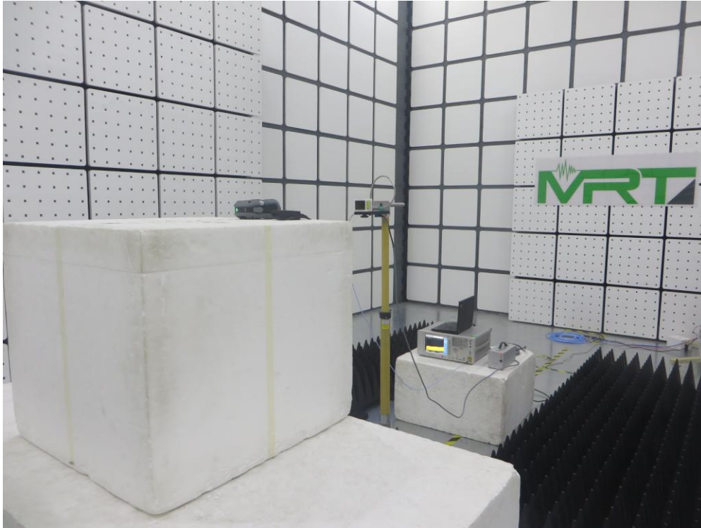
Description: Radiated Emission Test Setup for 18GHz ~ 40GHz (Host Model: RP2D)
