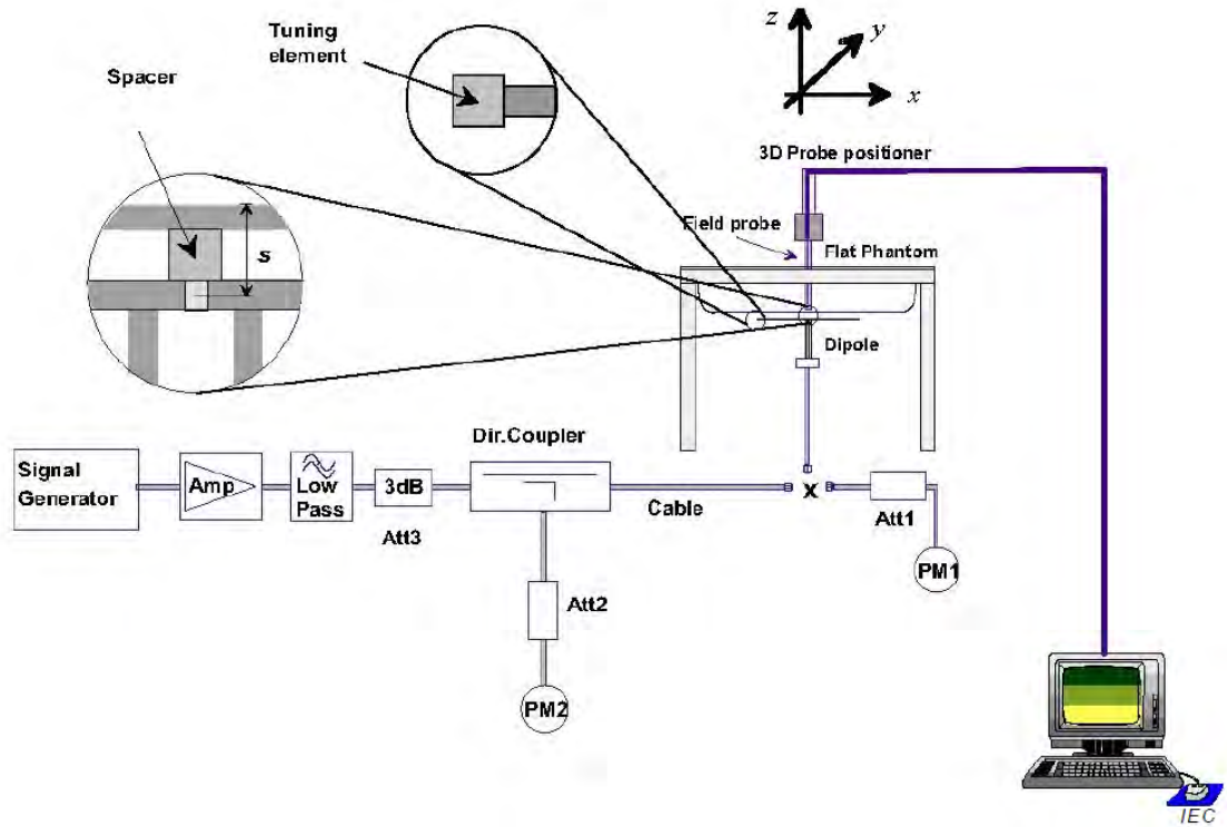
Figure 4 System Check Set-up
