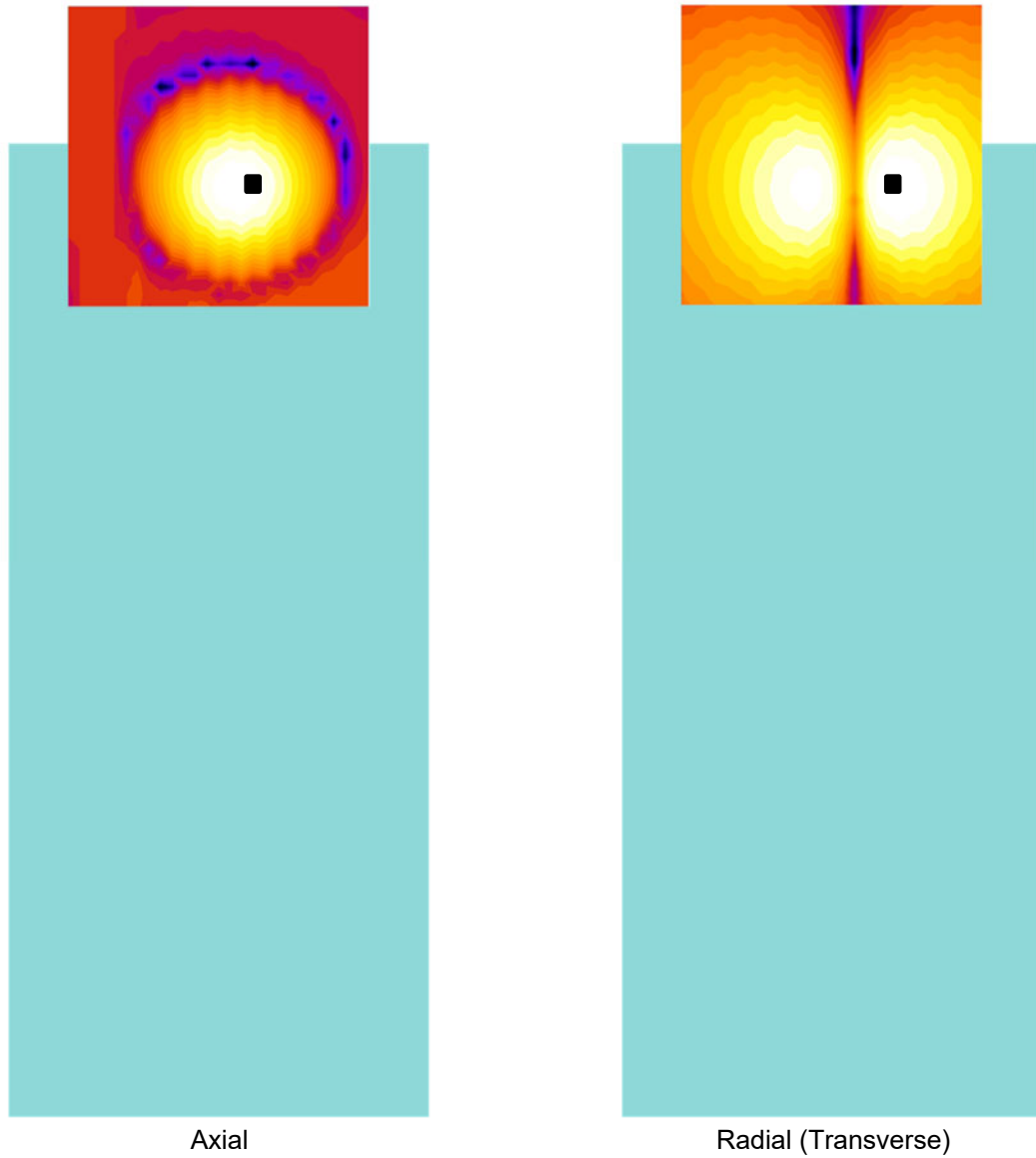
Figure 8-1 T-Coil Scan Overlay Magnetic Field Distributions
