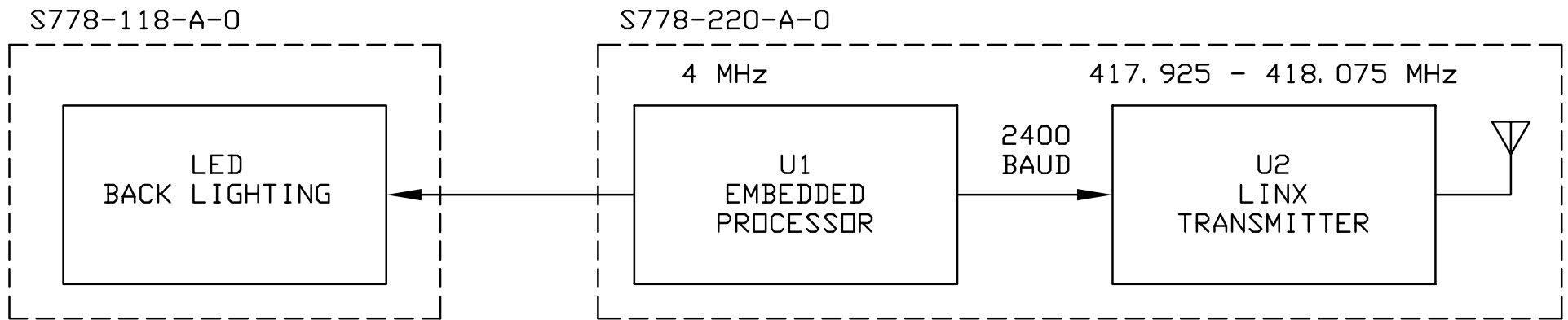
CORDLESS HAND REMOTE BLOCK DIAGRAM
