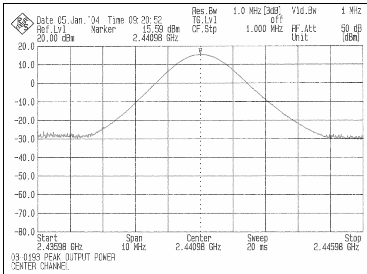
Figure 6.4-1: Output power
