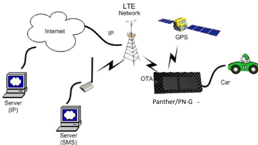
Figure 1 This product is based on the Mediatek 2503x. Antennas for cellular and GPS are internal to the device.
