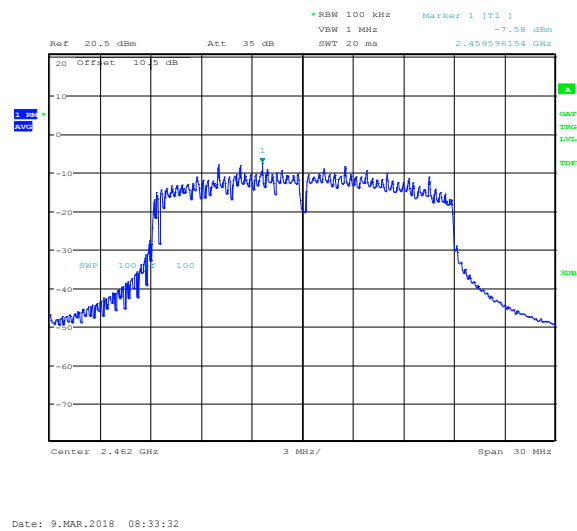
Figure 8.8-9: PSD measurement on 802.11n HT20, high channel
