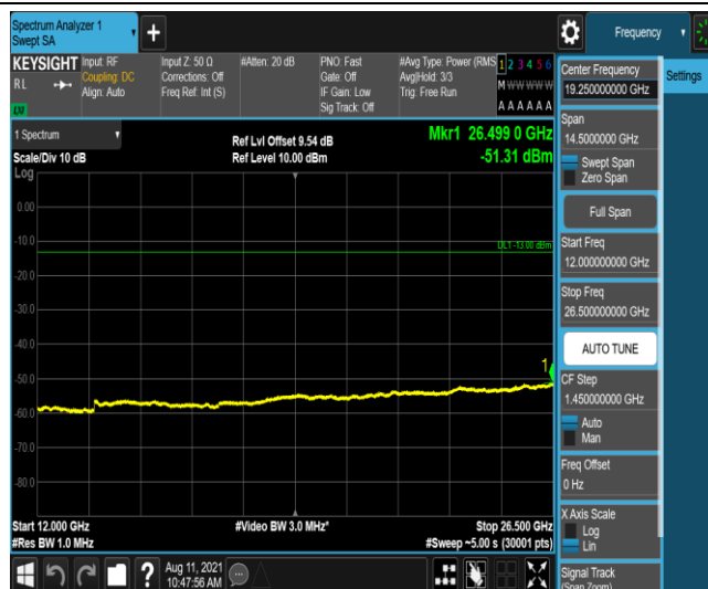
Band25-15MHz-16QAM-26615-1-0-High-12000-26500--51.31-PASS
