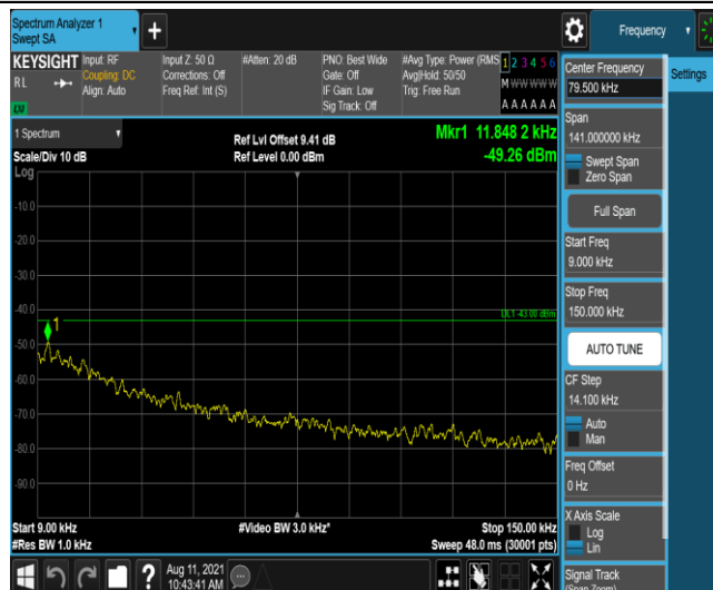
Band25-15MHz-16QAM-26365-1-0-Low-0.009-0.15--49.26-PASS
