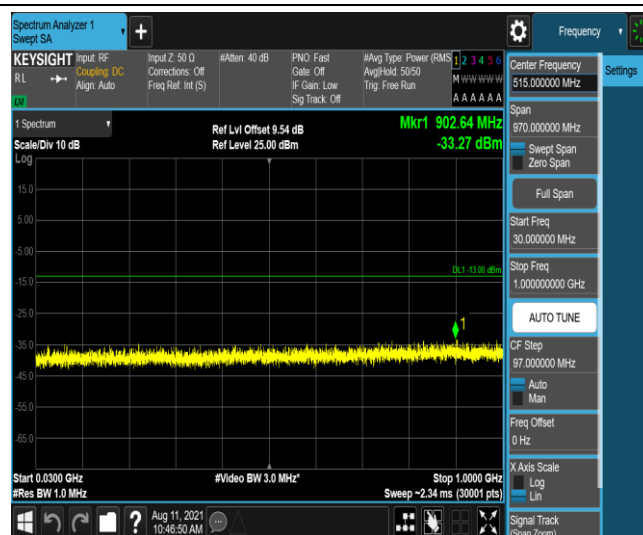
Band25-15MHz-16QAM-26615-1-0-High-30-1000--33.27-PASS
