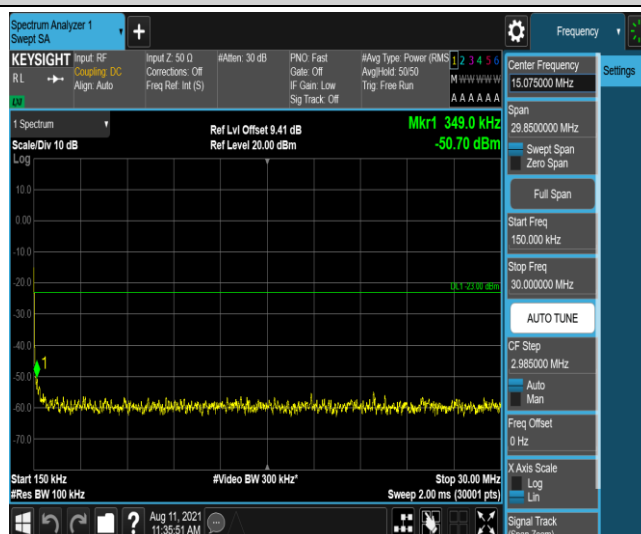
Band25-20MHz-QPSK-26140-1-0-Low-0.15-30--50.7-PASS
