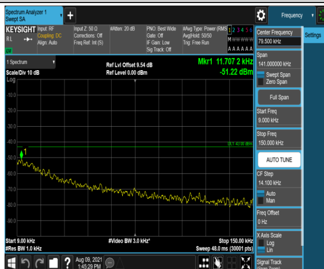
Band25-10MHz-16QAM-26640-1-0-High-0.009-0.15--51.22-PASS
