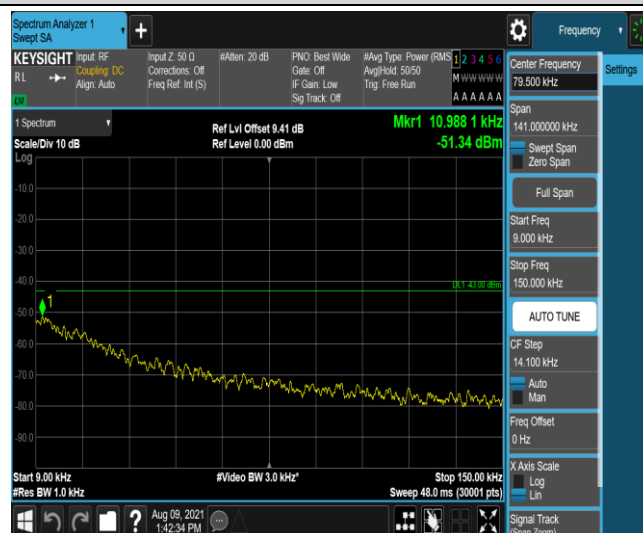
Band25-10MHz-16QAM-26365-1-0-Low-0.009-0.15--51.34-PASS
