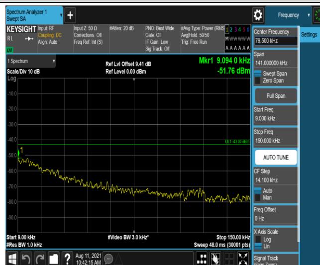
Band25-15MHz-QPSK-26365-1-0-Low-0.009-0.15--51.76-PASS
