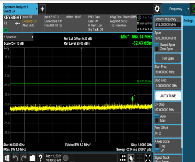
Band25-15MHz-16QAM-26115-1-0-Low-30-1000--32.43-PASS
