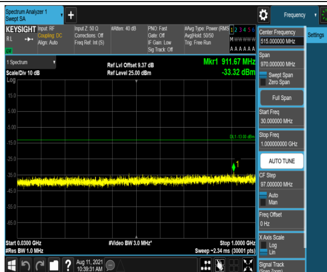
Band25-15MHz-QPSK-26115-1-0-Low-30-1000--33.32-PASS
