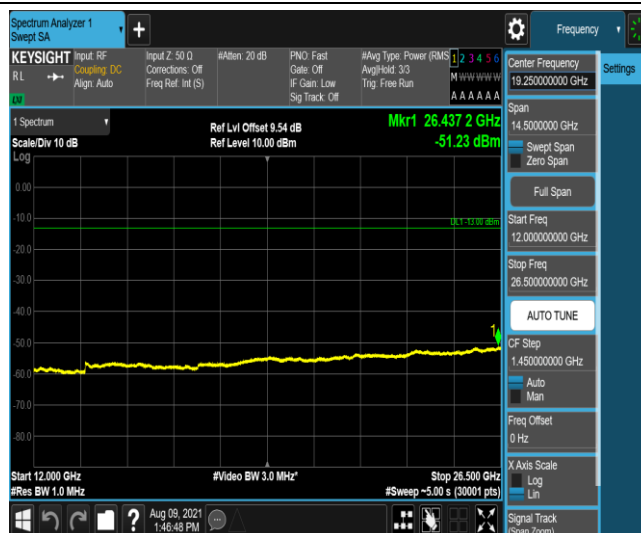
Band25-10MHz-16QAM-26640-1-0-High-12000-26500--51.23-PASS
