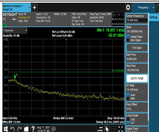
Band25-15MHz-16QAM-26615-1-0-High-0.009-0.15--52.07-PASS
