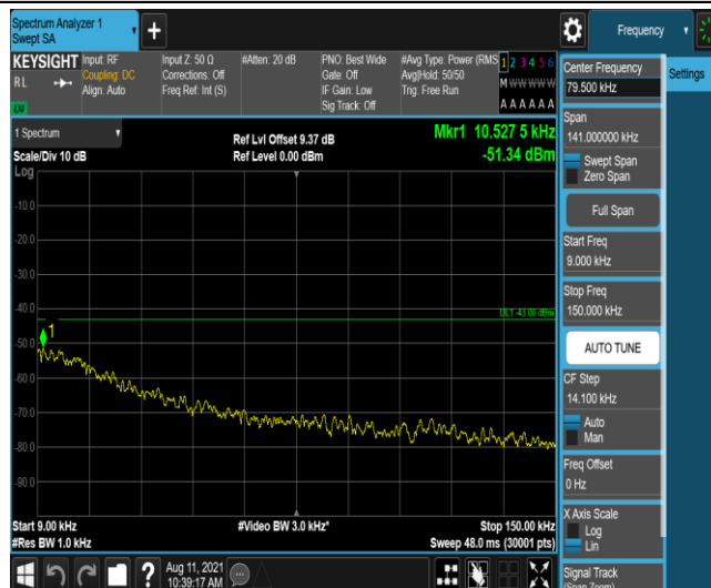
Band25-15MHz-QPSK-26115-1-0-Low-0.009-0.15--51.34-PASS
