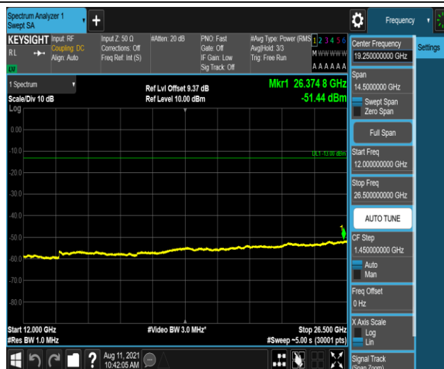
Band25-15MHz-16QAM-26115-1-0-Low-12000-26500--51.44-PASS
