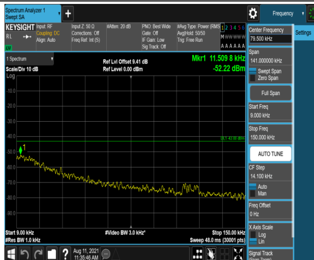
Band25-20MHz-QPSK-26140-1-0-Low-0.009-0.15--52.22-PASS
