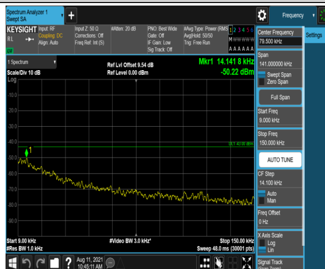
Band25-15MHz-QPSK-26615-1-0-High-0.009-0.15--50.22-PASS
