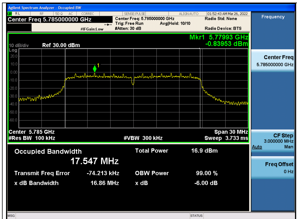
Test Graph 802.11n20 ANT1 5785 MCS0 DTBW
