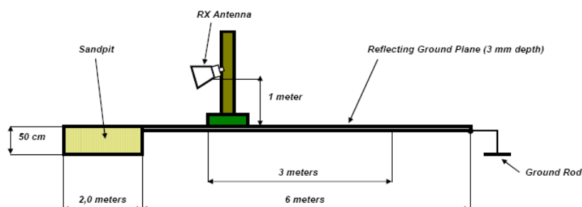
Radiated measurement above 960 MHz
