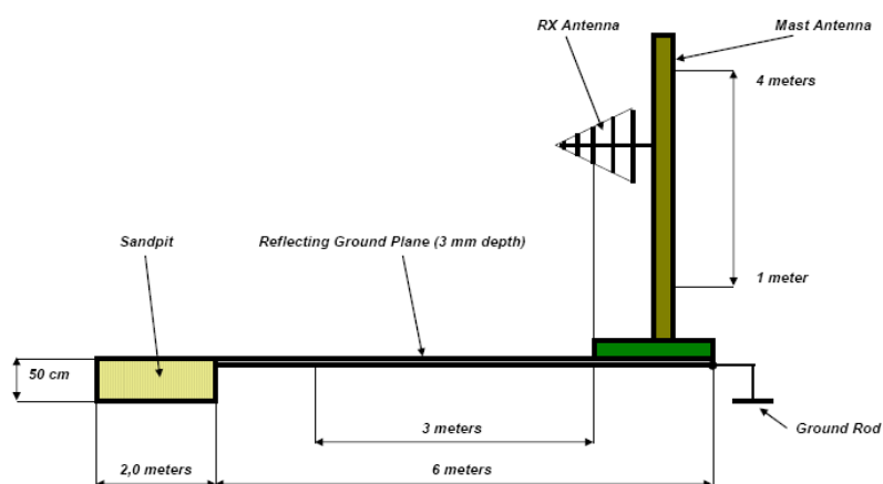
Radiated measurement below 960 MHz
