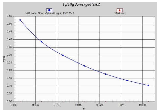
Fig. 1-25 Z-Scan at power reference point (LTEB17)
