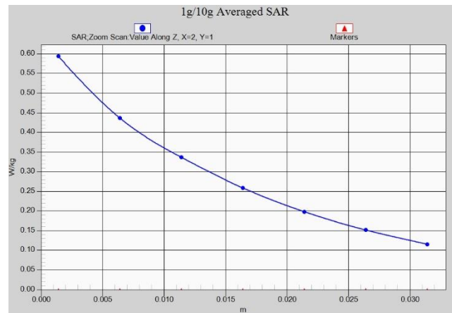
Fig. 1-24 Z-Scan at power reference point (LTEB17)
