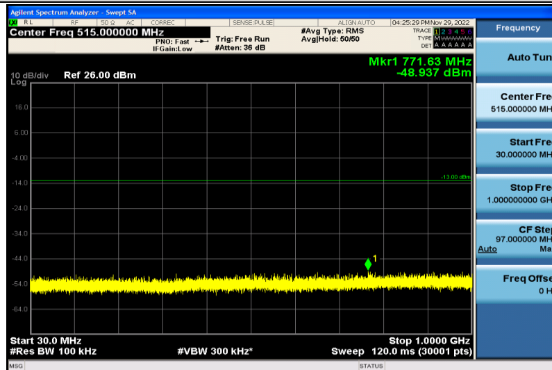
Band66-15MHz-16QAM-132597-1RB#0-30~1000MHz
