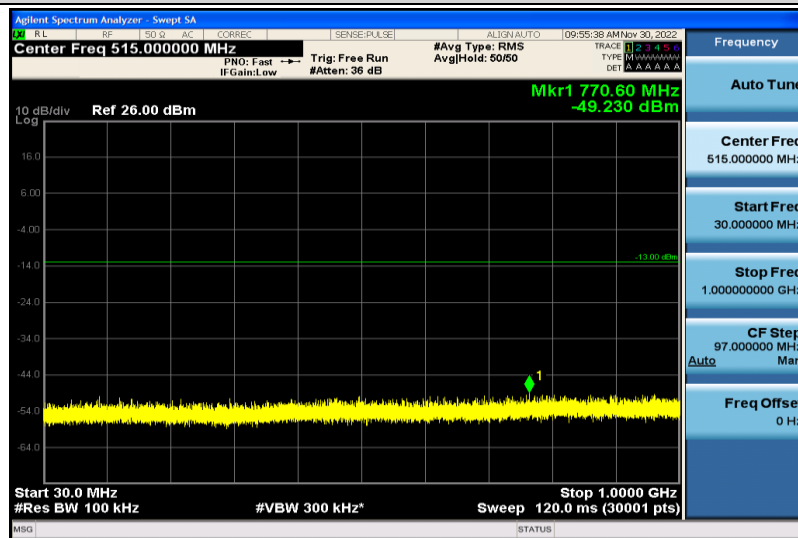
Band66-20MHz-64QAM-132072-1RB#0-30~1000MHz
