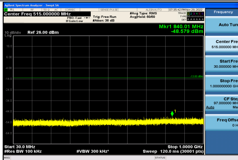
Band66-10MHz-64QAM-132622-1RB#0-30~1000MHz
