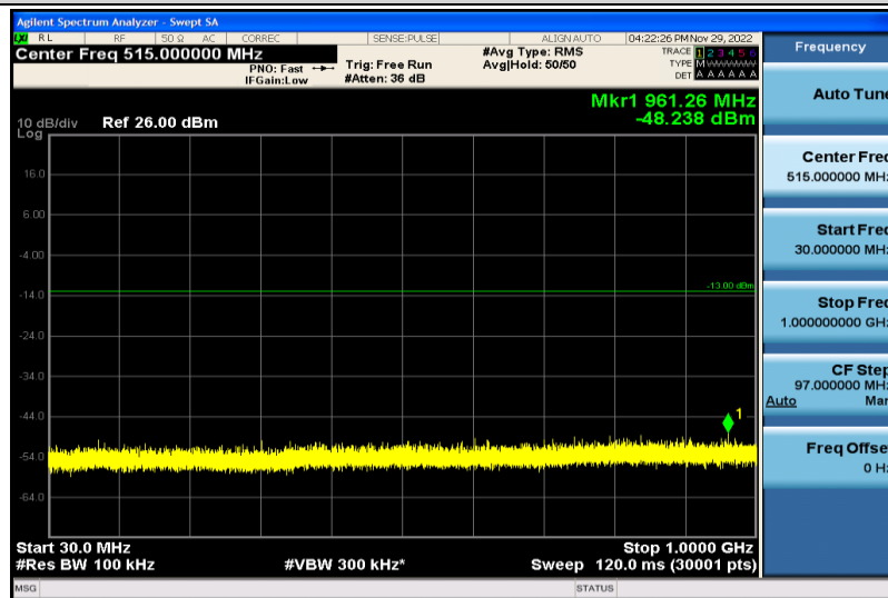
Band66-15MHz-QPSK-132047-1RB#0-30~1000MHz
