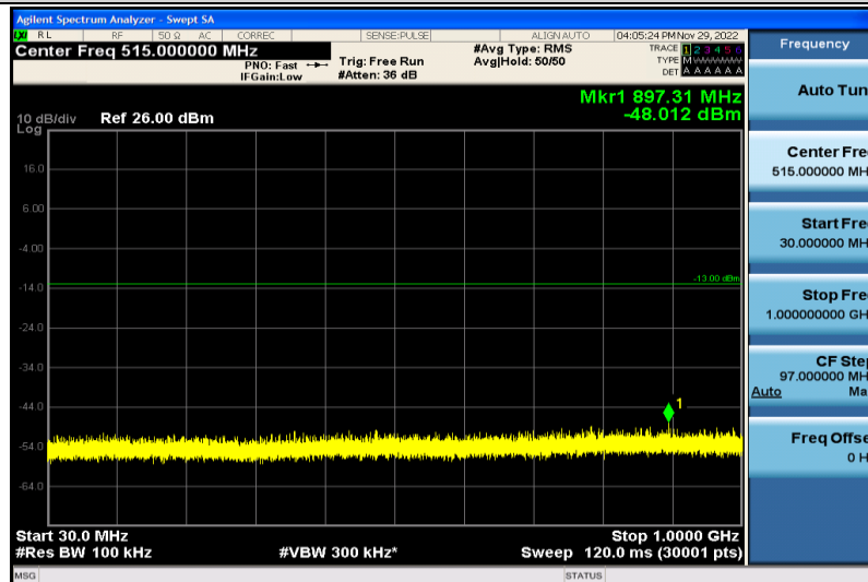
Band66-10MHz-16QAM-132622-1RB#0-30~1000MHz
