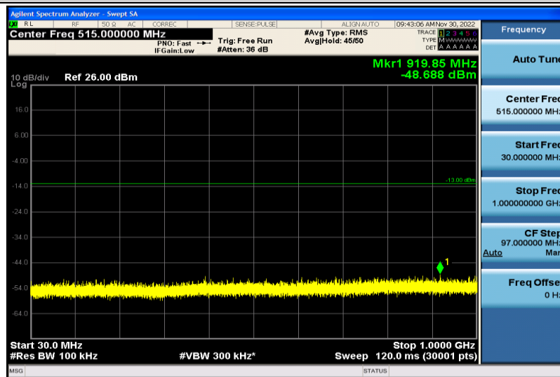
Band66-15MHz-64QAM-132047-1RB#0-30~1000MHz
