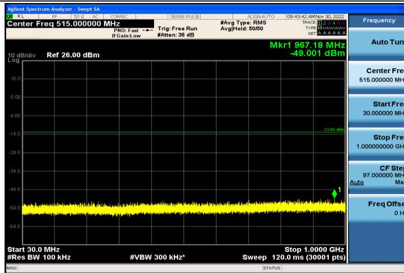
Band66-15MHz-64QAM-132322-1RB#0-30~1000MHz
