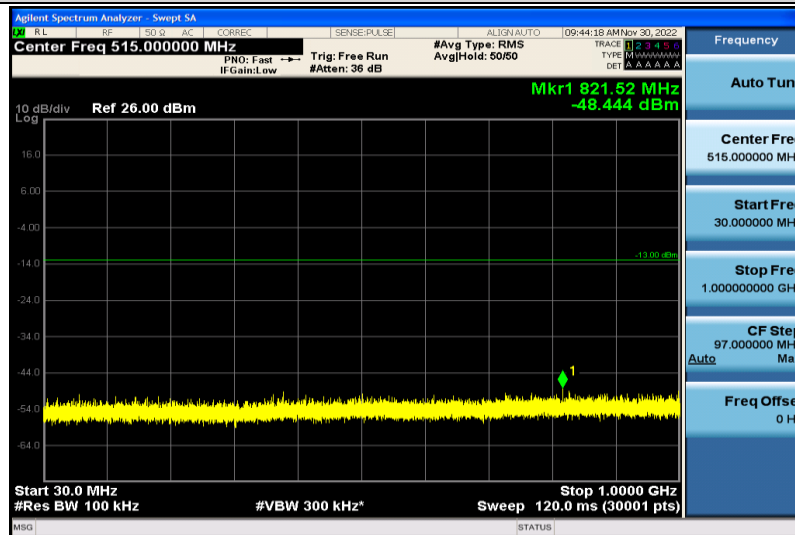
Band66-15MHz-64QAM-132597-1RB#0-30~1000MHz
