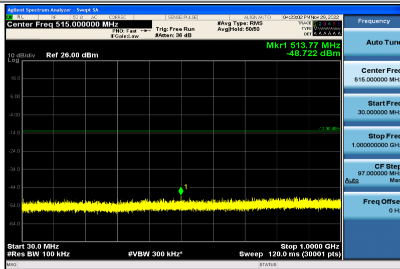
Band66-15MHz-16QAM-132047-1RB#0-30~1000MHz
