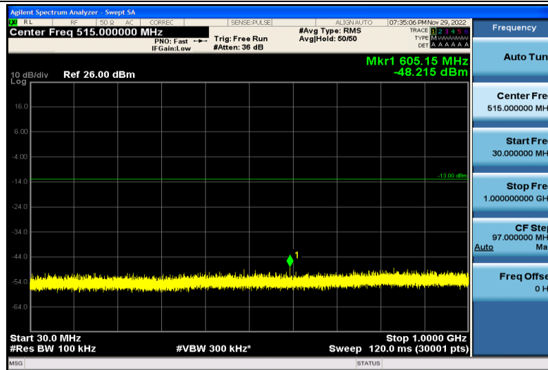
Band66-10MHz-64QAM-132322-1RB#0-30~1000MHz
