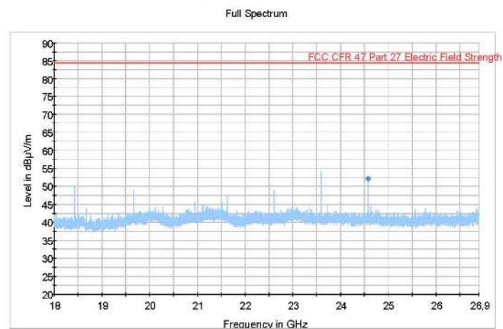
Figure 297 Radiated Emission 18 GHz – 26.9 GHz (2652.5MHz/2657.5MHz) (5MHz+5MHz Channel BW)
