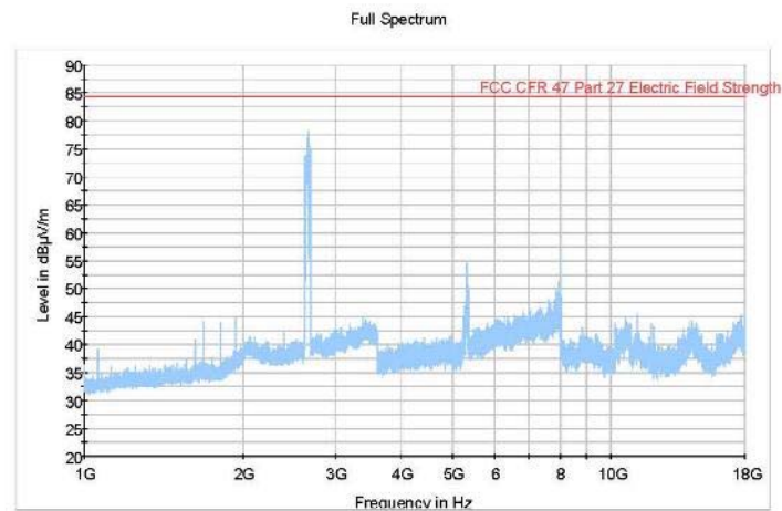
Figure 312 Radiated Emission 1 GHz – 18 GHz (2647.5MHz/2622.5MHz) (15MHz+15MHz Channel BW)
