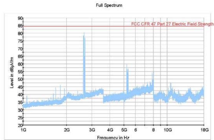
Figure 294 Radiated Emission 1 GHz – 18 GHz (2652.5/2657.5MHz) (5+5 MHz Channel BW)
