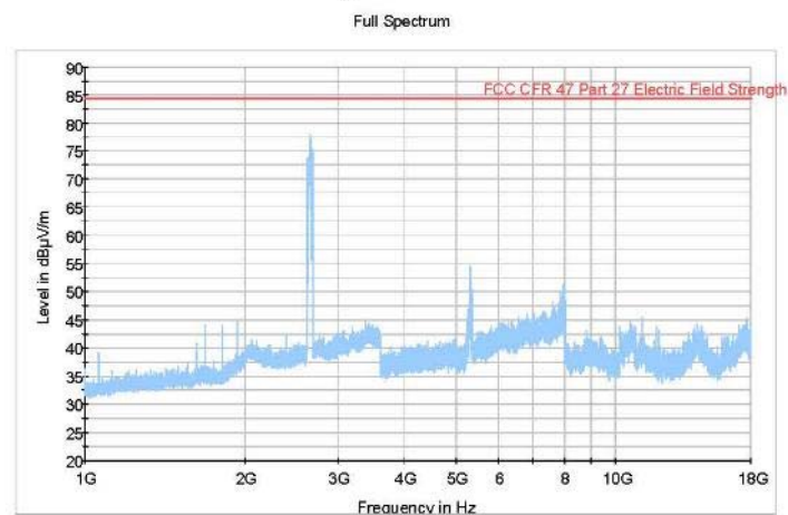
Figure 311 Radiated Emission 1 GHz – 18 GHz (2627.5MHz/2645.5MHz) (15MHz+15MHz Channel BW)
