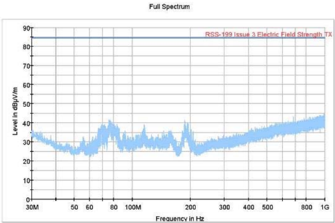
Figure 345 Radiated Emission 30 MHz – 1 GHz (2655MHz) (15MHz Channel BW)
