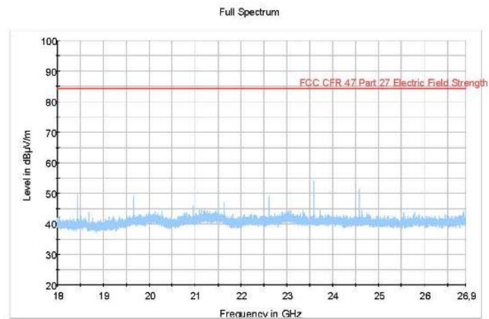
Figure 296 Radiated Emission 18 GHz – 26.9 GHz (2622.5MHz/2627.5MHz) (5MHz+5MHz Channel BW)
