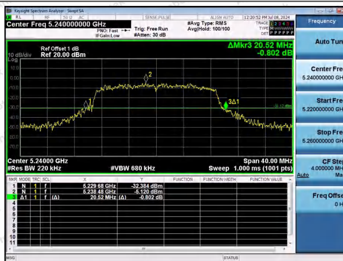
11AC20SISO-Ant1-5240
