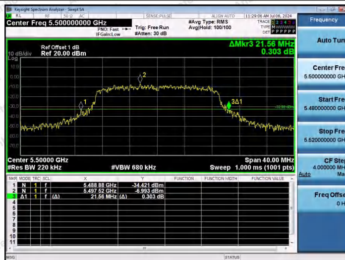
11N20SISO-Ant1-5500
