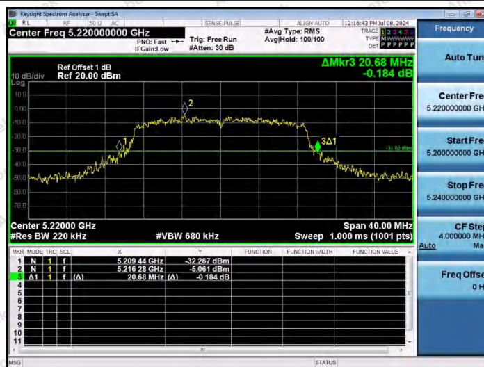
11AC20SISO-Ant1-5220
