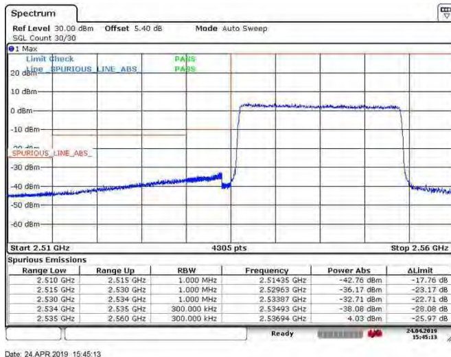
Band41_20MHz_64QAM_41140_1RB#99
