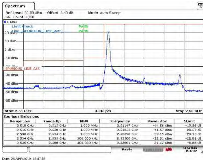
Band41_20MHz_64QAM_40140_100RB#0
