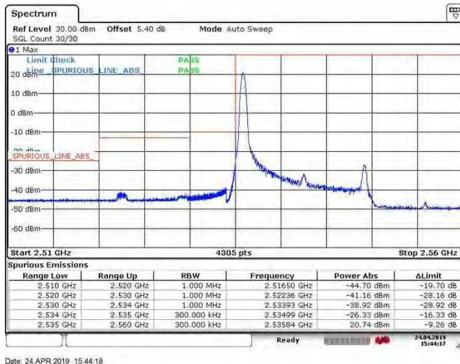
Band41_15MHz_64QAM_40115_75RB#0
